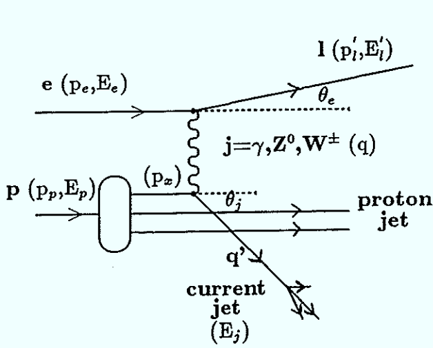
Fig. 2.15 Diagram of the deep inelastic electron-proton scattering process.
