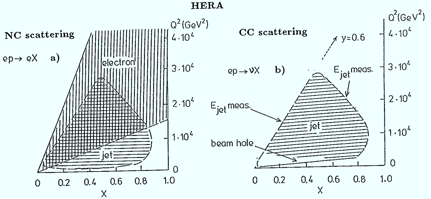
Fig. 2.20 The accessible regions at HERA where x and Q^2 can be well measured: a) for NC scattering from either the electron or the jets and b) for CC scattering only from the jets.
