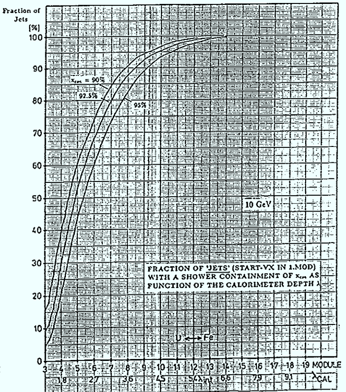
Fig. 4.30b Fraction of 'jets' with a shower containment of x_{cen} as function of the calorimeter depth \lambda_{CAL} for 10 GeV.
