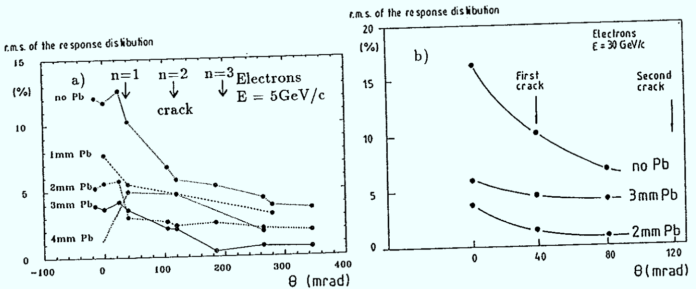
Fig. 5.25 R.m.s. of the response distribution for the same conditions as for Fig. 5.24. These values indicate the direct contribution to the electron energy resolution.
