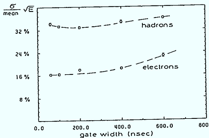
Figure 4.60 Energy resolution for hadrons and electrons vs. integration time in TEST 35.
