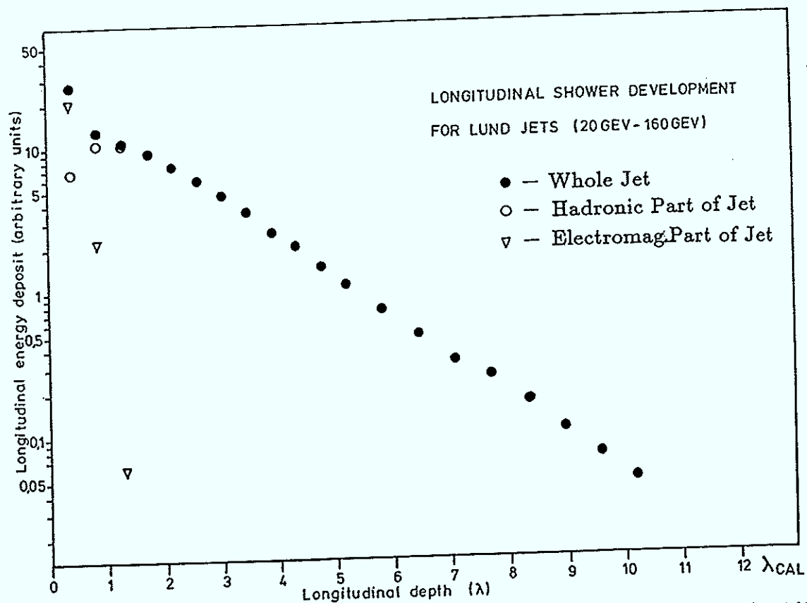
Fig. 4.26 Longitudinal shower profiles of LUND jets ( x > 0.1 , y > 0.6 ; 20 GeV - 160 GeV jets) plus electromagnetic and hadronic parts as function of the calorimeter depth \lambda_{CAL} using the shower development measured for single particles.
