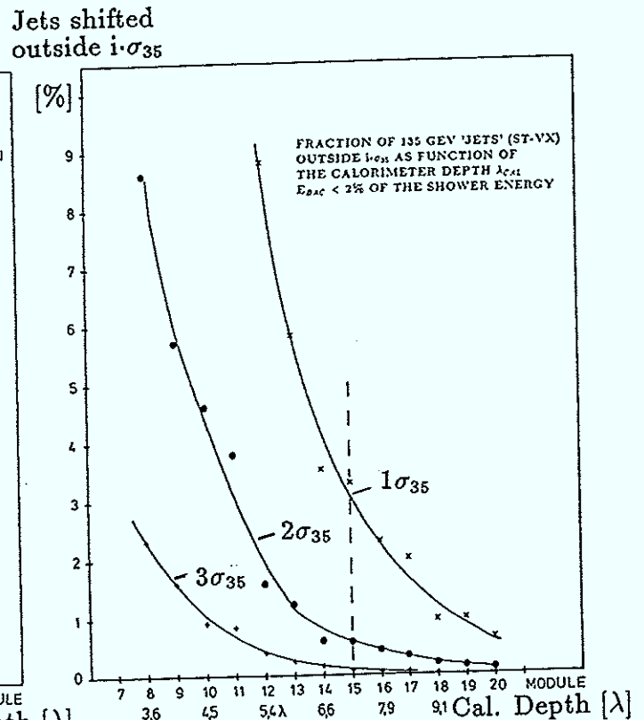
Fig. 4.44 Fraction of 135 GeV 'Jets' additionally outside 1\sigma_{35} as Function of the Calorimeter Depth for E_{BAC} < 2\% of the Shower Energy.
