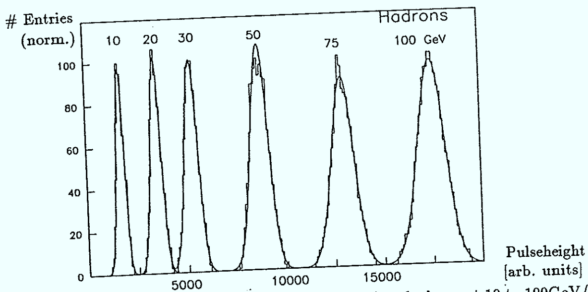
Fig. 4.72b Response of the TEST 60 calorimeter (T60B2) to hadrons at 10 to 100GeV/c.
