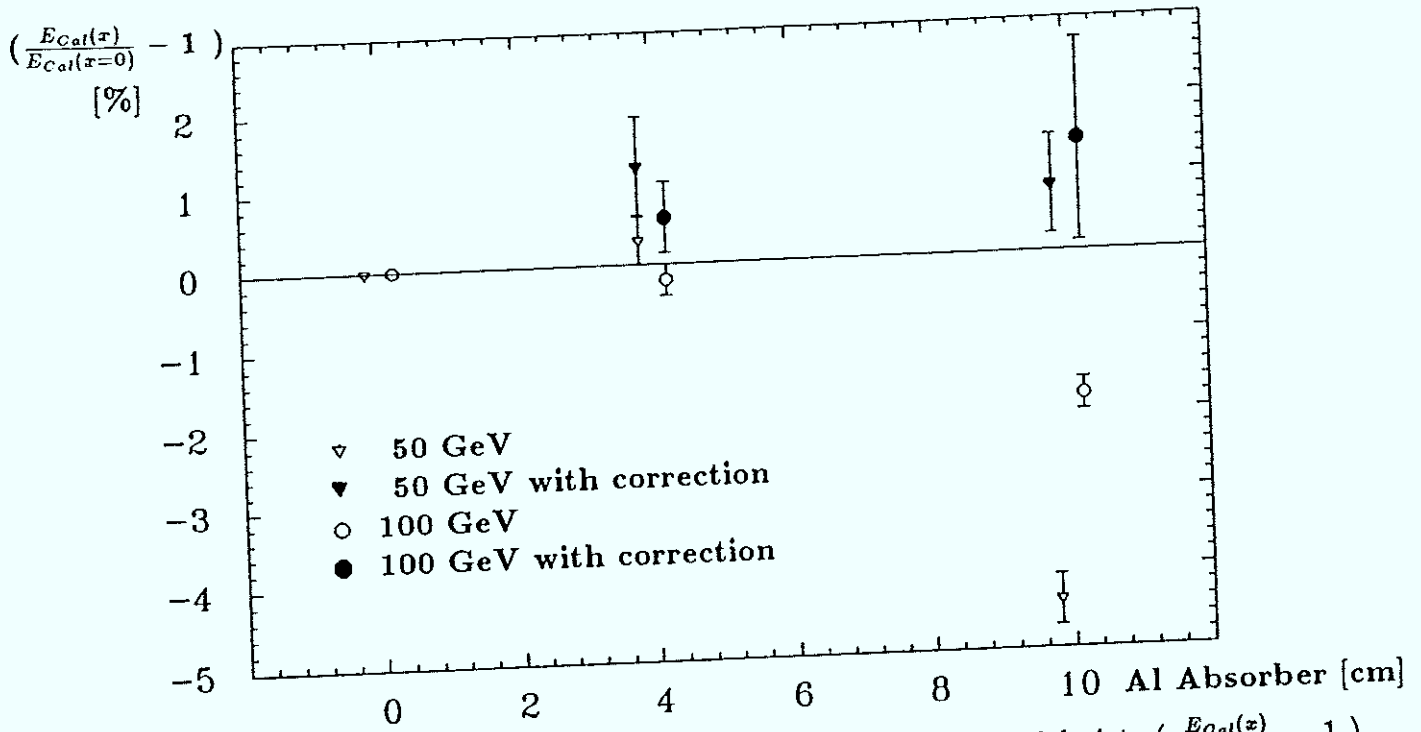
Fig. 5.38 Influence of an Al abs. on the average response to particle jets (\frac{E_{Cal}(x)}{E_{Cal}(x=0)} - 1) as a function of the Al absorber thickness x [cm] for 50GeV and 100GeV jets without and with correction by the multiplicity measured with the trigger system and the presampler.
