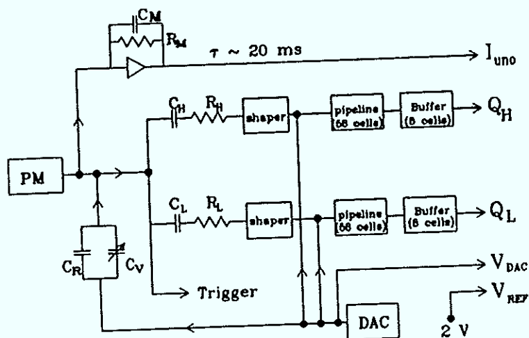
Figure 6.15 Schematics of a front-end card.
