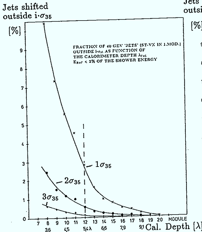
Fig. 4.43 Fraction of 40 GeV 'Jets' additionally outside 1\sigma_{35} as Function of the Calorimeter Depth for E_{BAC} < 2\% of the Shower Energy.
