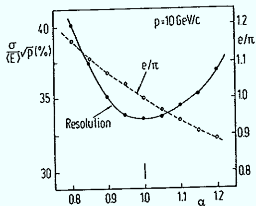
Figure 5.15 Energy resolution and e/h -ratio for 10 GeV/c pions as a function of the intercalibration parameter \alpha .
