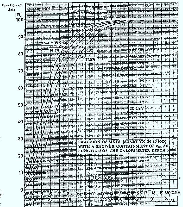
Fig. 4.31b Fraction of 'jets' with a shower containment of x_{cen} as function of the calorimeter depth \lambda_{CAL} for 20 GeV.
