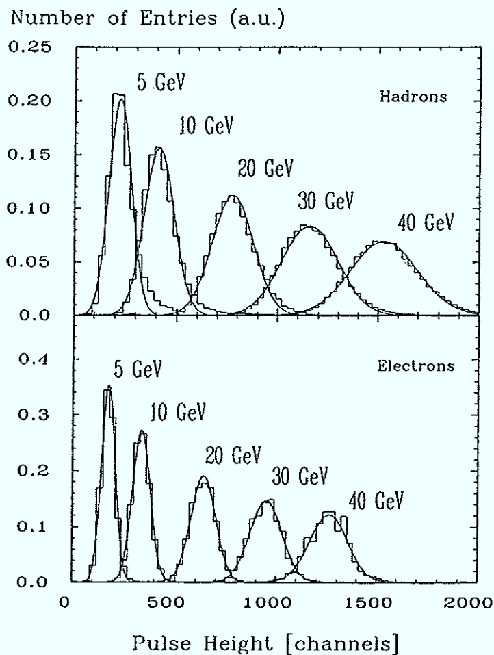
Fig. 4.17 Hadron and Electron Response in the Uranium Part for Various Beam Energies.
