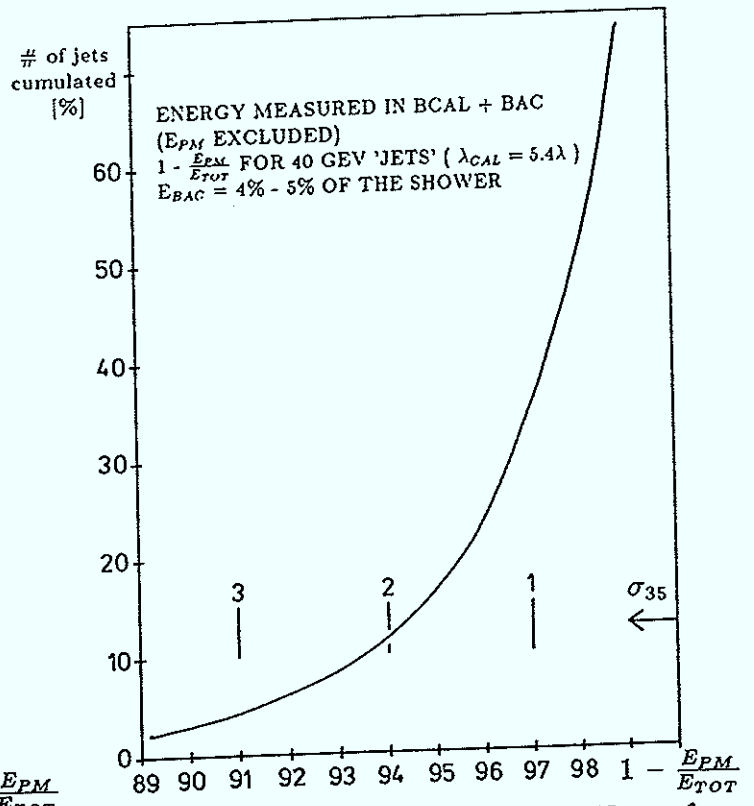
Fig. 4.42 Fraction of 40 GeV 'Jets' as Fct. of 1 - \frac{E_{PM}}{E_{TOT}} for E_{BAC} = 4\% - 5\% of the Shower Energy; \lambda_{CAL} = 5.4\lambda .
