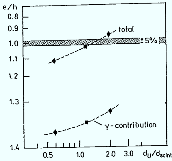
Figure 3.22 The e/h -ratio as a function of the ratio of uranium to scintillator plate thickness R_d = d_U/d_{Scint} .
