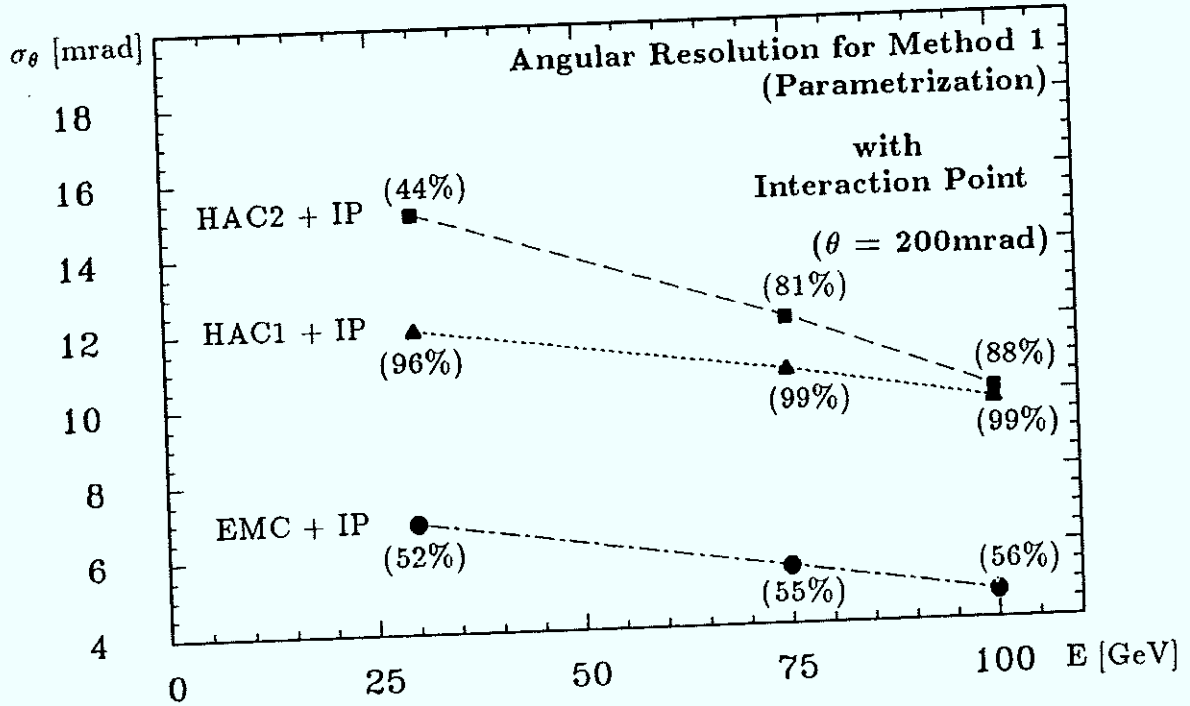
Fig. 5.59 Angular resolution as a function of the energy of the hadron shower at \theta = 200\text{mrad} for combinations of EMC + IP, HAC1 + IP and HAC2 + IP. The fractions of hadron showers are indicated in brackets.
