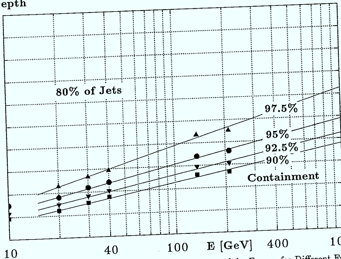
Fig. 4.47b Calorimeter Depth for 80% of 'Jets' as Function of the Energy for Different Fractions of Shower Containment.
