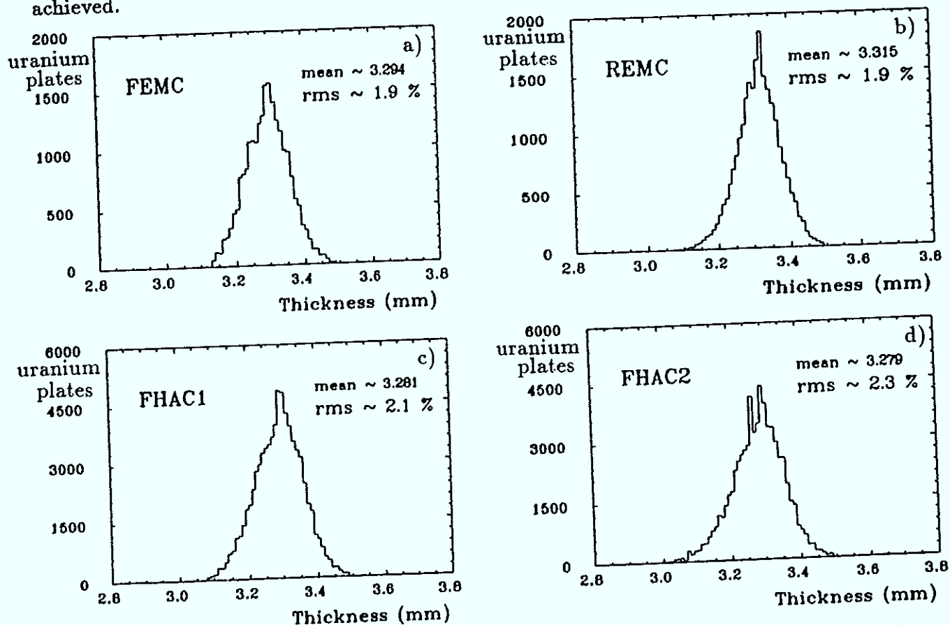
Fig. 6.4 Thickness distributions of uranium plates for a) EMC sections of FCAL, b) EMC sections of RCAL, c) HAC1 and d) HAC2 sections of FCAL.
