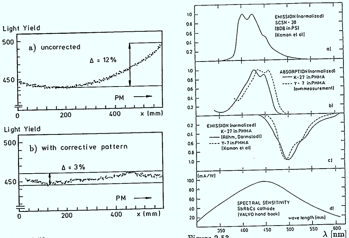
Figure 2.52 Uniformity of a FHAC1 WLS measured with a xenon lamp a) before and b) after correction.
