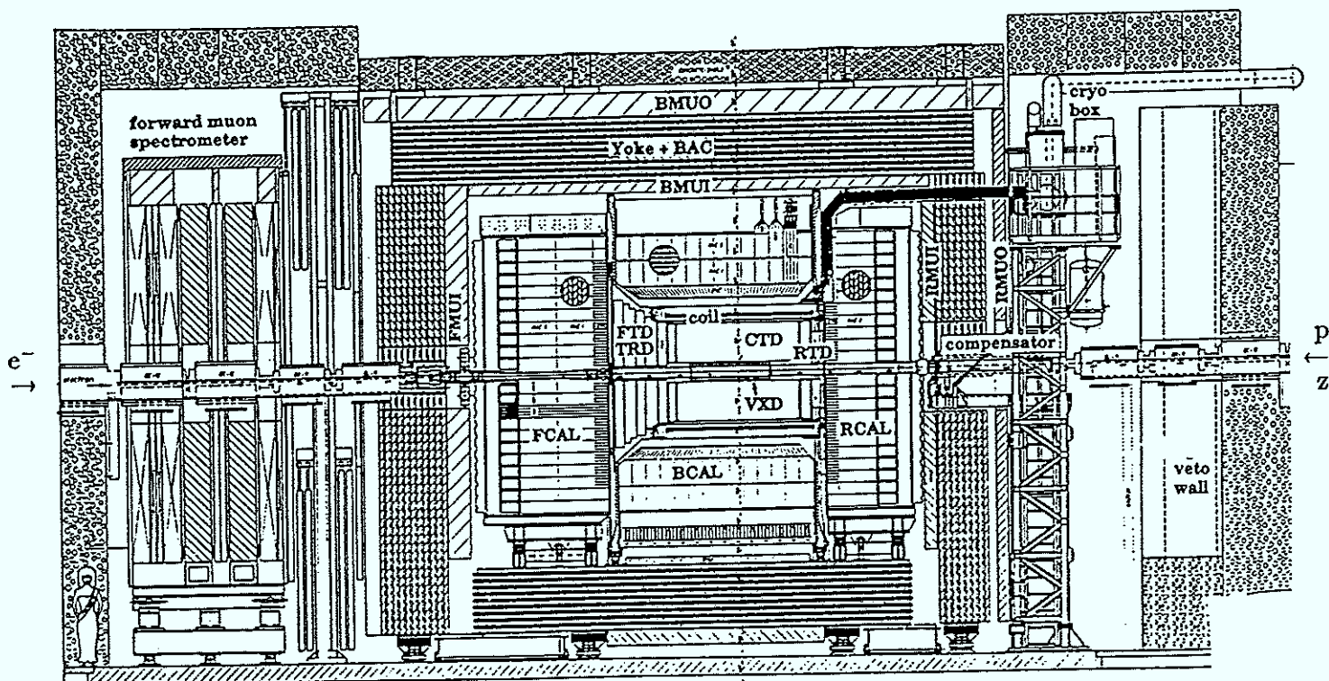
Fig. 2.34 Section of the ZEUS detector along the beam.
