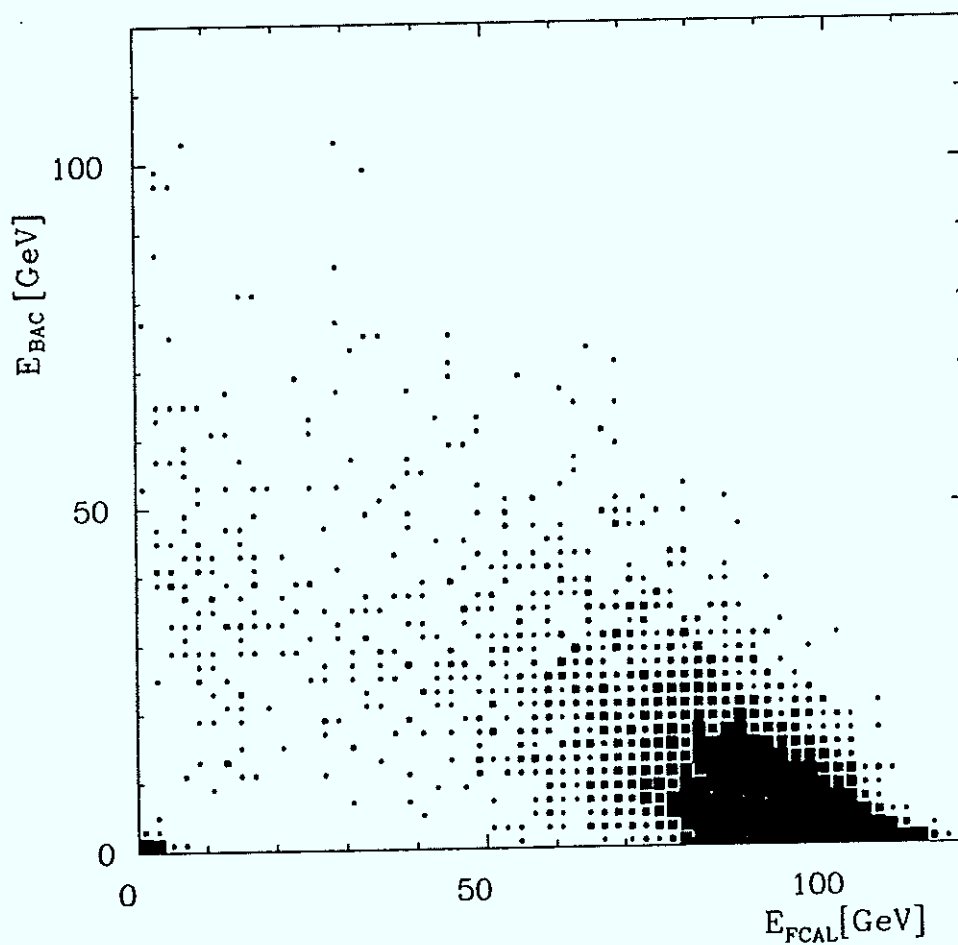
Fig. 2.58 Correlation between the energy measured in the BAC prototype calorimeter E_{BAC} and the FCAL prototype calorimeter E_{FCAL} for 100 GeV hadrons.
