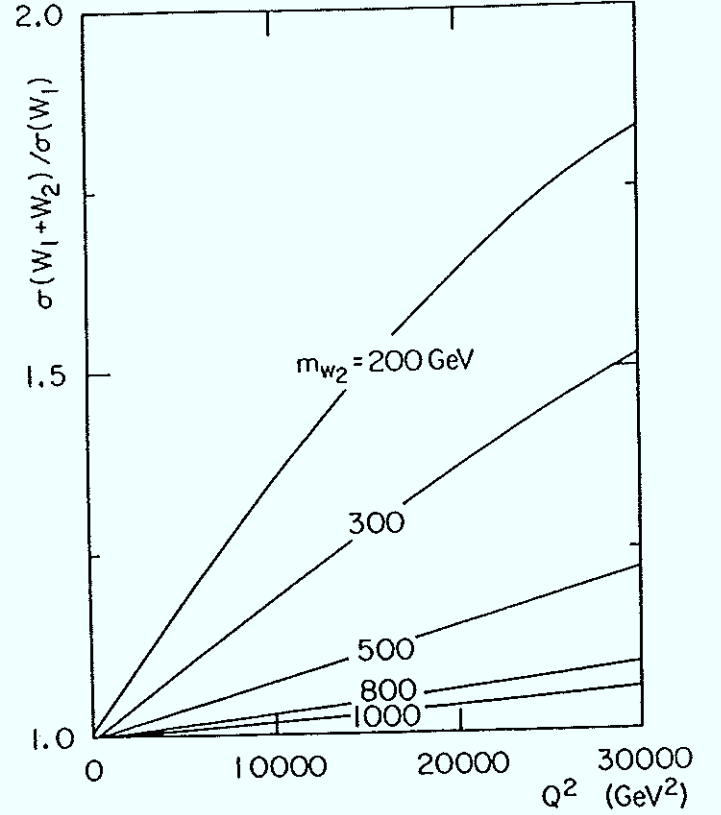
Fig. 2.27 Ratio of the cross sections of \sigma(W_1 + W_2) to \sigma(W_1) .
