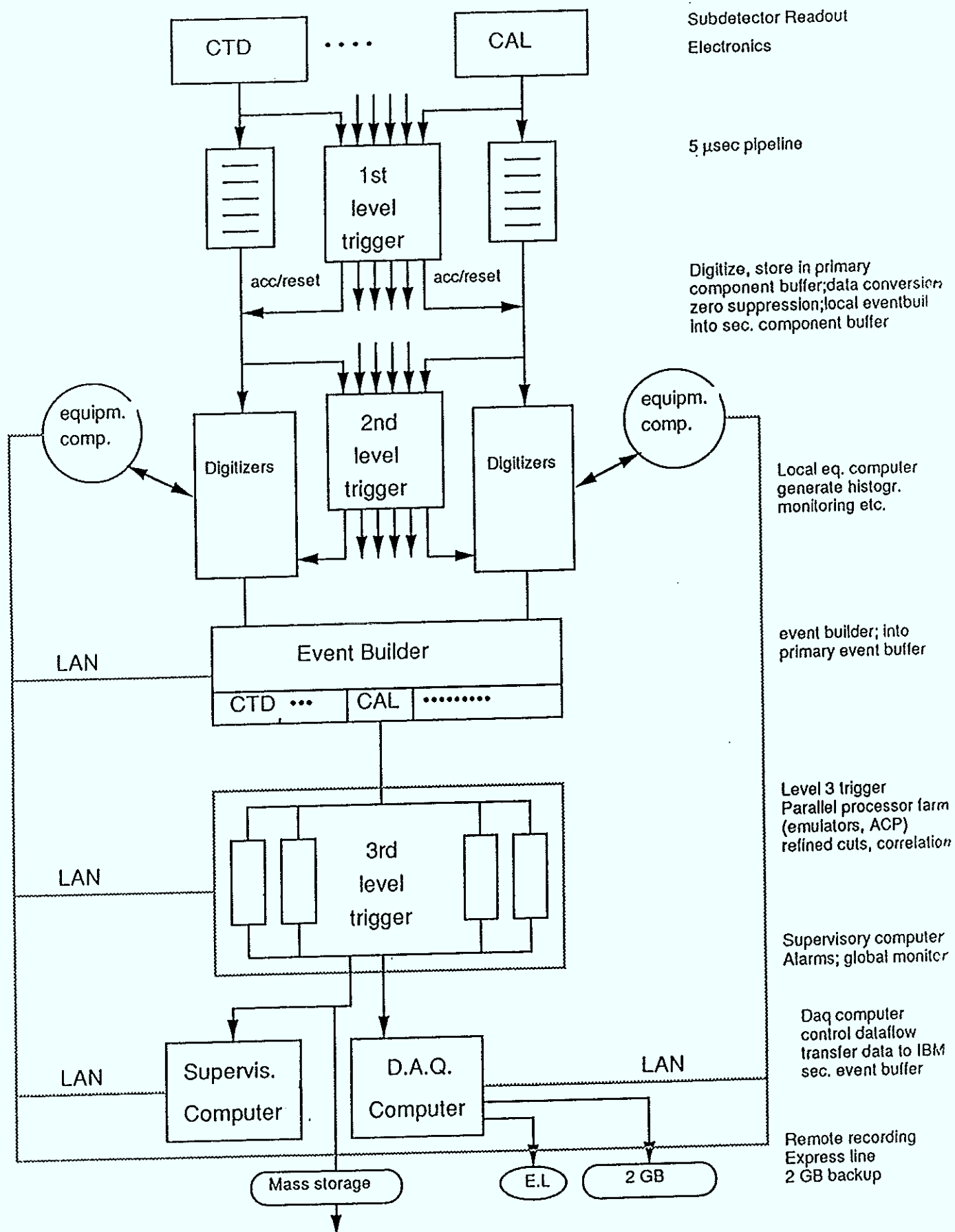
Fig. 2.77 Outline of the ZEUS Data Acquisition System.
