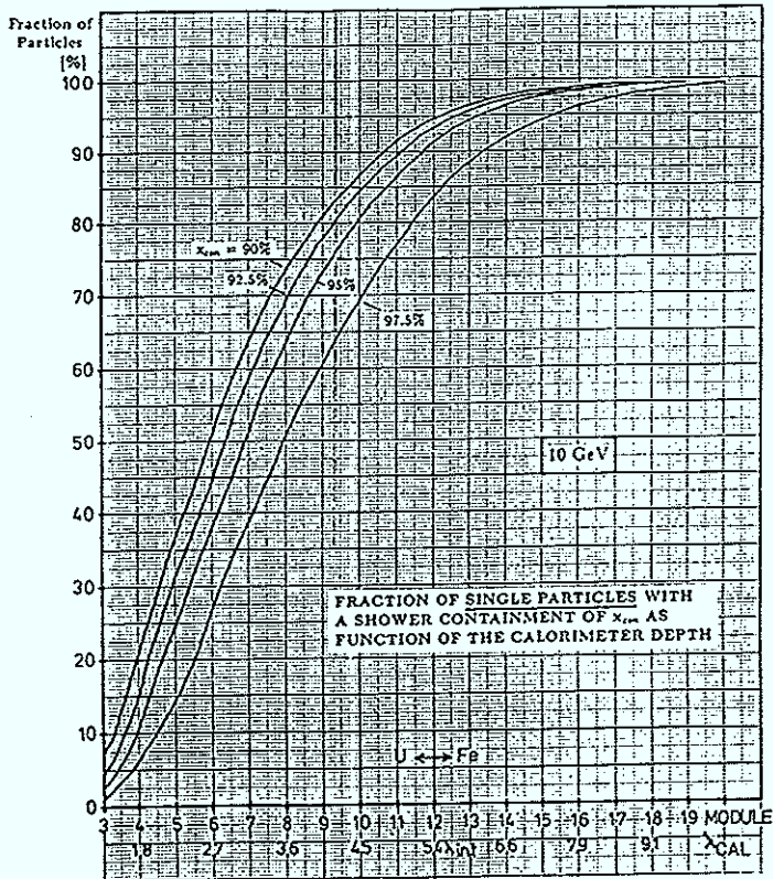
Fig. 4.30a Fraction of single particles with a shower containment of x_{cen} as function of the calorimeter depth \lambda_{CAL} for 10 GeV.
