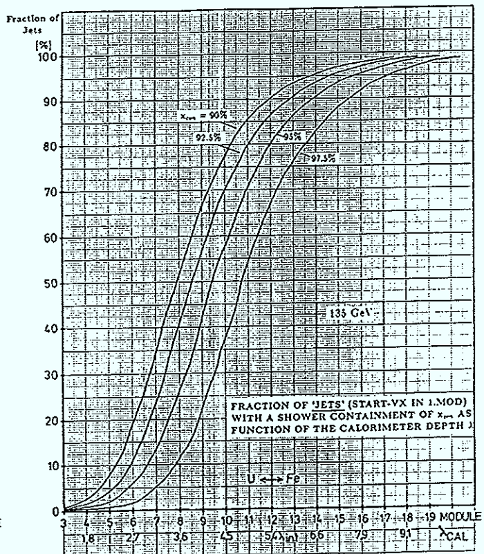
Fig. 4.34b Fraction of 'jets' with a shower containment of x_{con} as function of the calorimeter depth \lambda_{CAL} for 135 GeV.
