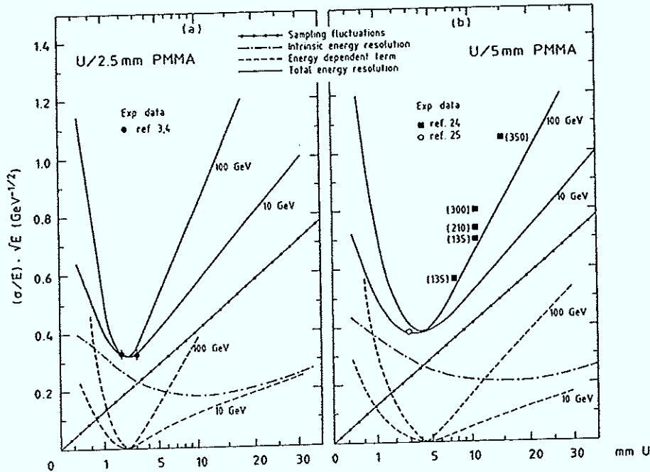
Fig. 3.24 The total energy resolution and the various contributions for 10 GeV and 100 GeV hadrons in uranium scintillator calorimeters as a function of the uranium plate thickness for 2.5 mm (a) and 5 mm (b) thick scintillator layers. The numbers in brackets denote the energies at which the experimental results were reported from Wigmans.
