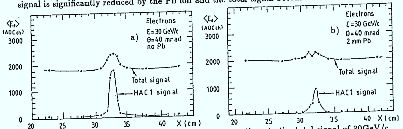
Fig. 5.23 Contribution of the different calorimeter sections to the total signal of 30GeV/c electrons for 40mrad beam incidence a) without and b) with a 2mm thick Pb foil between modules 2 and 3.
