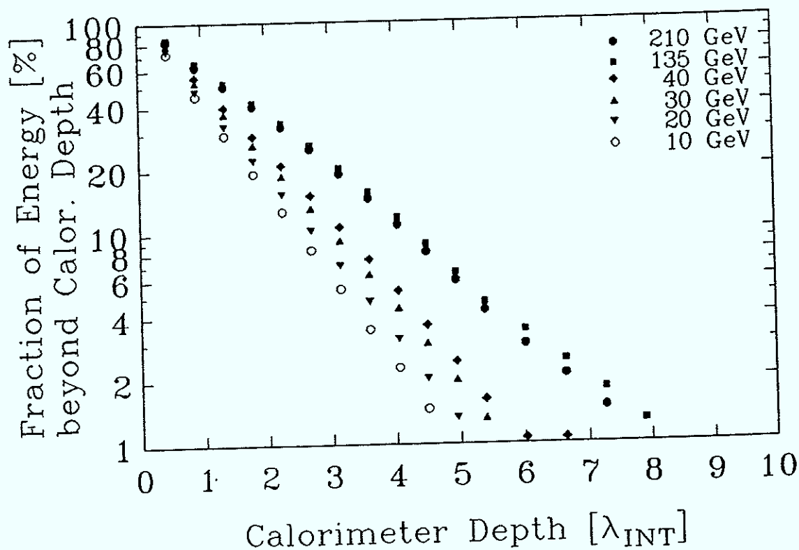
Fig. 4.22 Cumulative Distributions of Longitudinal Shower Profiles for Events with Shower Vertex in the First Module.
