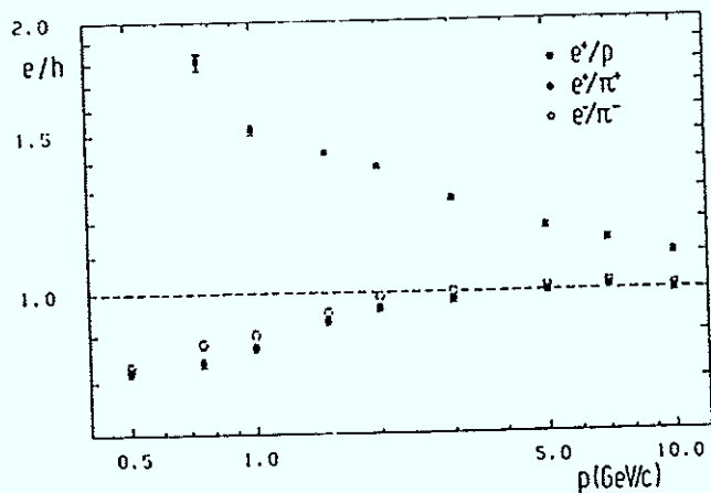
Figure 5.17 e/h -ratio as a function of the momentum for \pi^+ , \pi^- and p .
