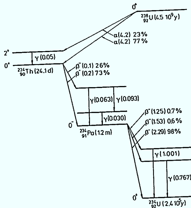
Fig. 6.6 Decay chain of ^{238}_{92}\text{U} into ^{234}_{92}\text{U} , including only the main decay lines and indicating the energy in MeV of the emitted particles.
