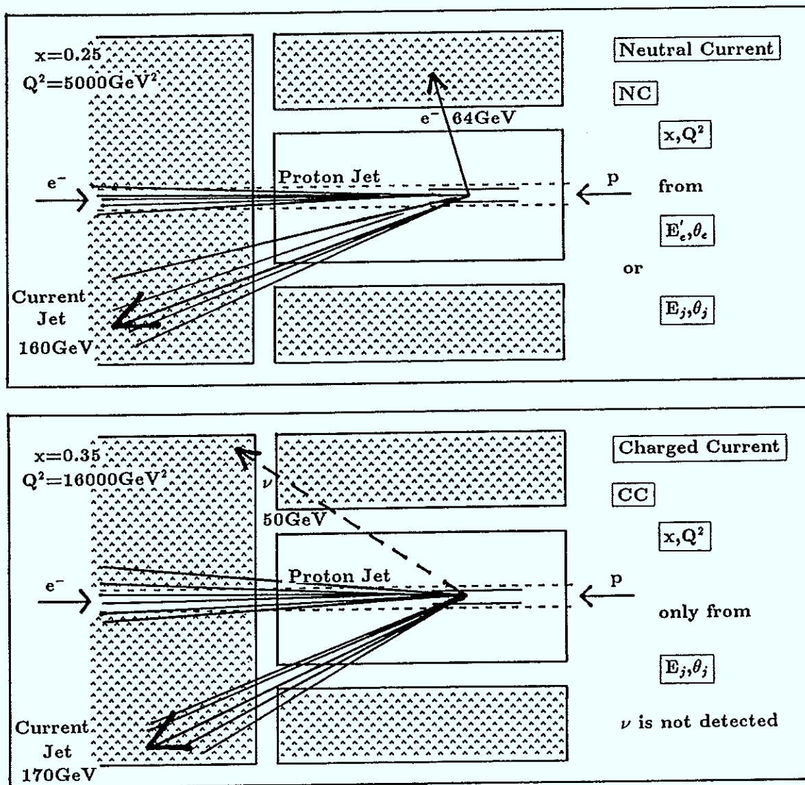
Fig. 2.31 Monte Carlo simulated neutral current (NC) and charged current (CC) events.
