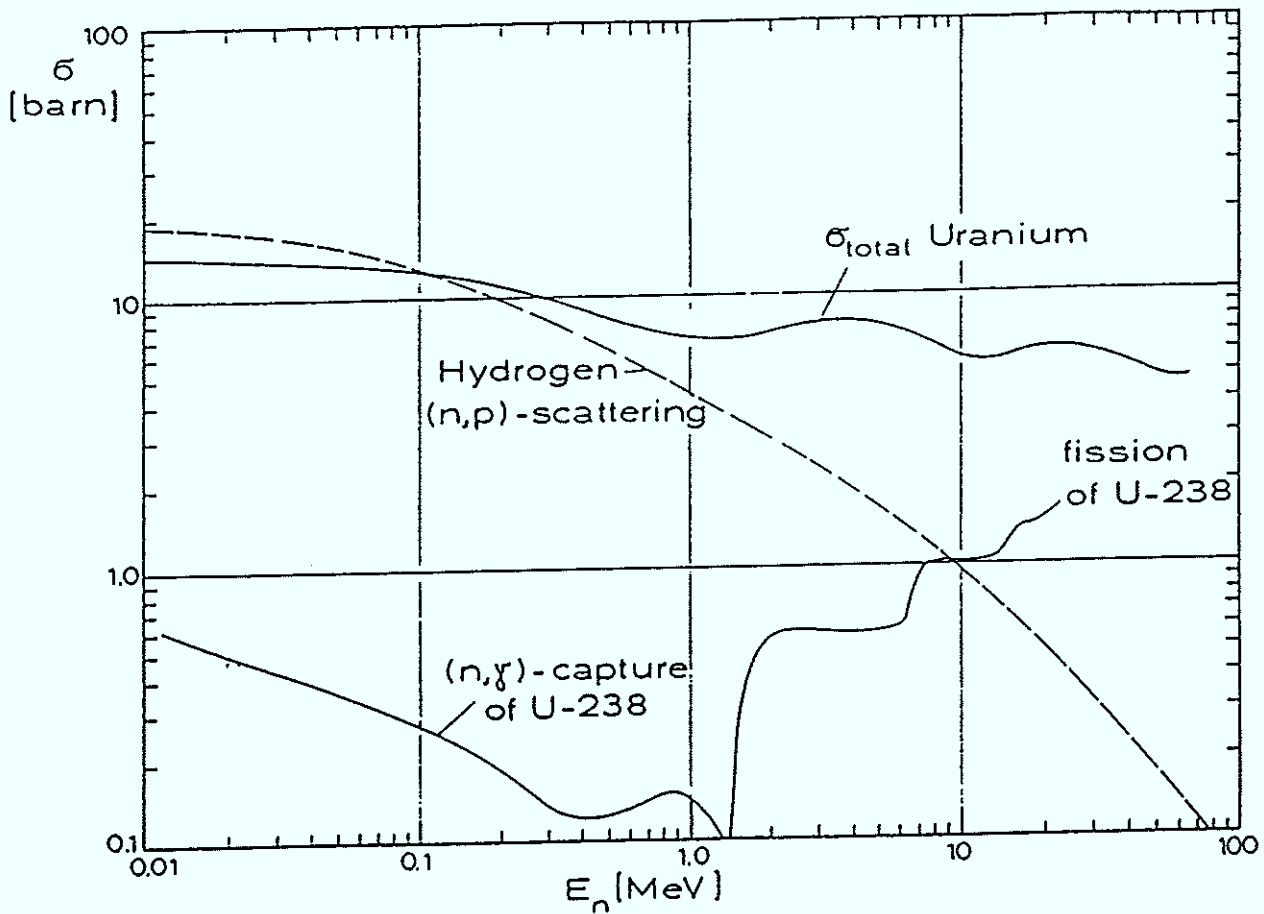
Fig. 3.18 Cross sections for neutron induced reactions on uranium and hydrogen.
