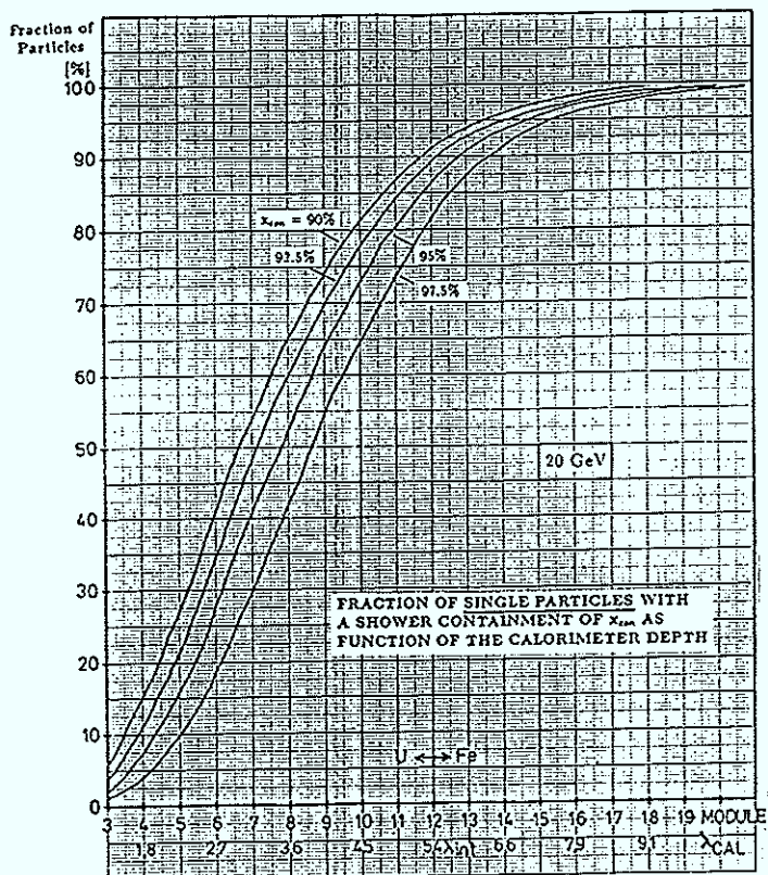
Fig. 4.31a Fraction of single particles with a shower containment of x_{cen} as function of the calorimeter depth \lambda_{CAL} for 20 GeV.
