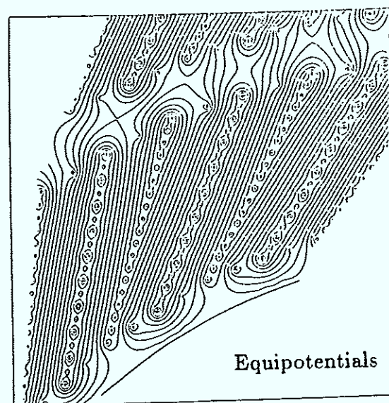
Figure 2.62 Equipotentials and electron drift trajectories in superlayer 1.
