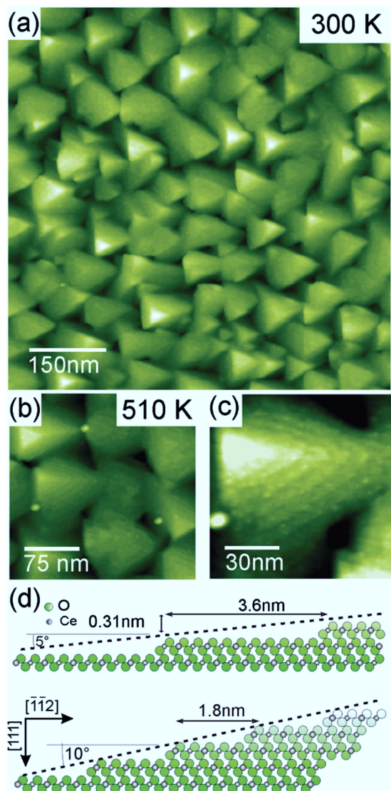
Fig. 20 (a) to (c) NC-AFM images taken on a cub- \text{CeO}_2(111) sample representing (a) the as-prepared ceria sample and (b and c) the sample heated to a temperature of 510 K. The terrace structure of the pyramid is clearly seen in (c). Bright spots preferentially attached to step edges are due to contaminants that could not be removed by the heat treatment. (d) Side view model for the bottom (typically 10) and top (typically 5) layers of the pyramids yielding nominal values for the terrace widths and slope angles. (Reproduced from ref. 131.)
