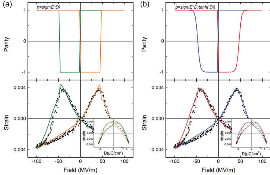
Figure S10. Parity function. Example of (a) square and (b) gradual parity function for a P(VDF-TrFE) capacitor, with the corresponding fits of the S-E characteristics shown. The insets show the fits for the S-D representation of the data.
