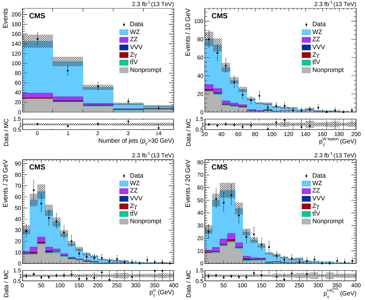
Figure 2: (upper left) Distribution of the number of jets with p_T > 30 GeV in the event. (upper right) Transverse momentum of the lepton associated with the W boson. (lower left) Transverse momentum of selected Z boson candidates. (lower right) Transverse momentum of selected W boson candidates. Solid symbols represent the data with statistical uncertainty, while histograms represent the expected WZ signal and backgrounds. Uncertainties in signal and background yields include experimental systematic, theoretical, and integrated luminosity uncertainties in addition to the statistical uncertainty. The background shapes are taken from simulation or data, as described in the text.
