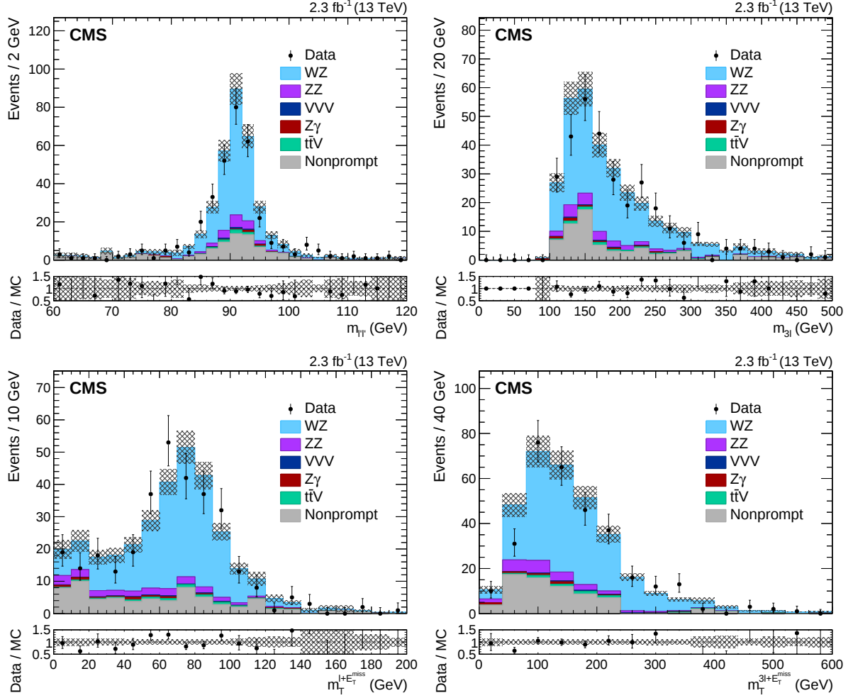
Figure 1: (upper left) Distribution of the reconstructed \ell'\ell' pair mass summed for all decay channels with the m_{\ell'\ell'} selection extended to 60–120 GeV. (upper right) Distribution of the \ell\ell'\ell' reconstructed mass summed for all decay channels with the m_{3\ell} > 100 GeV selection requirement removed. (lower left) The transverse mass of the lepton from the W boson and the E_T^{\text{miss}} system. (lower right) The transverse mass of the three leptons and the E_T^{\text{miss}} system. Solid symbols represent the data with statistical uncertainty, while histograms represent the expected WZ signal and backgrounds. Uncertainties in the signal and background yields include experimental systematic, theoretical, and integrated luminosity uncertainties in addition to the statistical uncertainty. The background shapes are taken from simulation or data, as described in the text.
