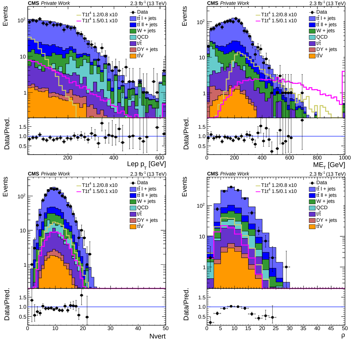
Fig. C.2: Distributions of the lepton p_T (top, left), E_T (top, right) and number of reconstructed PV (bottom, left) and average hadronic activity (bottom, right) after the baseline selection. The shapes of the lepton p_T and E_T distributions are affected by the L_T threshold, but also show a good data-MC agreement. The pileup distribution shows that the previously discussed corrections provide a good agreement, as well as the average hadronic activity, that is used to subtract the effect of pileup energy from the jet energy.
