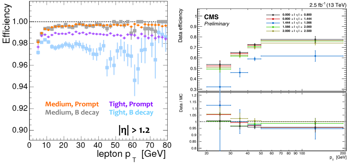
Fig. 4.3: Left : muon identification efficiency in simulated t\bar{t} events for the medium and tight criteria [134]. The medium WP shows a high and stable efficiency for prompt muons, as well as from b-decays. Right : electron identification efficiency with the tight WP in data and a comparison to the simulation expectation [135]. Except for the barrel-endcap overlap region, the efficiency is similar over the whole pseudorapidity range, and in good agreement with simulation.
