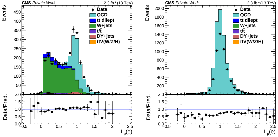
Fig. 6.14: L_p distributions for selected ( left ) and anti-selected ( right ) electron events after the baseline selection with modified requirements of n_{\text{jet}} \in [3, 4] and zero b-tags. In this phase-space the selected events are composed of similar contributions from the EWK and QCD backgrounds, however the former is modelled better, than the latter. The anti-selected sample is dominated by QCD events, as intended for a fake electron enriched selection.
