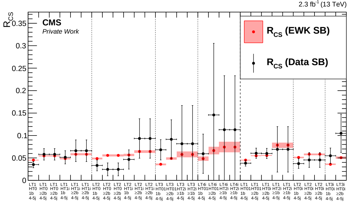
Fig. 6.27: R_{CS} values in the sideband regions as expected from the EWK backgrounds in simulation (red) and as observed in data (black). The error bands correspond to the statistical uncertainties only. Despite some large statistical uncertainties, the agreement is satisfactory in the majority of the categories.
