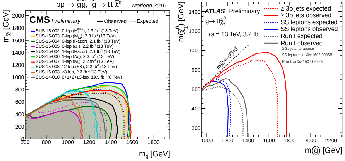
Fig. 7.8: Exclusions limits at 95% C.L. on the simplified SUSY model of gluino pair production with subsequent decay \tilde{g} \rightarrow t\bar{t}\tilde{\chi}_1^0 obtained by the CMS [181] (left) and ATLAS [182] (right) collaborations. The Run 1 results demonstrate the respective strongest exclusion achieved. SUS-15-006 corresponds to results obtained by the present analysis.
