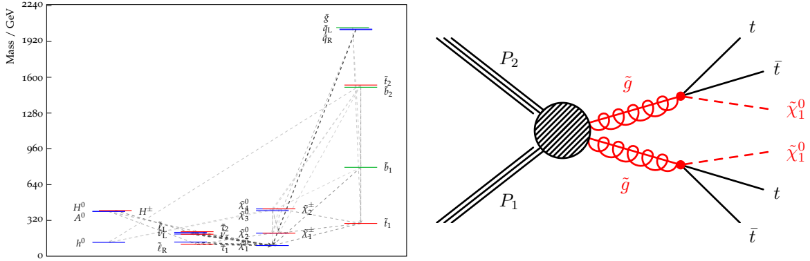
Fig. 1.3: Left : SUSY particle spectrum for a pMSSM model [43]. The dashed lines indicate possible decay channels, with darker colours representing higher branching ratios.
