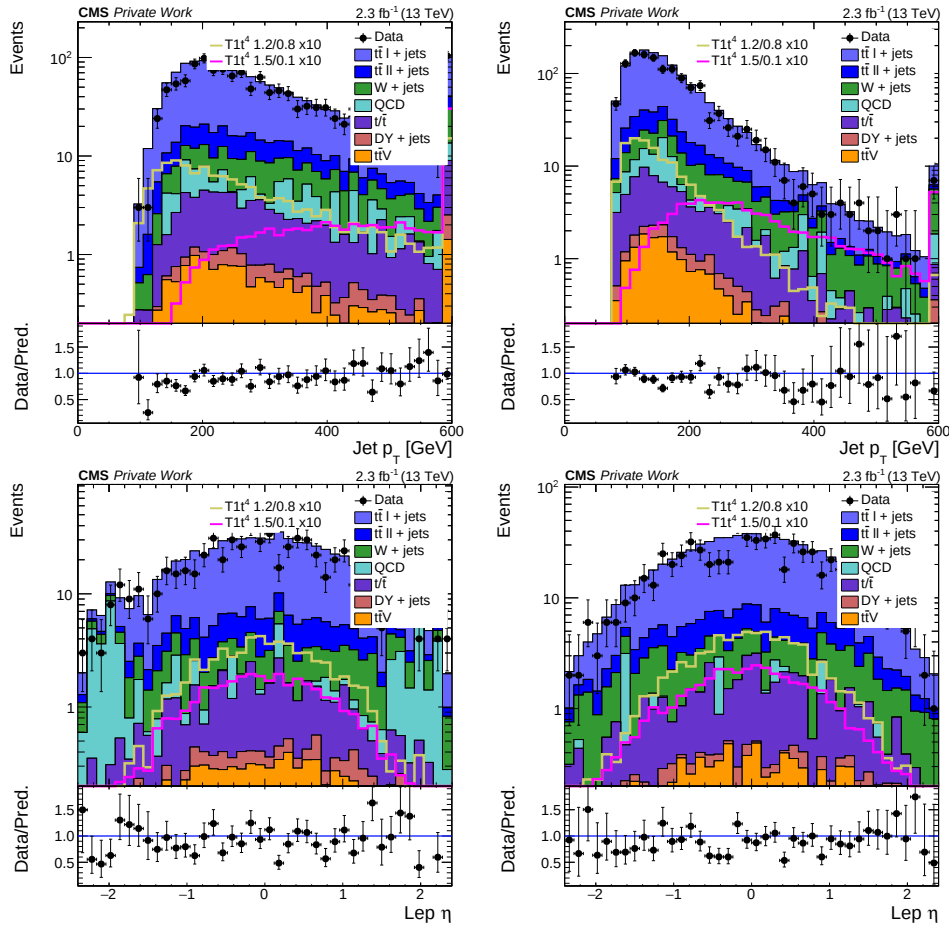
Fig. C.1: Distributions of the leading (top, left) and subleading (top, right) jet transverse momenta and electron (bottom, left) and muon (bottom, right) pseudorapidity after the baseline selection. Similar to the H_T distribution, the non-compressed T1tttt (1500,100) scenario dominates the high values of the jet momentum spectra in the top figures. The pseudorapidity distributions allow to see the different contribution of the QCD background for electron and muon events.
