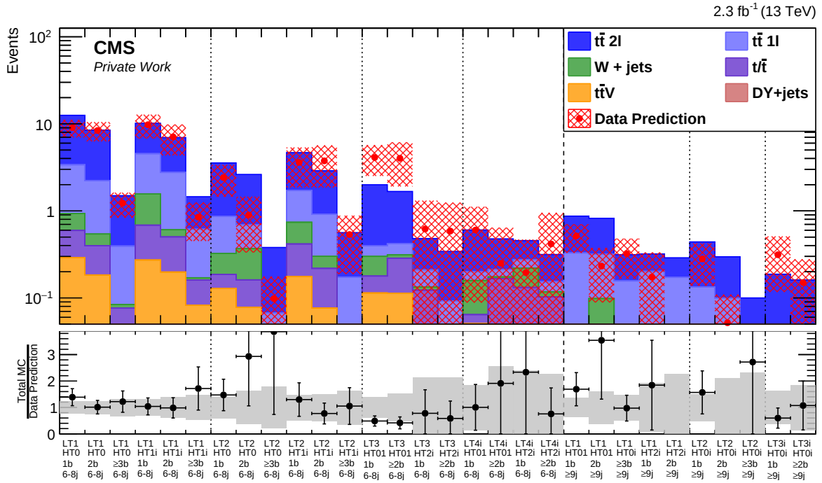
Fig. 6.28: Comparison of simulated event yields and the data-driven predictions in the signal regions of the mainband. The lower panel shows the ratio of the total background from simulation over the data prediction. The grey band shows the total uncertainty on the prediction. In general, a good agreement is observed for the majority of the bins, with no systematic over- or underestimation.
