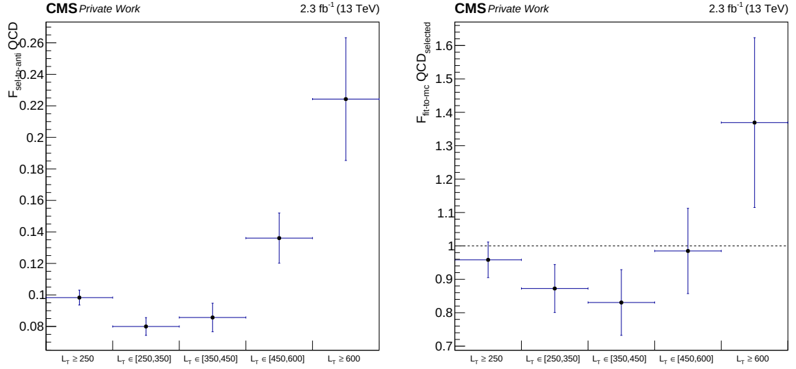
Fig. 6.17: The left plot shows the values of F_{\text{sel-to-anti}} from the fits to pseudo-data in different L_T bins with n_{\text{b-tag}} = 0, n_{\text{jet}} \in [3, 4] . The measured ratios are in agreement with the values based on the MC yields. Due to the decreasing sample, the statistical uncertainties rise with L_T . The comparison of the number of selected QCD events from the fit and MC yields in the corresponding bins is shown on the right .
