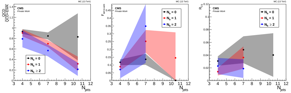
Fig. 6.23: Properties of the QCD background in simulated anti-selected muon events versus n_{\text{jet}} for L_T > 250 GeV and H_T > 500 GeV: fraction of multijet events over the sum of QCD, t\bar{t} +jets and W+jets (left), the selected to anti-selected ratio F_{\text{sel-to-anti}} (middle) and the R_{\text{CS}} factor (right).
