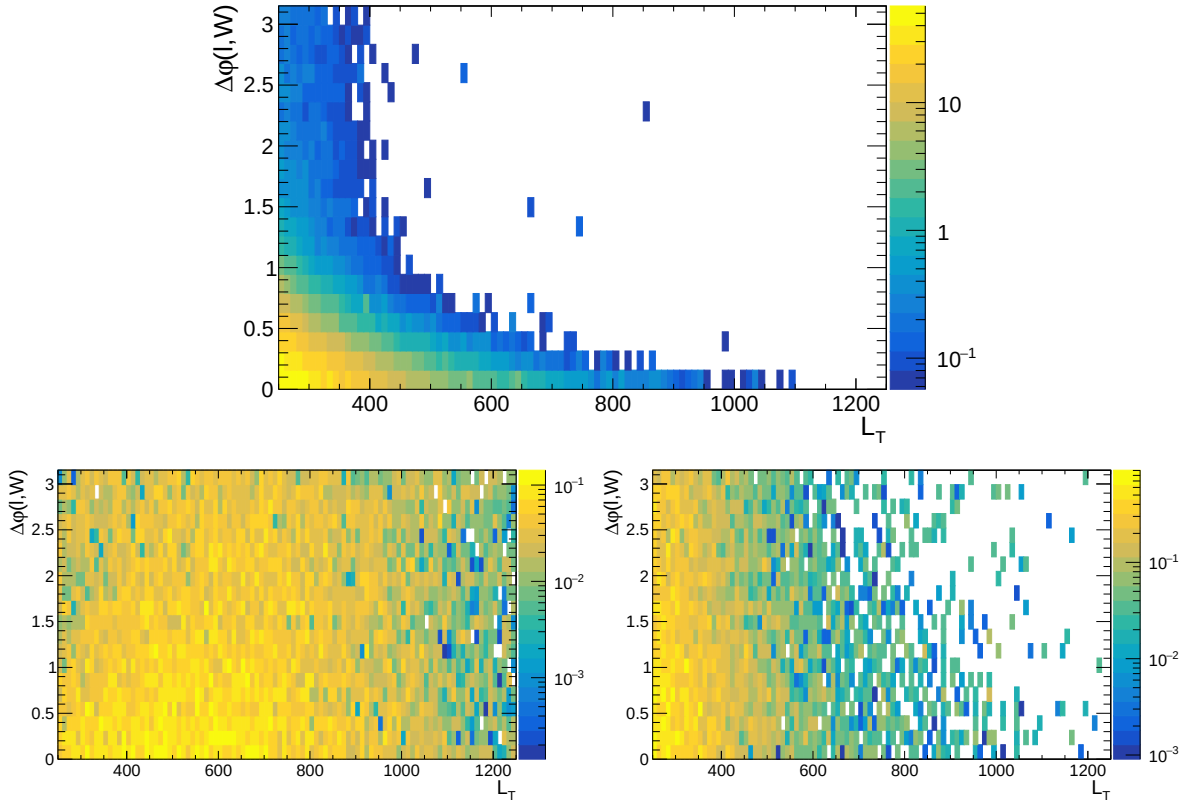
Fig. 5.10: Distribution of simulated EWK background ( top ) and signal T1tttt (1500,100) ( left ), T1tttt (1200,800) ( right ) events in the the \Delta\phi vs. L_T plane after the preselection. While the signal shows no correlation of those variables, the \Delta\phi of background events decreases towards large values of L_T .
