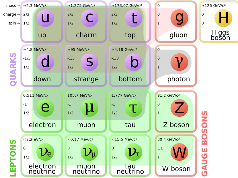
Fig. 1.1: All fundamental particles of the Standard Model with three generations of matter, the gauge and Higgs bosons; the electric charge, spin and mass (or limit for neutrinos) are given in the corners of the boxes. The shaded areas indicate which particles couple to which gauge boson according to the different interactions [16].
