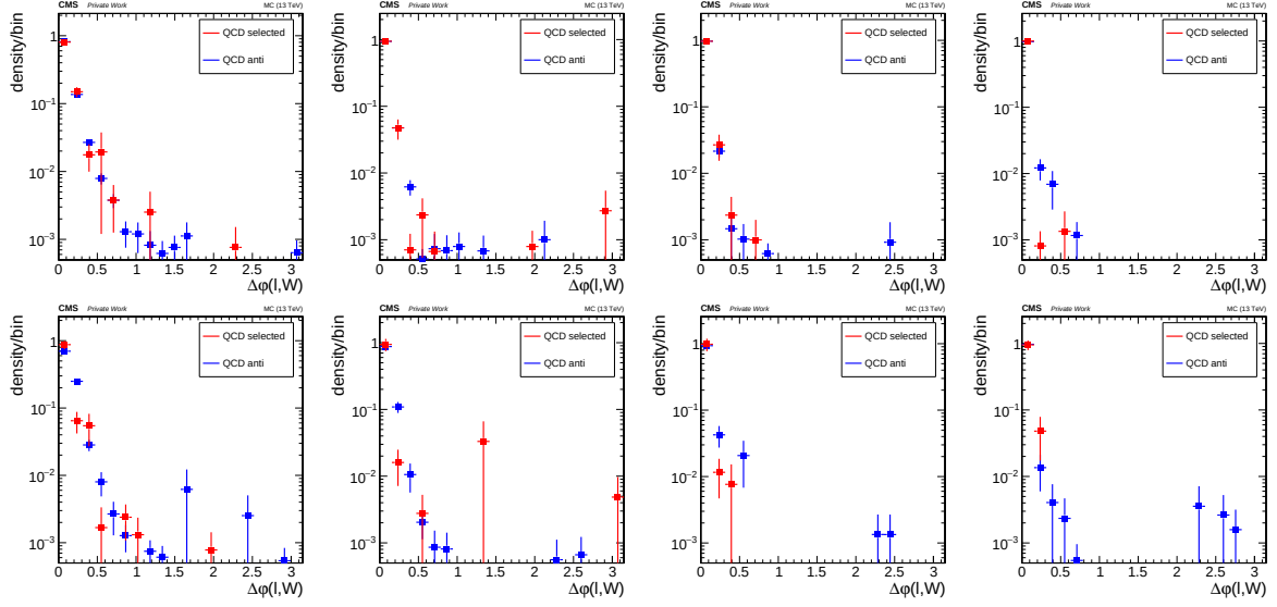
Fig. D.2: Shapes of \Delta\phi for selected and anti-selected QCD events in n_{\text{jet}} \in [4, 5] (top) and n_{\text{jet}} \geq 6 (bottom) for different L_T bins in simulation: [250, 350] , [350, 450] , [450, 600] and > 600 GeV.
