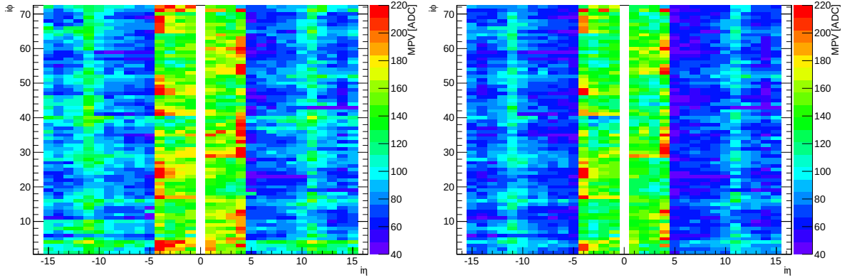
Fig. 3.14: Landau fit MPVs of nominal ( left ) and path-length corrected signal ( right ) obtained from HO global run data. The uncorrected signal MPVs show an i\phi modulation due to the incident angle of the muon. The central ring signal is twice as high due to the double layer of scintillators. Compare to the local run results in Fig. 3.8.
