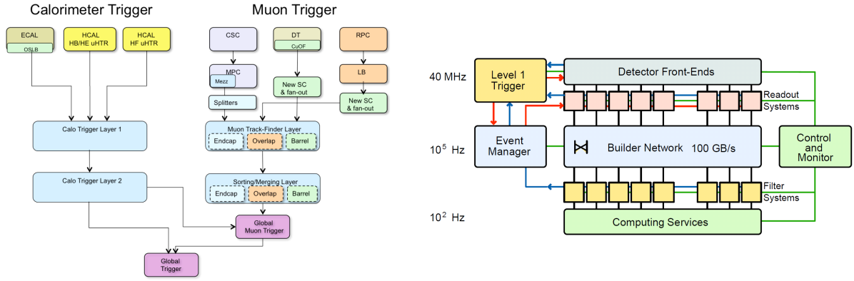
Fig. 2.11: Dataflow of the upgraded Level-1 Trigger [93] (left). The general architecture of the CMS Data Acquisition (DAQ) system [73] during Run 1 (right) shows the key building blocks for a single slice.
