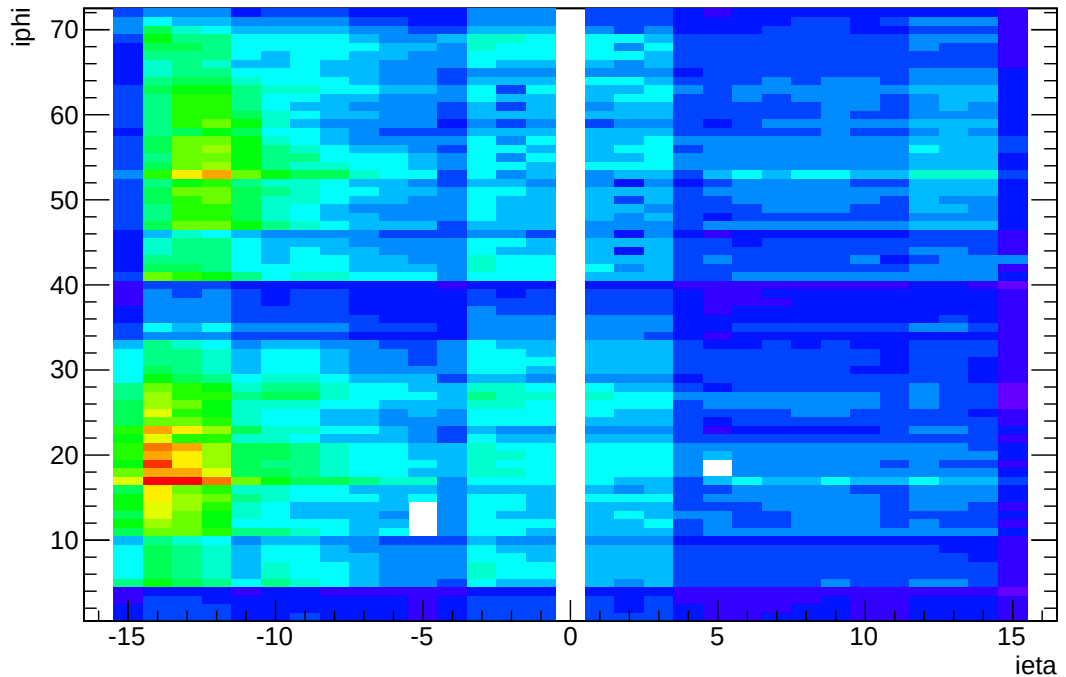
Fig. 3.6: Occupancy of the individual HO channels in a self-triggered run. The tiles with i\eta < -10 are close to the cavern shaft. Horizontal sectors are within 10 < i\phi < 30 and 45 < i\phi < 65 . The white spots at i\eta = \pm 5 correspond to the magnet chimneys and are not instrumented with tiles.
