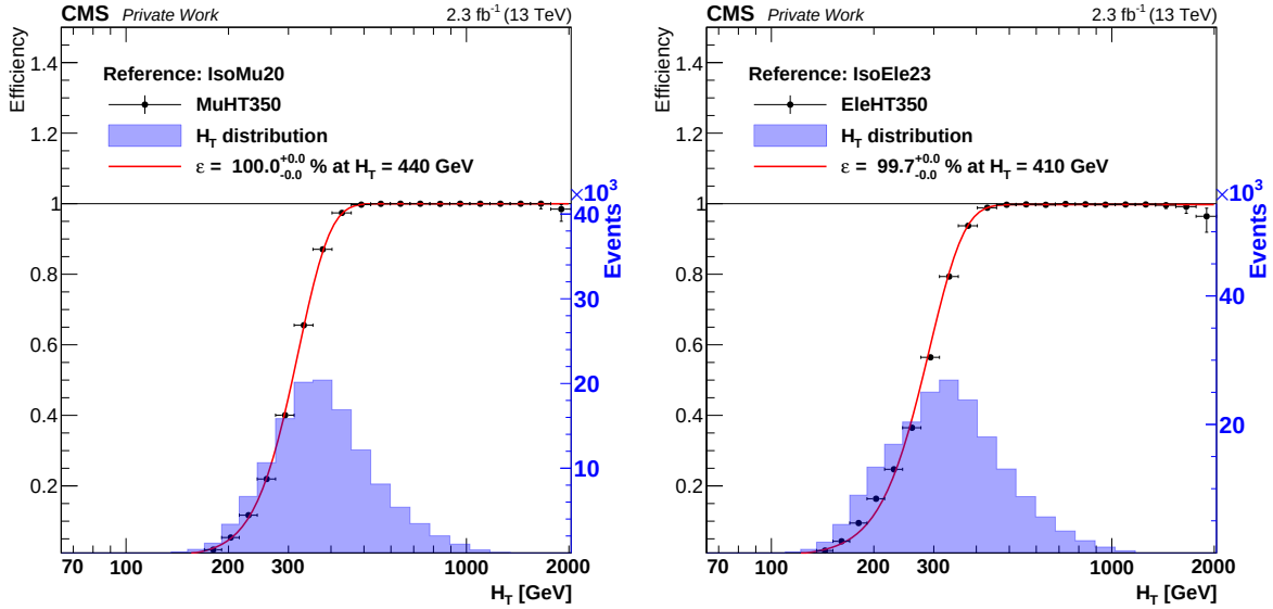
Fig. 5.4: Efficiency of the H_T leg for the analysis HLT paths including a muon HLT_Mu15_IsoVVVL_PFHT350 (left) or an electron HLT_Ele15_IsoVVVL_PFHT350 (right). The baseline selection requires the events to pass a corresponding single isolated lepton trigger (HLT_IsoMu20 or HLT_Ele23_WPLoose_Gsf) and contain a single good lepton with p_T > 25 GeV.
