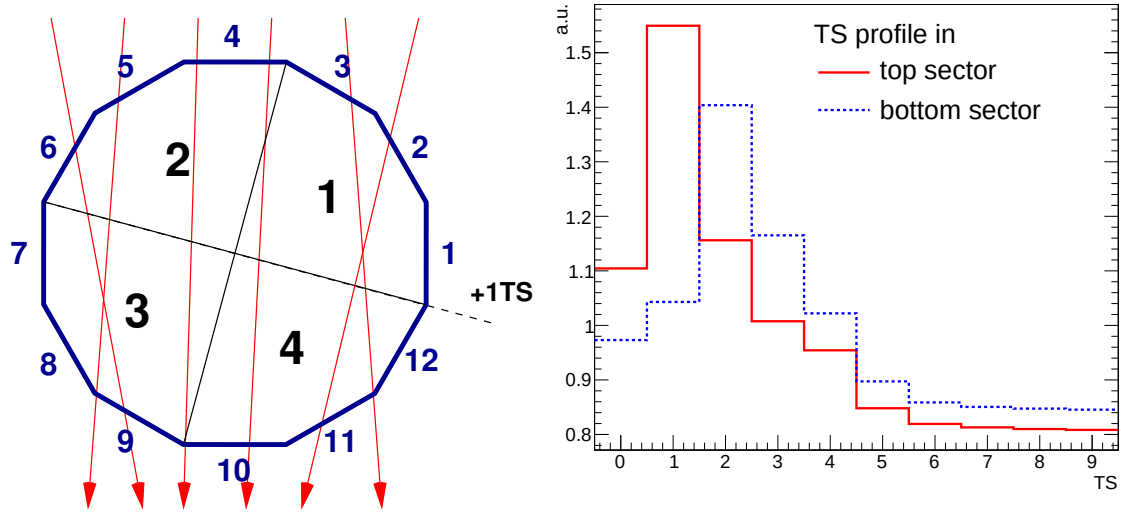
Fig. 3.5: Left : Configuration of the TTP quadrants in HO. The coincidence trigger is fired if a signal is seen in two separate quadrants. A time delay of 1 TS is required between the top and bottom sectors. Right : Comparison of averaged TS profiles for an up and down sector channel. The first bins show the signal shape, while the last ones are zero-suppressed.
