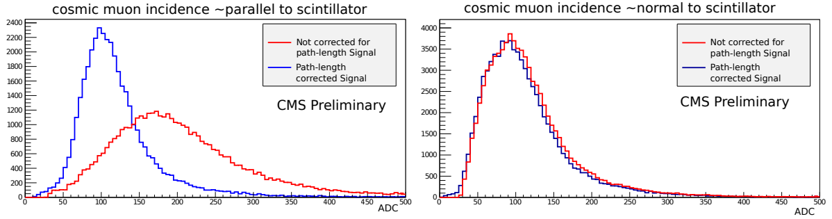
Fig. 3.10: Muon signal spectra for vertically aligned ( Left ) and horizontal ( Right ) tiles with and without the HO muon path-length correction. The signal distribution of the side channel is narrowed and shifted towards a smaller MPV, while for the top channel the changes are marginal.
