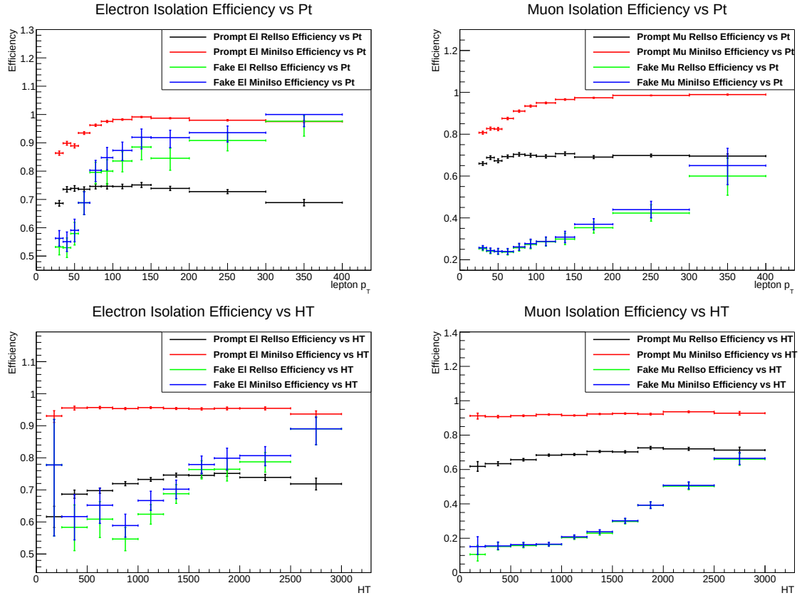
Fig. B.1: Isolation efficiency for T1tttt(1500,100) events with upper requirements of I < 0.1 for both isolation types. Mini-isolation improves the efficiency of prompt leptons in general w.r.t. the fixed-cone isolation, and also remains efficient at high p_T and H_T .
