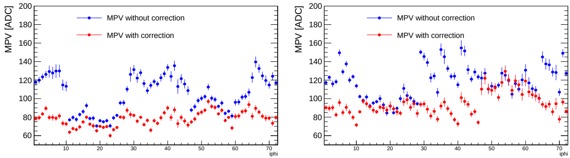
Fig. 3.11: Profile of nominal and path-length corrected MPVs averaged over the i\eta axis for Rings \pm 1,2 ( Left ) and Ring 0 ( Right ). The nominal values (blue) show a modulation along the i\phi axis, while the muon path-length correction equalizes the MPVs. The remaining structure is due to hardware differences between the channels.
