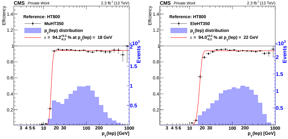
Fig. 5.3: Efficiency of the lepton p_T leg for the analysis HLT paths including a muon HLT_Mu15_IsoVVVL_PFHT350 (left) or an electron HLT_Ele15_IsoVVVL_PFHT350 (right). The baseline selection requires the events to pass a pure H_T trigger HLT_PFHT800 and contain a single good lepton with p_T > 10 GeV.
