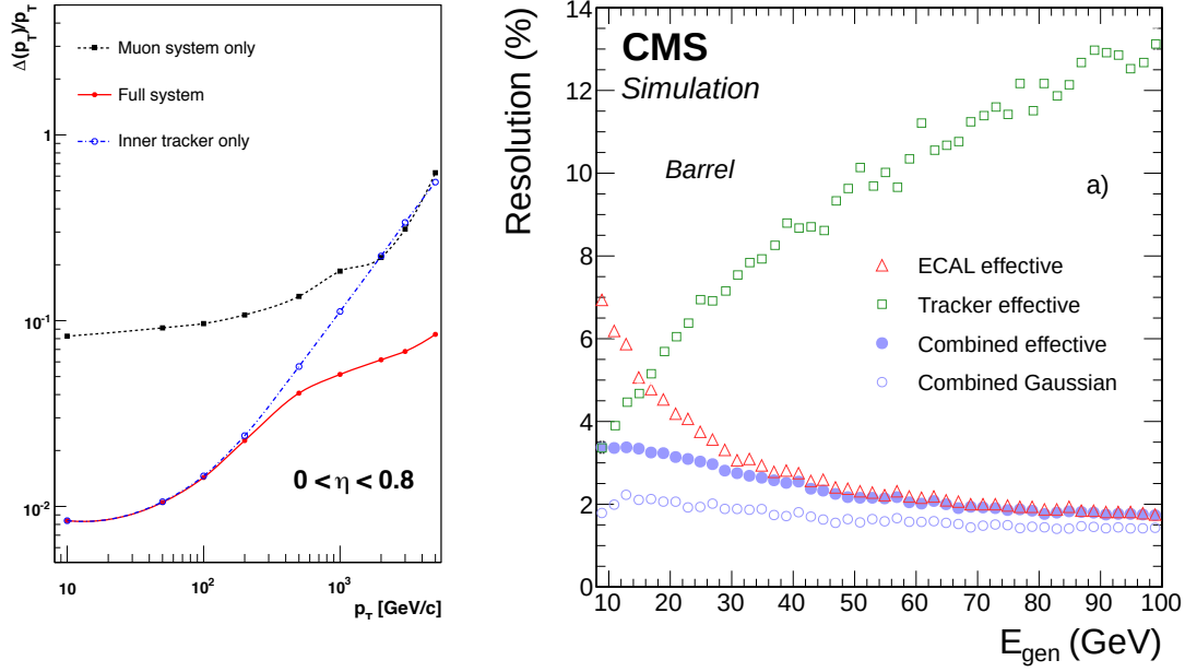
Fig. 4.2: Left : comparison of the muon transverse momentum resolution for global muons (red), tracker-only muons (blue) and tracks reconstructed only in the muon system (black) [73]. The low p_T resolution is mainly driven by the inner tracker. Right : energy resolution for electrons reconstructed using only the track (squares) or the ECAL (triangles) in comparison to the combined measurement as used by the PF algorithm (circles) [125].
