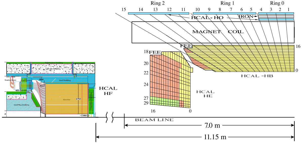
Fig. 2.8: Schematic view of a quarter of the CMS HCAL subsystems. For the central HCAL detectors (right) the tiles with the same color are read out by a single channel [85]. The HF (left) segmentation is explained in the text [86].
