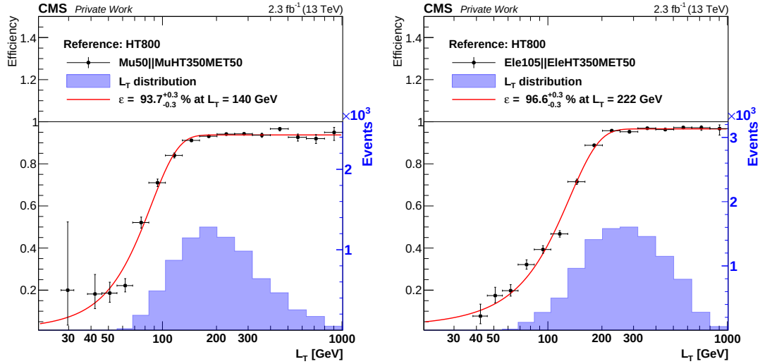
Fig. A.3: Efficiency of the combined isolated and non-isolated lepton HLT trigger paths for muons ( left ) and electrons ( right ). The black dashed lines indicate the analysis selection threshold L_T = 250 GeV. The reference selection requires the events to pass a pure H_T trigger HLT_PFHT800 and contain a single lepton with p_T > 10 GeV.
