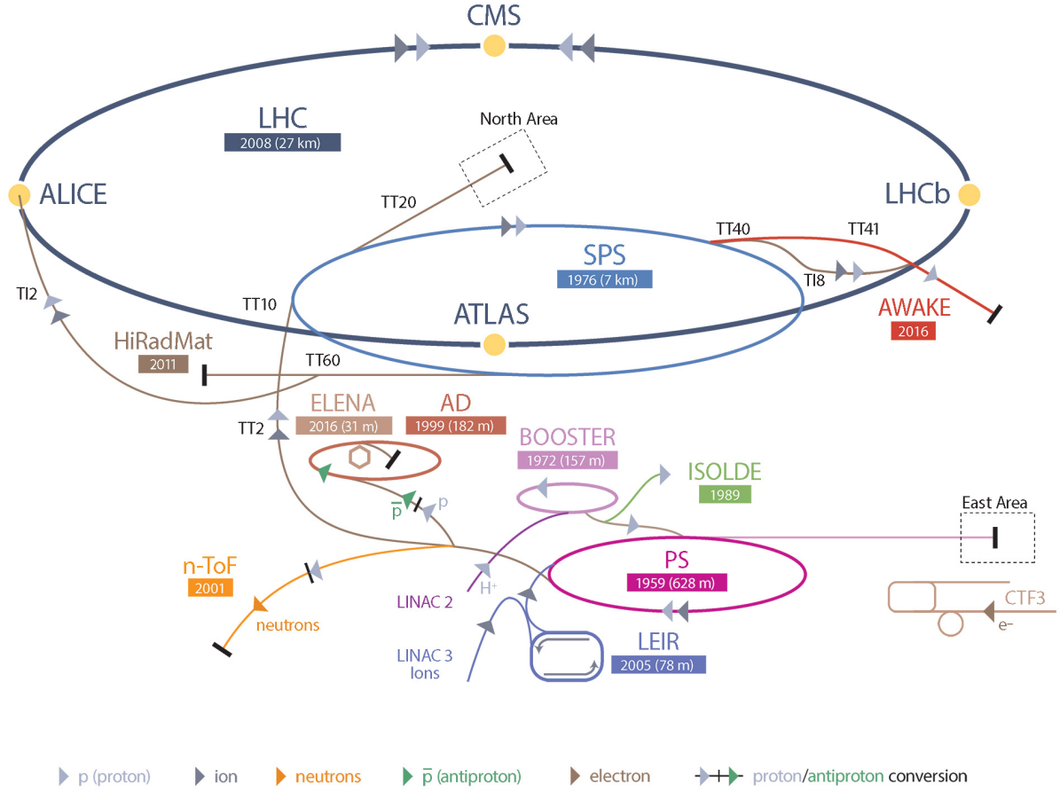
Fig. 2.2: The accelerator complex of CERN [67]: a schematic overview of the operating accelerators, storage rings and beam transfer lines. The location of the major LHC experiments is also indicated.
