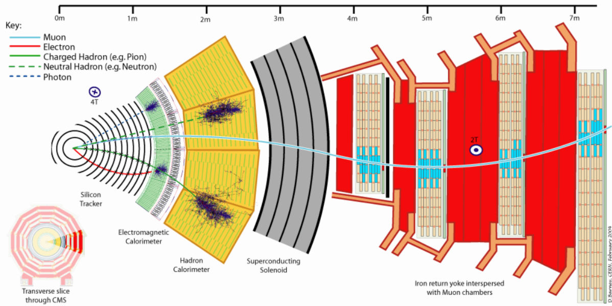
Fig. 4.1: Slice of the CMS detector in the transverse plane with some characteristic particles crossing the subsystems indicated [119]. For simplicity, only energy deposits in the most relevant subdetectors are shown.
