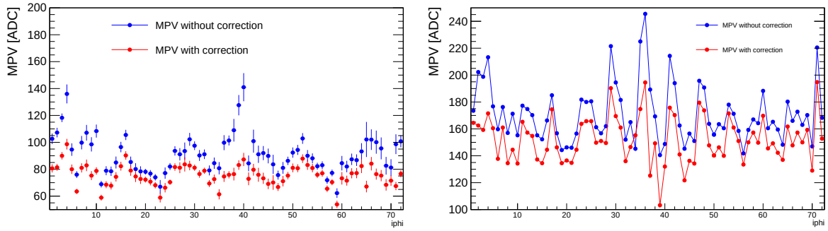
Fig. 3.15: Profile of nominal and path-length corrected MPVs averaged over the i\eta axis for Rings \pm 1,2 ( left ) and Ring\ 0 ( right ) obtained from global runs. The nominal values (blue) show a modulation along the i\phi axis, while the muon path-length correction equalizes the MPVs. The remaining structure is due to hardware differences between the channels. Ring\ 0 MPVs are higher due to the two layers.
