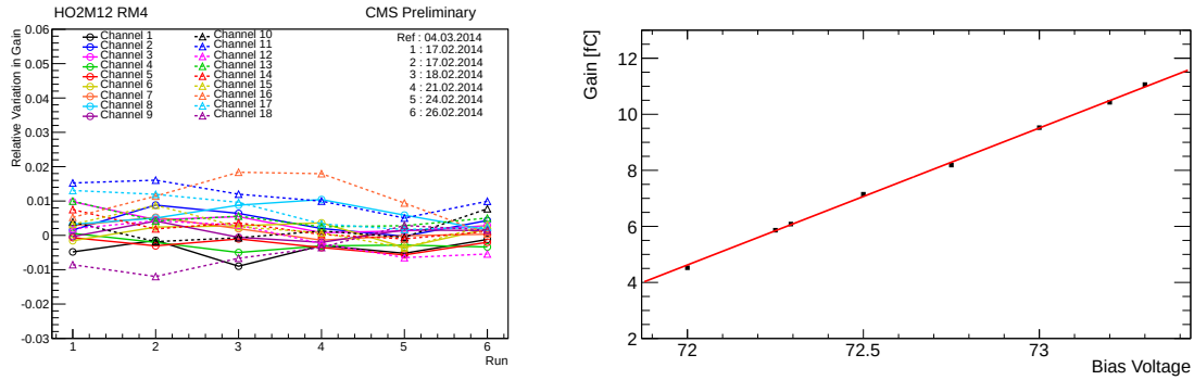
Fig. 3.4: Left : Relative variation of the SiPM gain over time for a single RM with 18 channels [113]. Right : Gain vs. bias voltage distribution for one SiPM fitted with a linear function [112]. The extrapolation of the line to zero gain provides the breakdown voltage.
