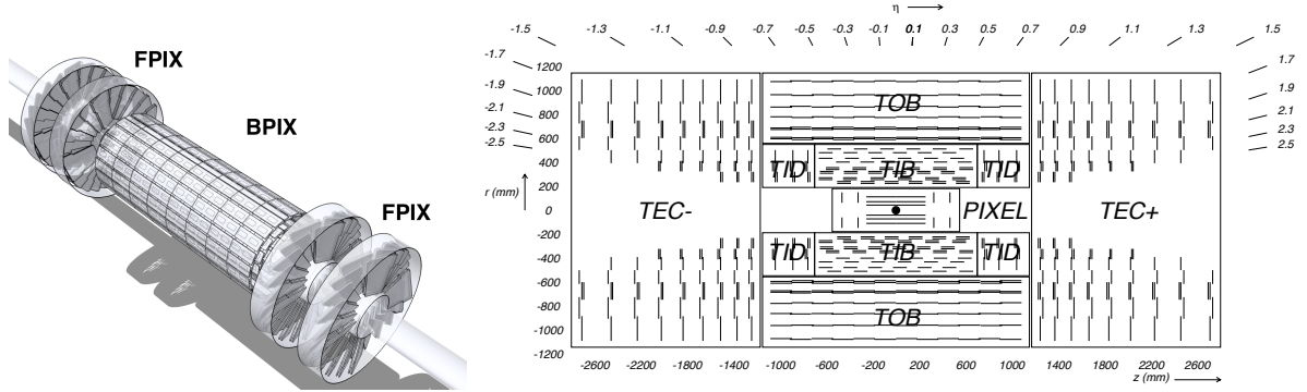
Fig. 2.6: The inner silicon tracking system of CMS. Left : the pixel barrel (BPix) and forward (FPix) detectors depicted by a 3D model [81]. Right : schematic view of the tracker in the r - z plane, with the silicon strip tracker segments labelled individually. Each line represents a detector module. Double lines indicate back-to-back modules which deliver stereo hits [73].
