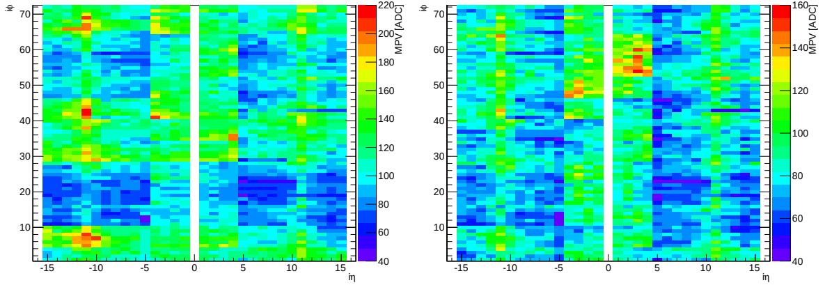
Fig. 3.8: Landau fit most probable values (MPVs) of nominal ( Left ) and path-length corrected signal ( Right ) obtained from HO local run data. The uncorrected signal MPVs show an i\phi modulation due to the incident angle of the muon.
