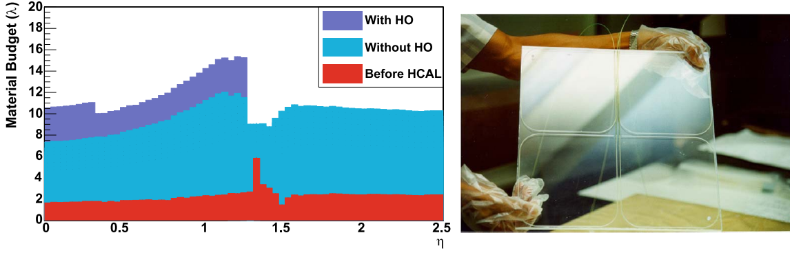
Fig. 2.9: Left : material budget (in units of nuclear interaction length) with and without the HO, as well as before the HCAL [87]. Right : an HO scintillator tile with four embedded fibres (“sigma grooves”); this group corresponds to a single tower in the HB and is read out together by a single channel.
