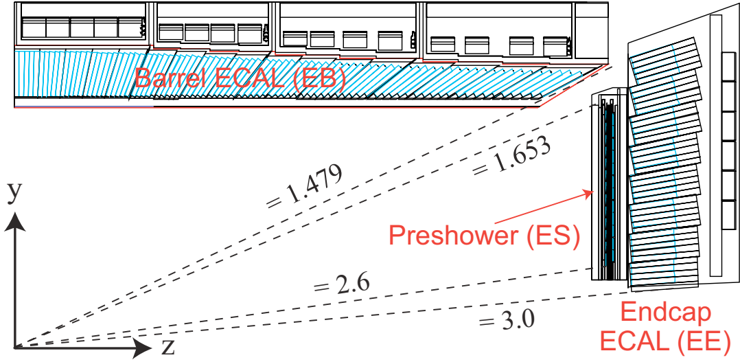
Fig. 2.7: Layout of an ECAL quarter with its subsystems indicated [83], their geometric acceptances are shown with the dashed lines. The \text{PbWO}_4 crystals are highlighted in blue.
