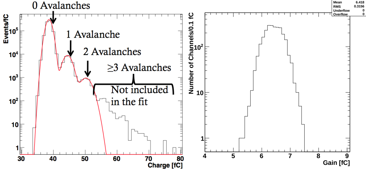
Fig. 3.3: Left : Charge distribution in dark events for one SiPM. The integration time here is 100 ns (4TS). The first peak corresponds to the pedestal distribution, where no pixel fires, followed by the SPE peaks. A three-peak fit (red line) is performed to extract the gain [110]. Right : Distribution of gain for all SiPMs installed in HO as measured from the dark spectrum [112].
