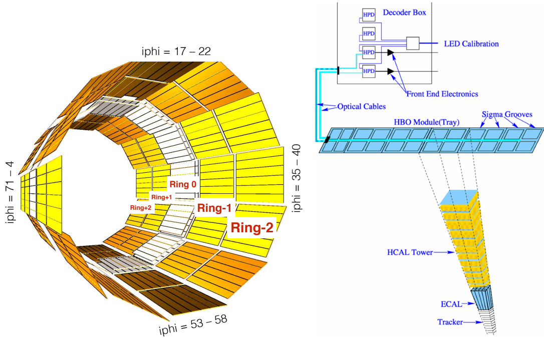
Fig. 3.1: Left : layout of the HO scintillator trays. There are five rings with twelve sectors each. The i\phi coordinates are shown for the horizontal and vertical sectors. Right : HO scintillator tray and corresponding HB projective tower [87]. The light from the four fibres in the HO tower is combined in a decoder box and then measured by the photodetectors.
