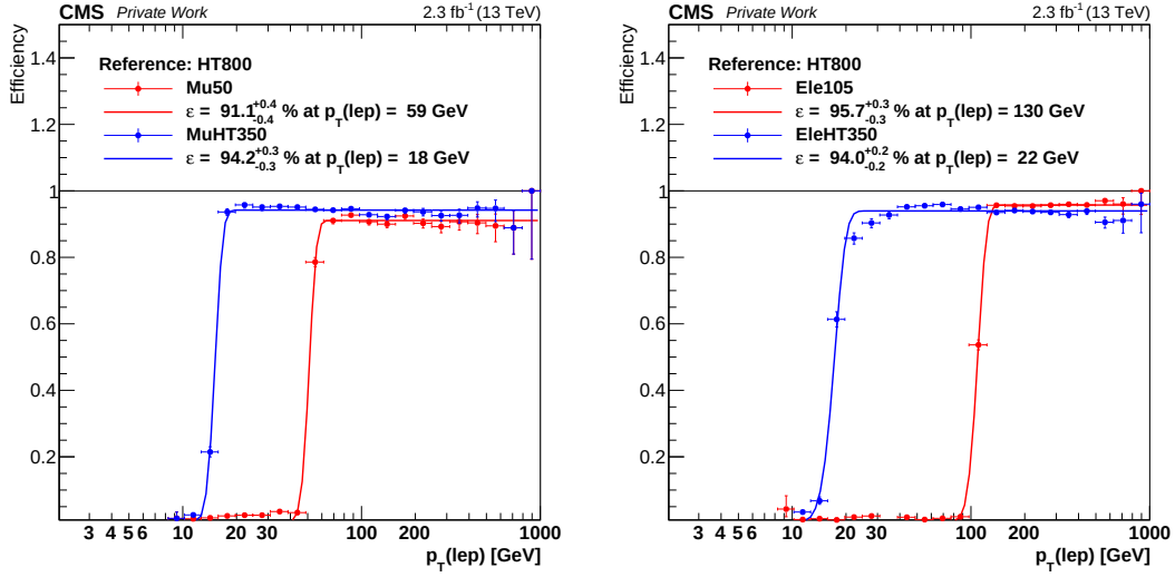
Fig. A.1: Efficiency of the lepton p_T leg for the main and backup analysis HLT paths with isolated and non-isolated leptons, respectively. The reference selection requires the events to pass a pure H_T trigger HLT_PFHT800 and contain a single lepton with p_T > 10 GeV.
