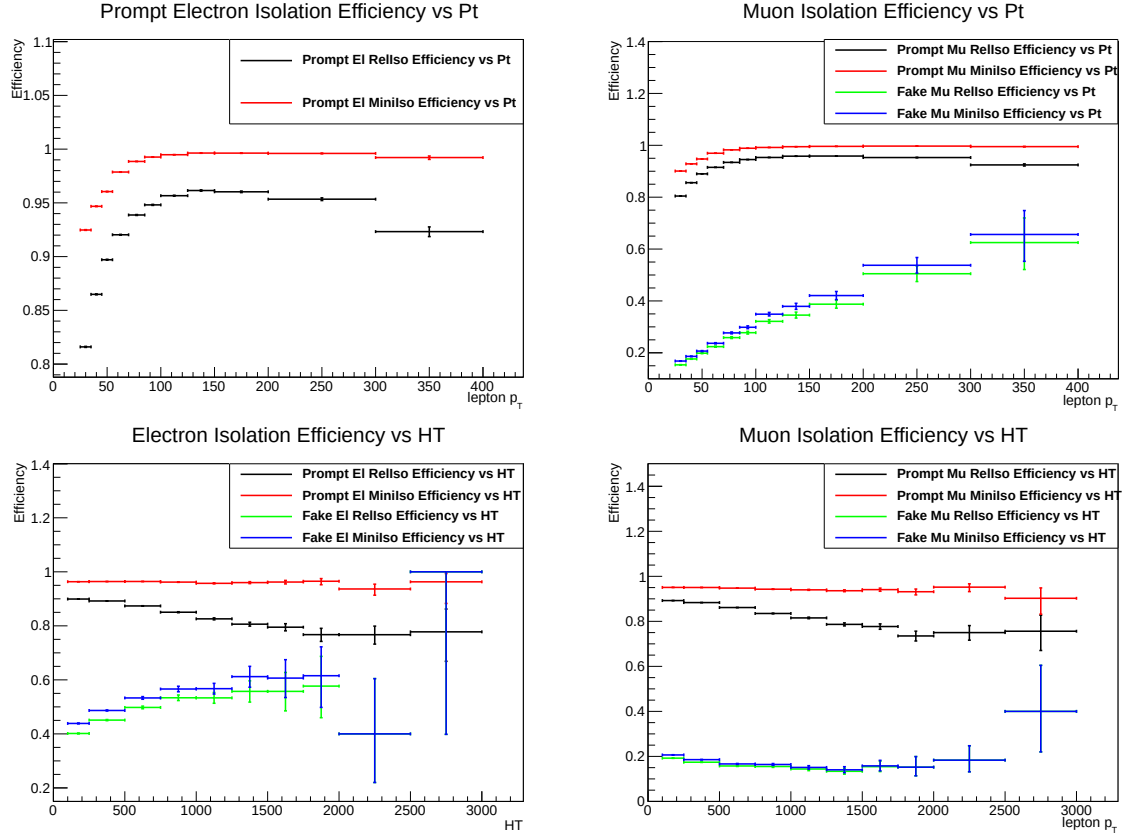
Fig. B.3: Isolation efficiency for t\bar{t} +jets events with upper requirements of I < 0.1 for both isolation types. Mini-isolation improves the efficiency of prompt leptons in general w.r.t. the fixed-cone isolation, and also remains efficient at high p_T and H_T .
