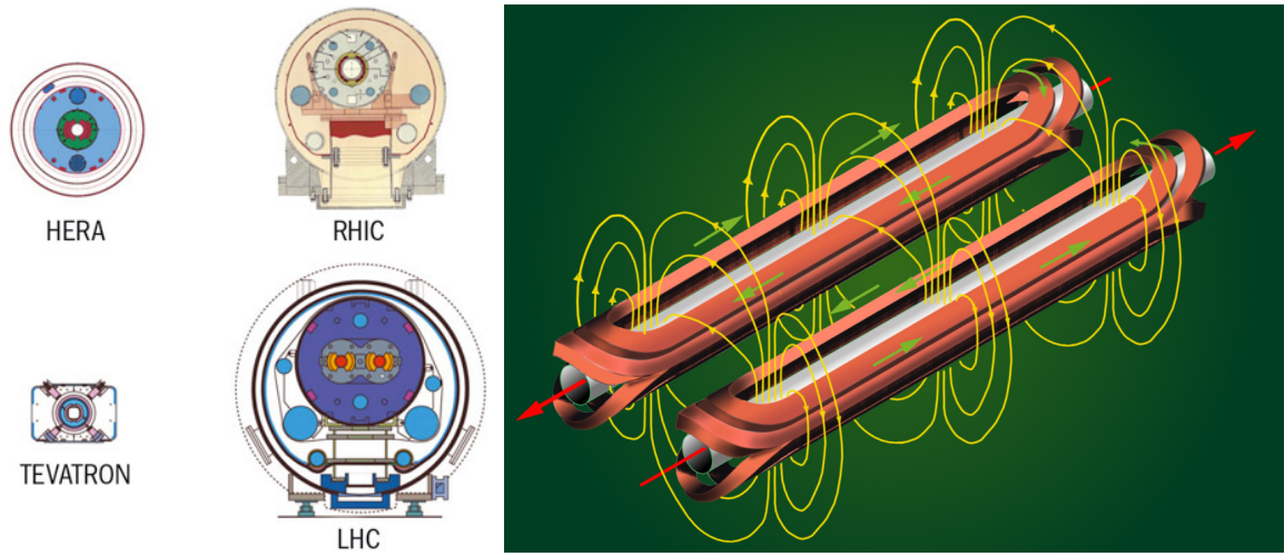
Fig. 2.1: Left : cross-section comparison of dipole magnets from the Tevatron to the LHC [62]. Right : schematic view of the two dipole coils of the LHC cryodipole [63]. The red arrows indicate the beam direction, the yellow show the magnetic field lines.
