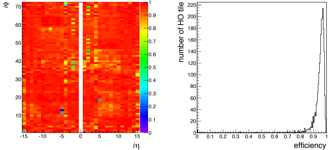
Fig. 3.19: Left : HO muon detection efficiency with a signal requirement above 45 ADC counts obtained from cosmic muons in global runs. The dashed regions correspond to not instrumented channels in the magnet chimney. Right : distribution of the efficiency for all HO channels. The median is 98.8%.
