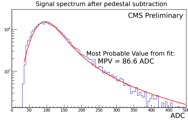
Fig. 3.7: Single channel signal spectrum with coincidence trigger. The fit with a Landau-Gaussian function is shown in red.
