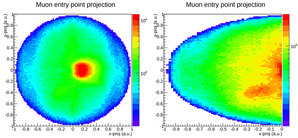
Fig. 3.12: Projections of the entry point for the global muons collected during the AGR ( left ). A zoom into the left half is shown on the right . The majority of tracks are coming vertically down, while also the effect of the access shafts is visible.
