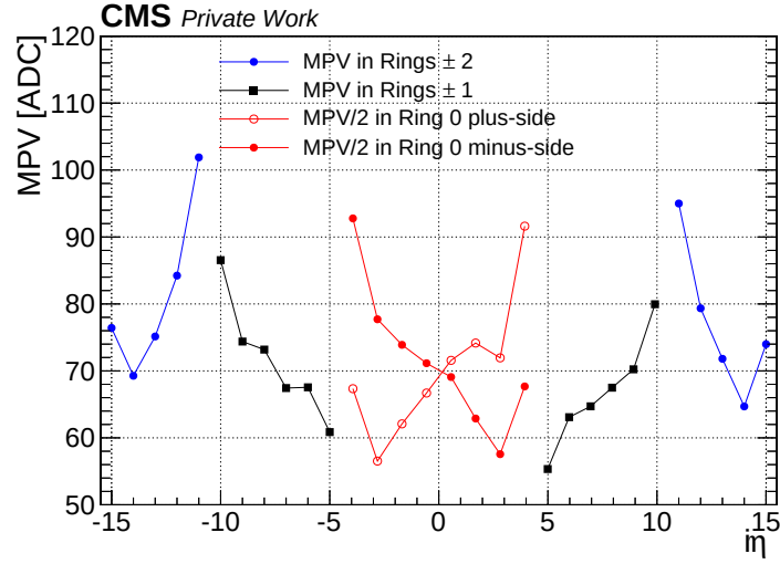
Fig. 3.18: Profile of the path-length corrected MPVs averaged over the i\phi axis in all HO tiles. For Ring 0 the values are divided by two because of the double layers. The highest signal corresponds to the position closest to the RBX.
