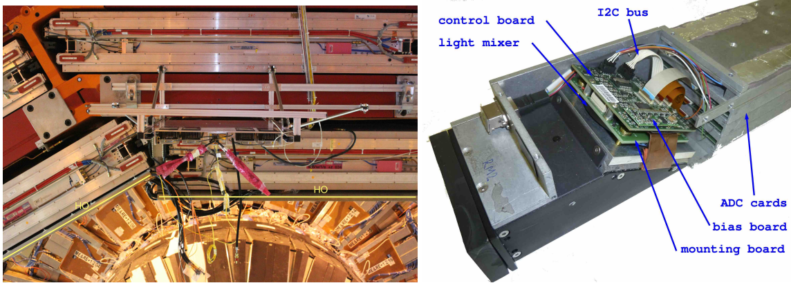
Fig. 3.2: Left : an HO readout box extracted from the barrel yoke. The black rectangles are the readout modules with the optical connectors. The scintillator planes of two sectors are indicated by yellow lines. Right : internal components of an HO readout module [109]. The SiPMs are fixed to the mounting board and coupled to the ODU with a light mixer.
