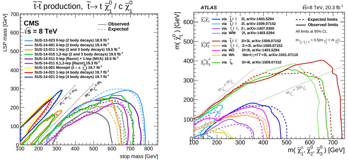
Fig. 1.5: Exclusion limits at 95% C.L. for searches of simplified pair production of stop quarks by CMS [49] (left) and different neutralinos or charginos by ATLAS [50] (right).
