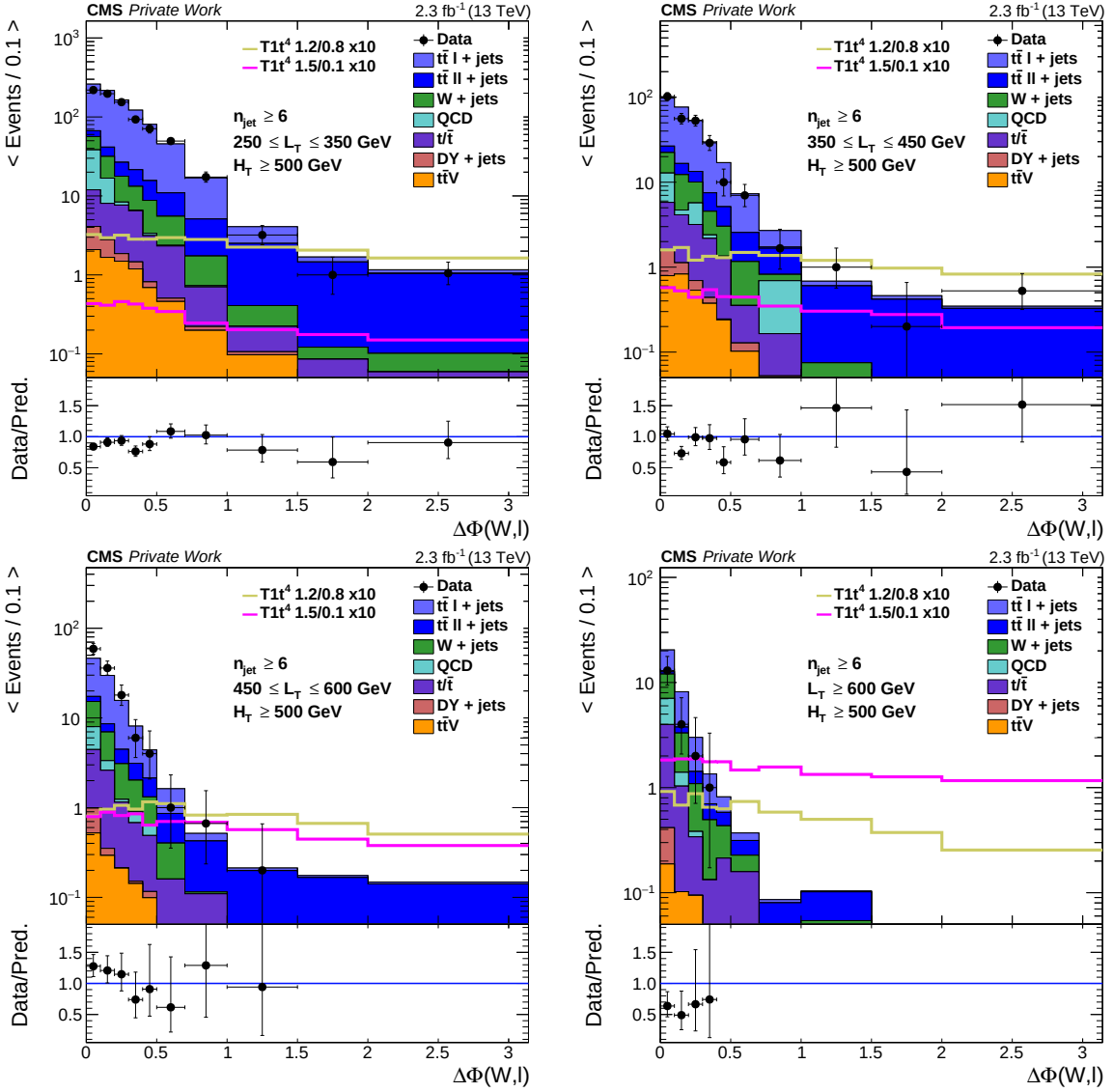
Fig. 7.2: \Delta\phi distributions in different L_T bins in data (black) and simulated samples after the baseline selection with n_{\text{jet}} \geq 6 , n_{\text{b-tag}} \geq 1 and H_T > 500 GeV. While the SM background samples are stacked on top of each other, the two signal benchmark points are scaled up by a factor of ten and drawn separately. The data-MC agreement is satisfactory throughout the \Delta\phi tails, and no significant excess is visible.
