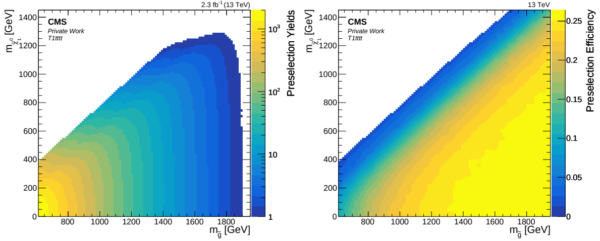
Fig. 5.11: T1tttt signal yields ( left ) and selection efficiency ( right ) after the baseline requirements. The missing mass points are interpolated from the existing yields.
