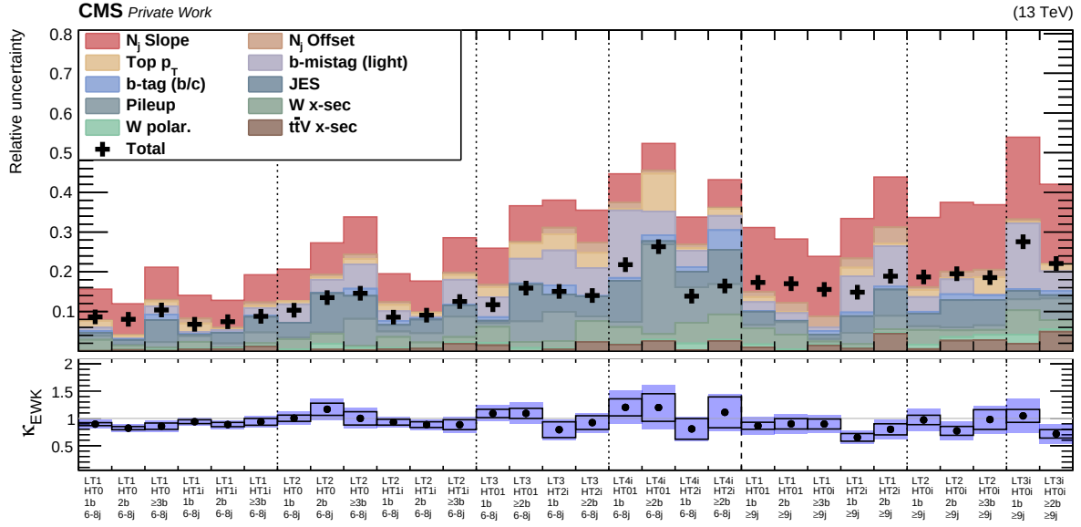
Fig. 6.25: Systematic uncertainties on the \kappa extrapolation for the simulated EWK background. Top : relative uncertainties for the individual sources stacked linearly on top of each other. The black crosses represent the total uncertainty. Bottom : nominal \kappa values with statistical uncertainties represented by the black box and the combined systematic and statistical uncertainties shown by the blue area.
