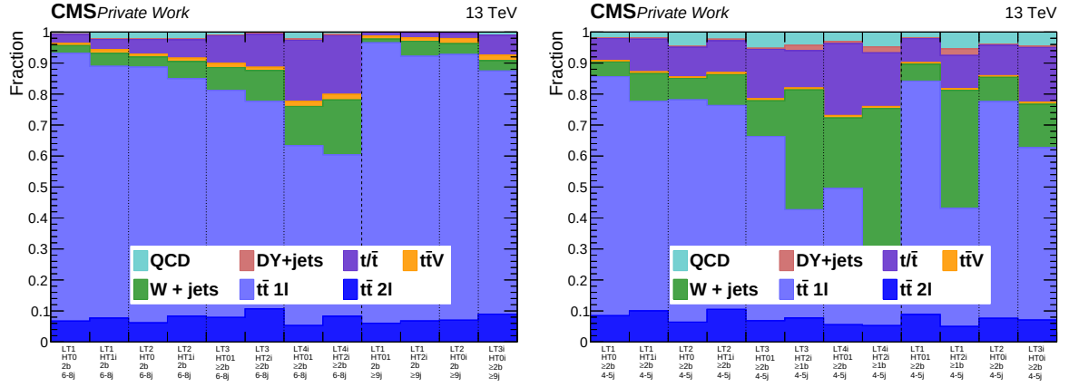
Fig. 6.8: Fractions of the SM backgrounds in the control regions of the mainband ( left ) bins with n_{b\text{-tag}} \geq 2 and corresponding sideband ( right ). The harder n_{b\text{-tag}} requirement further suppresses the W+jets contributions in both bands.
