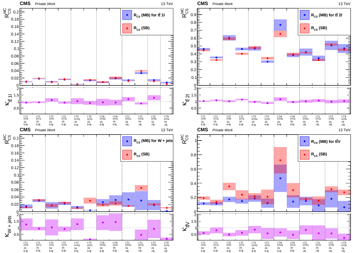
Fig. 6.7: R_{CS} in the SB and MB regions with n_{b\text{-tag}} \geq 1 , and \kappa values of the corresponding bins for the most important backgrounds. The individual R_{CS} of the t\bar{t} components and W +jets are similar between the n_{jet} bands, thus yielding a \kappa factor around one. The t\bar{t}V R_{CS} values resemble the one of combined t\bar{t} channels with a \kappa below one.
