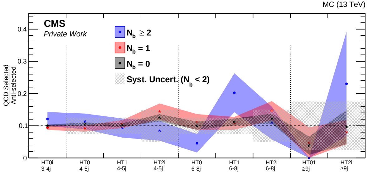
Fig. 6.18: F_{\text{sel-to-anti}} from simulated QCD event yields for different n_{\text{jet}} , H_T and n_{b\text{-tag}} bins with L_T > 250 GeV. The grey mesh is showing the chosen systematic uncertainties in the corresponding H_T and n_{\text{jet}} bins for n_{b\text{-tag}} < 2 . For higher b-jet multiplicities an uncertainty of 100% is assigned.
