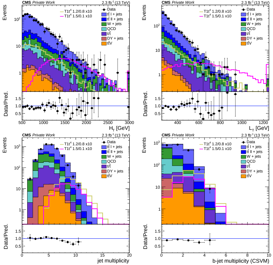
Fig. 5.8: Distributions of the H_T (left) and L_T (right) variables after the baseline selection in the top row. The bottom plots show the jet (left) and b-tag (right) multiplicities without the respective criteria applied besides the preselection. In the top plots the long tails of the non-compressed T1t^{ttt} (1500,100) signal distributions are visible, while the more compressed T1t^{ttt} (1200,800) scenario rather resembles the SM t\bar{t} process. The jet and b-tag multiplicities are independent of the gluino-neutralino mass splitting, and generally higher than of the background.
