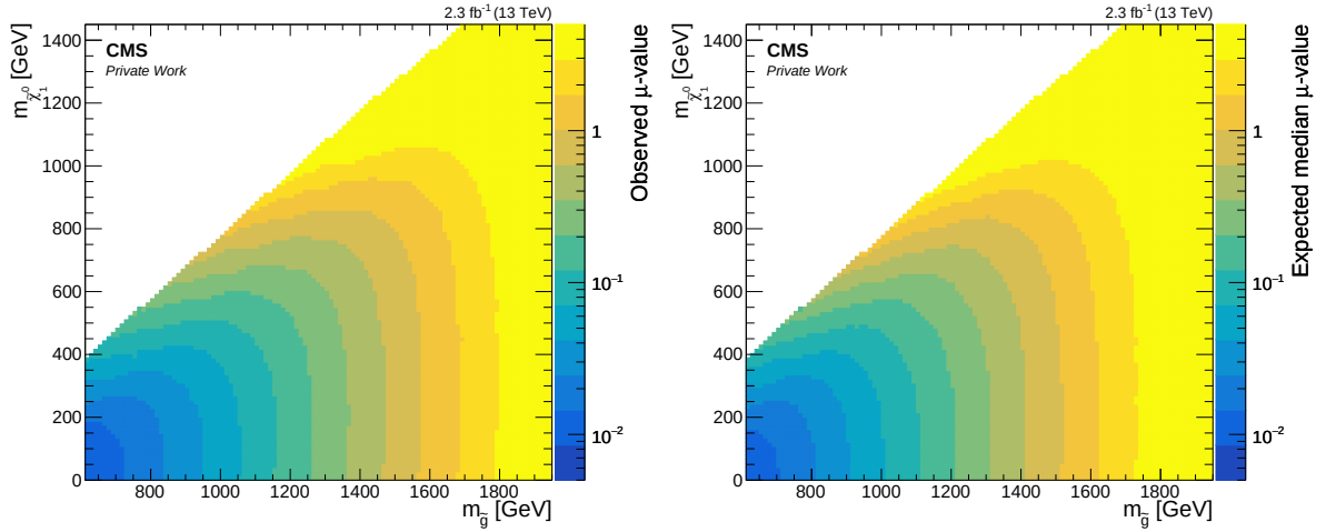
Fig. 7.5: 95% CL upper limits on the signal strength modifier \mu for the T1tttt model as observed (left) and for the median expected (right). The values for the missing mass scenarios are obtained from interpolating the adjacent results.
