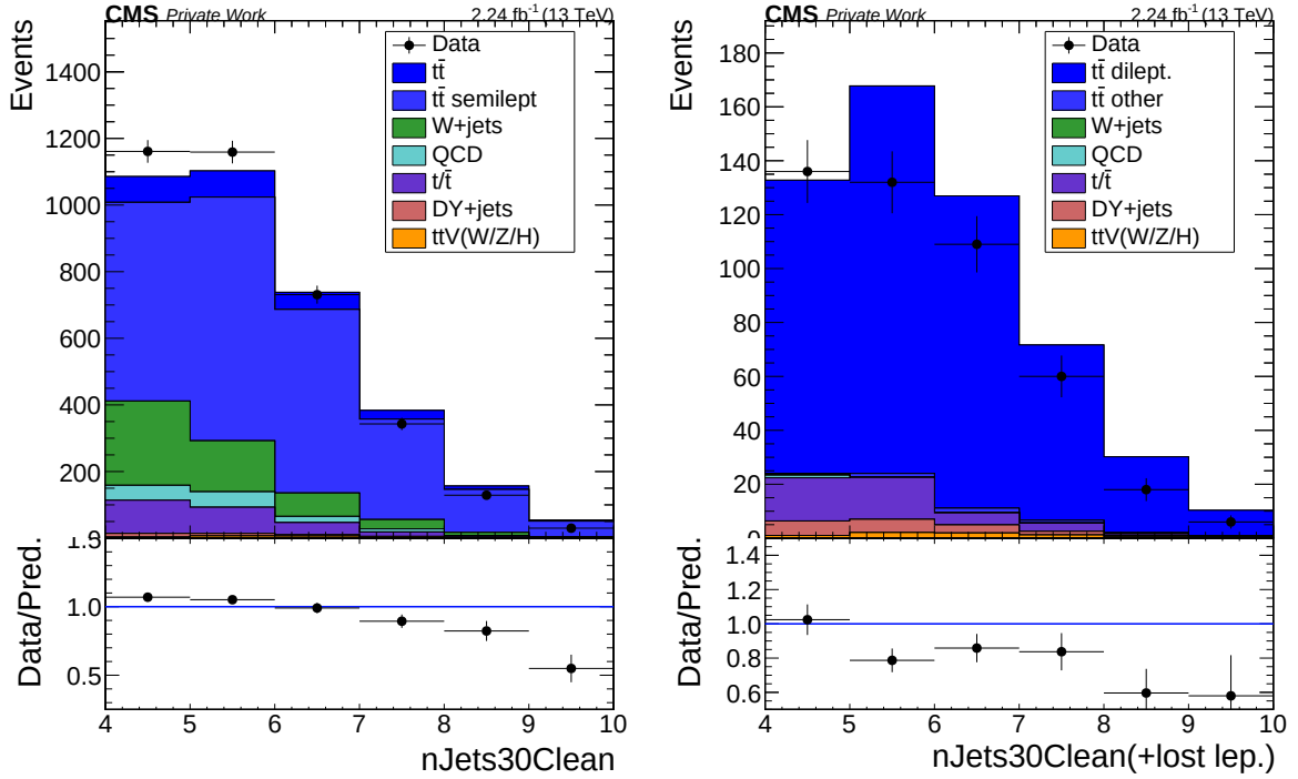
Fig. 6.4: Jet multiplicity distribution after the single-lepton baseline event selection with \Delta\phi < x (left) and in the dilepton control region (right), where one of the leptons is replaced with a \tau -decay like jet [159]. In both cases the simulation tends to overestimate the data towards high n_{\text{jet}} .
