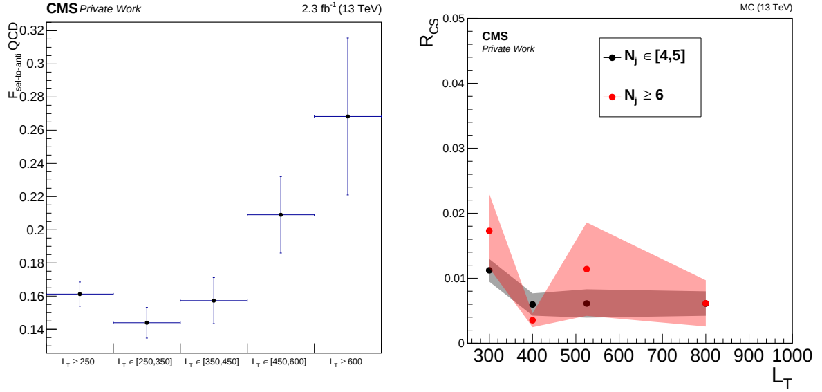
Fig. 6.21: Left: the corresponding ratio of selected to anti-selected events F_{\text{sel-to-anti}} in L_T bins. Right: R_{\text{CS}} values for anti-selected electron events in different L_T and n_{\text{b-tag}} bins for the n_{\text{jet}} = 4, 5 and \geq 6 in QCD MC.
