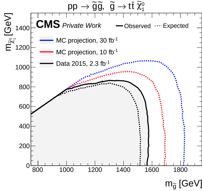
Fig. 7.7: T1tttt model exclusion limit for the current analysis with \mathcal{L} = 2.3 \text{ fb}^{-1} data (black) compared to the expected limits with 10 \text{ fb}^{-1} (red) and 30 \text{ fb}^{-1} (blue) based on simulation.
