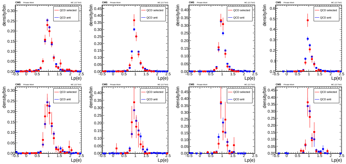
Fig. D.1: Shapes of L_p for selected and anti-selected QCD events in n_{\text{jet}} \in [3, 4] (top) and n_{\text{jet}} \geq 6 (bottom) for different L_T bins in simulation: [250, 350] , [350, 450] , [450, 600] and > 600 GeV.
