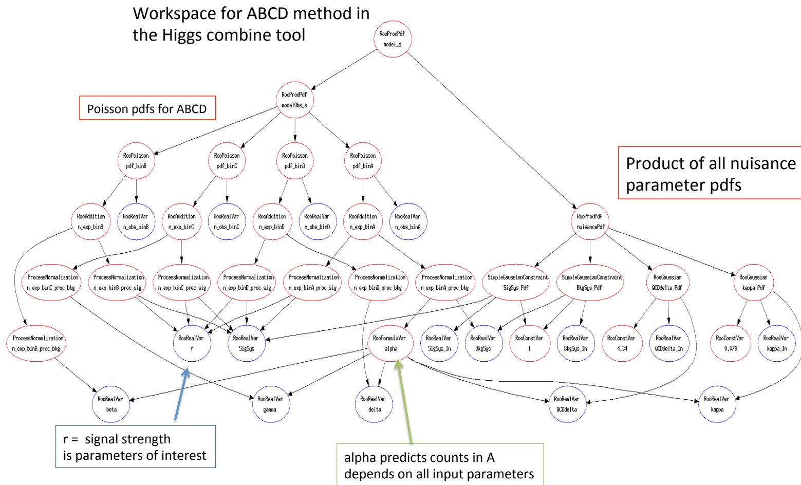
Fig. 7.4: Graphical representation of the likelihood implemented with an ABCD method for one bin in the Limit Tool [159].
