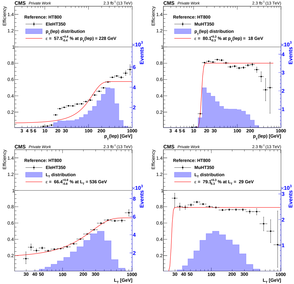
Fig. D.5: Measurement of the Lep15_IsoVVVL_PFHT350 trigger efficiency for the electron ( left ) and the muon ( right ) paths. The top plots show the turn-on of the leptonic leg, while the bottom show the turn-on of the hadronic leg. The number of events passing the trigger is given as shaded histogram.
