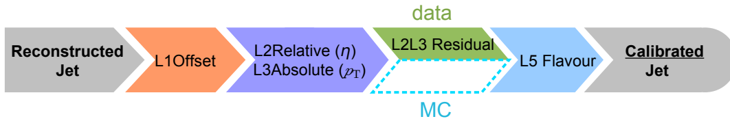
Fig. 4.6: Factorization of the CMS Jet Energy Calibration corrections. Except for the residual corrections, all factors are applied for data and simulated jets [144].
