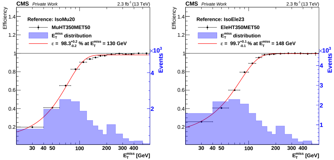
Fig. A.2: Efficiency of the E_T^{\text{miss}} leg for the backup HLT paths including an isolated muon (left) or electron (right). The reference selection requires the events to pass an isolated lepton trigger, contain a single lepton with p_T > 25 GeV and satisfy H_T > 500 GeV.
