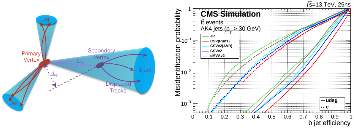
Fig. 4.8: Left : transverse view of an event containing two jets from the PV, and a b-jet composed of tracks originating from a secondary vertex. The SV is displaced by L_{xy} , and the transverse impact parameter d_{xy} is shown for a single displaced track. Right : performance of the CMS b-jet identification algorithms 4 ; the fraction of correctly identified b-jets (efficiency) is shown versus the probability to accept a non-b jet (misidentification). CSVv2, shown in blue, corresponds to the tagger used in the present analysis; the other algorithms are described elsewhere [141].
