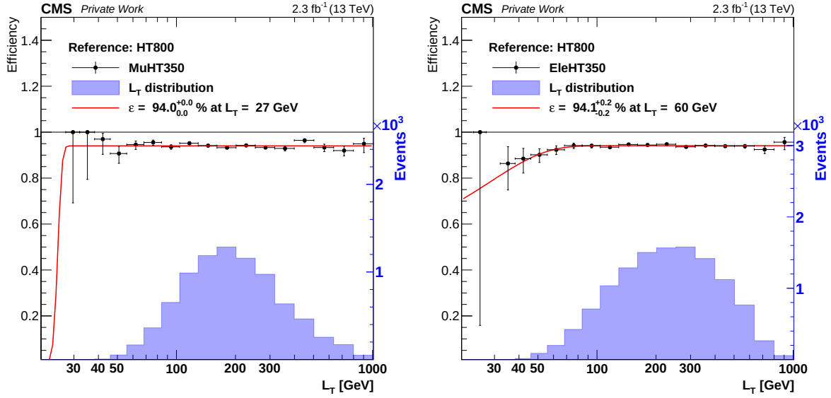
Fig. 5.5: Event selection efficiency as a function of the L_T variable for the analysis HLT paths including a muon HLT_Mu15_IsoVVVL_PFHT350 (left) or an electron HLT_Ele15_IsoVVVL_PFHT350 (right). The baseline selection requires the events to pass a pure H_T trigger HLT_PFHT800 and contain a single good lepton with p_T > 25 GeV. The number of events passing the triggers is shown in the blue histograms.
