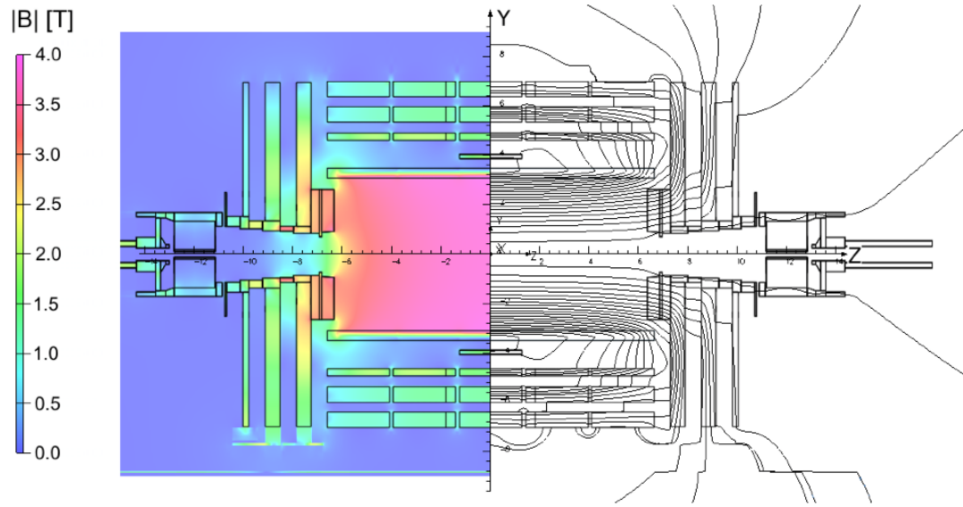
Fig. 2.5: Magnetic field strength (left) and field lines (right) in a longitudinal section of CMS as predicted at a central magnetic flux density of 3.8 T. The magnetic flux changes between the lines by 6 Wb. From Ref. [80].
