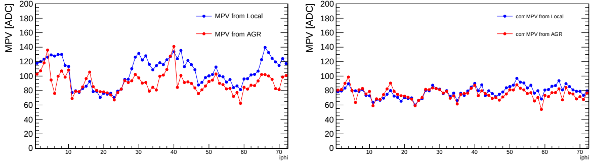
Fig. 3.16: Comparison of averaged MPV profiles from the local and global calibrations in Rings\pm 1,2 . The values for the uncorrected signal ( Left ) are similar only in the horizontal sectors, where the trigger acceptances are similar. After the path-length correction ( Right ) the overall agreement is improved over the whole i\phi range.
