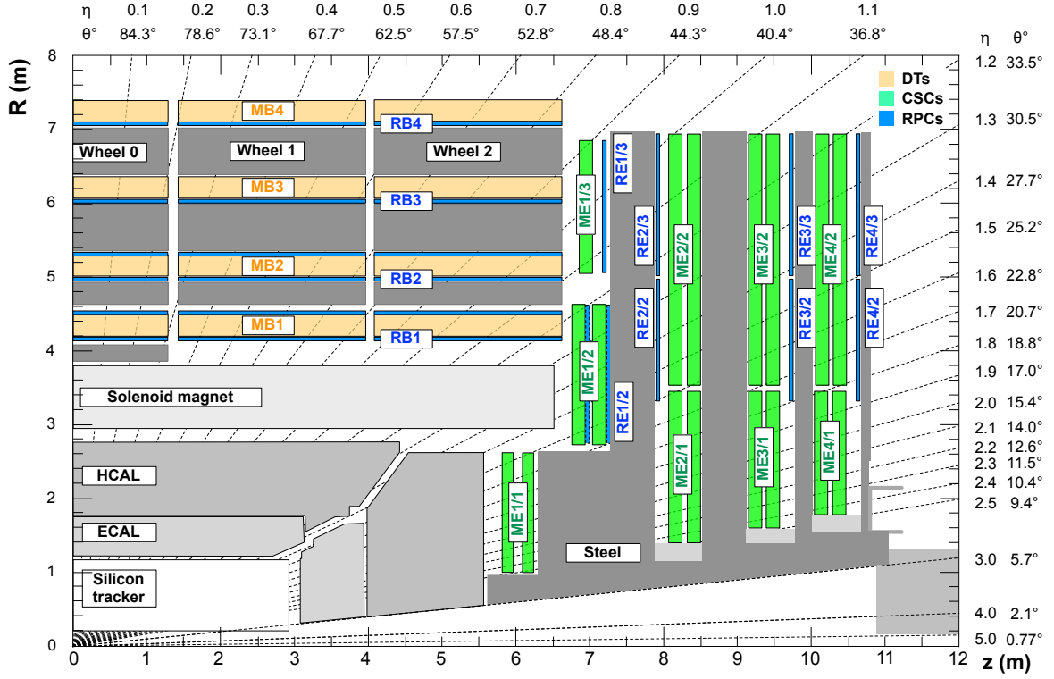
Fig. 2.10: Layout of a quadrant of the CMS Muon system after the LS1 [90]. The barrel wheels host the DT and RPC chambers in four stations parallel to the beam-pipe. Another four stations of CSC and RPC provide coverage in the endcaps.
