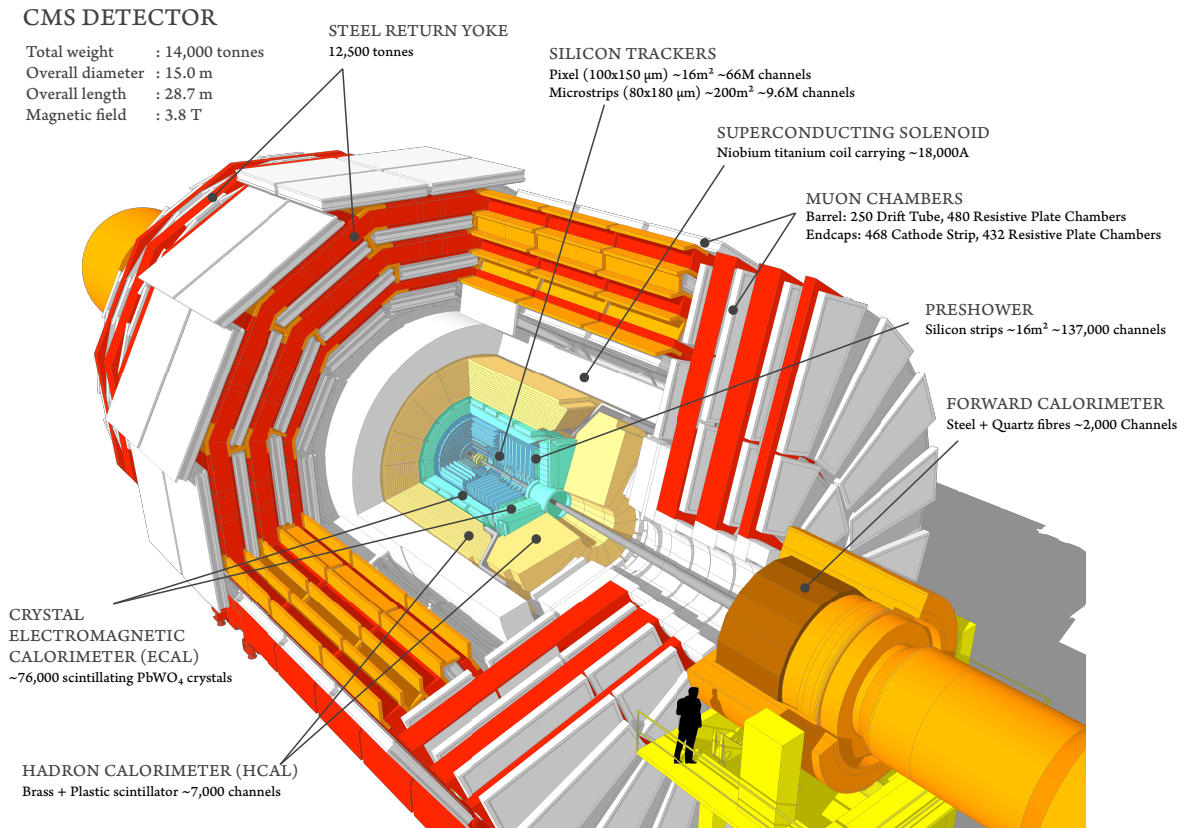
Fig. 2.4: Schematic view of the CMS detector with a cut-out quadrant [79]. The individual sub-detectors are shown with some highlights pointed out.
