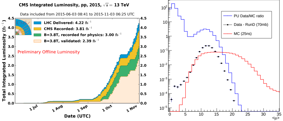
Fig. 5.2: Left : Cumulative integrated luminosity delivered to (blue), and recorded by CMS (orange) during pp-collisions at a centre-of-mass energy of 13 TeV in 2015 [149]. The green histogram shows the amount of data collected at the full magnetic field, while the fraction of data validated by the DQM experts is indicated in beige.
