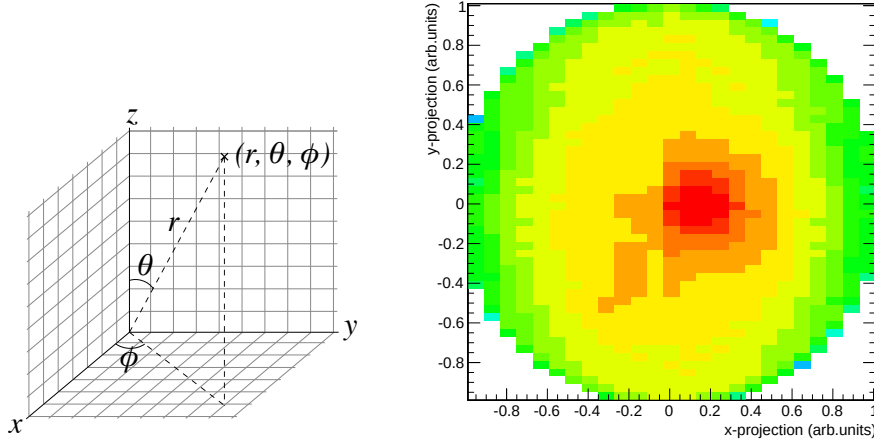
Fig. 3.9: Left : Coordinate system used for cosmic muons. For the entry point validation the track length is assumed one [116]. Right : Projection of the HO track entry points. Most tracks hit the center of the detector, while a slight shift towards the access shaft is seen. Another hot spot caused by the secondary shaft is seen at x \approx -0.2, y \approx -0.4 .
