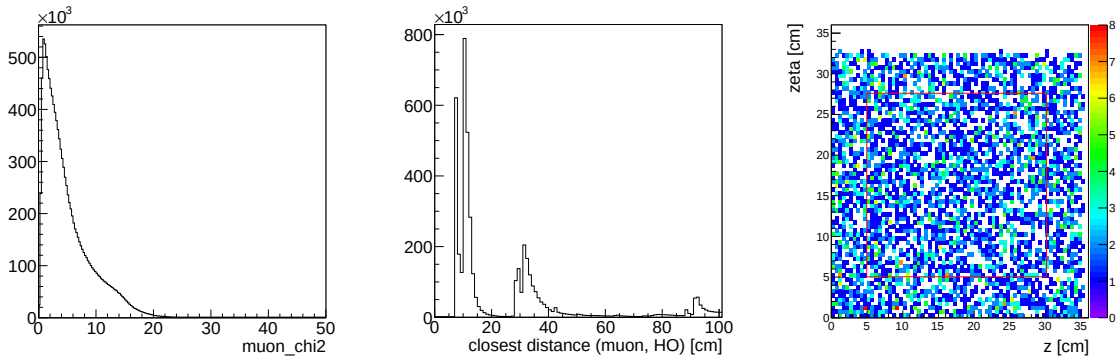
Fig. 3.13: Muon variables used for the selection of global run events. From left to right : muon \chi^2/\text{n.d.f} , \Delta R (closest muon station hit, HO hit position), and the HO tile hit map with the selection border indicated in red. In the middle plot, the first peak corresponds to the HO layer close to the first muon station, while the second peak arises from hits into the inner HO layer in Ring 0 which is farther away from the DT station.
