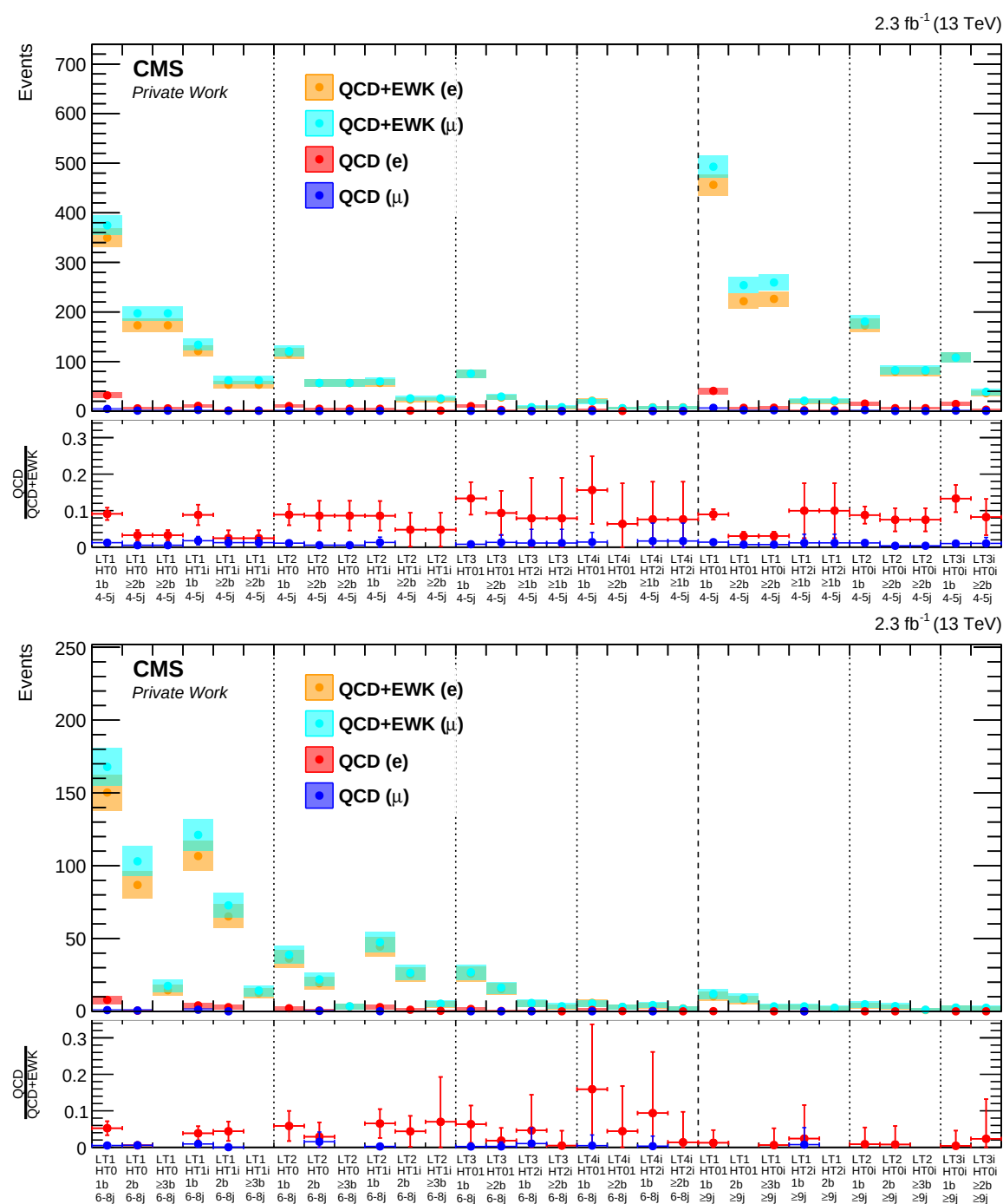
Fig. 6.13: Comparison of the simulated total background and QCD-only yields for electron and muon events in the sideband ( top ) and mainband ( bottom ) control regions. The error bars indicate the expected statistical uncertainty as for Poissonian distributed data. The bottom panels show the fraction of the QCD events relative to the total SM (i.e. QCD and EWK) background.
