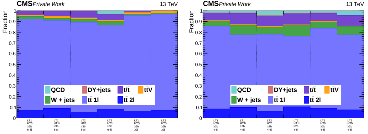
Fig. 6.10: Fractions of the SM backgrounds in the control regions of the mainband ( left ) bins with n_{b\text{-tag}} \geq 3 and corresponding sideband ( right ). Both bands are dominated by t\bar{t} +jets events at around 90%.
