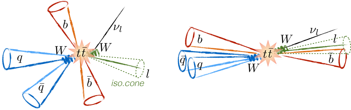
Fig. 4.4: Topology of a t\bar{t} event in case of low (left) and high (right) boost, where the isolation cone of the lepton can overlap with other decay products [137].
