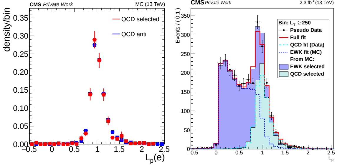
Fig. 6.15: Left : Comparison of normalized L_p shapes for simulated selected (red) and anti-selected (blue) electron events after the baseline selection with modified requirements of n_{\text{jet}} \in [3, 4] and zero b-tags. Right : L_p shape fit for pseudo-data after the same selection as on the left . The simulated distributions of EWK and QCD events for the given luminosity are shown by the shaded histograms, which, combined, serve as a template for the pseudo-data (black) generation. The EWK shape (blue dashed) is taken from the same selected events, while the QCD template (cyan dashed-dotted) is obtained from the anti-selected sample.
