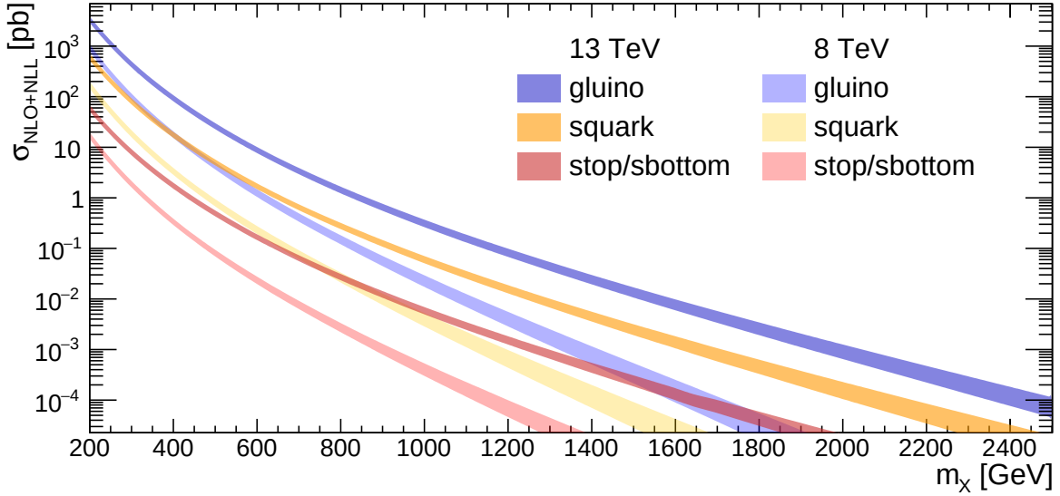
Fig. 1.6: SUSY particle pair production cross-sections for different masses of gluinos, squarks and stops/sbottoms in proton collisions at \sqrt{s} = 8 and 13 TeV. Based on Refs. [52–55].
