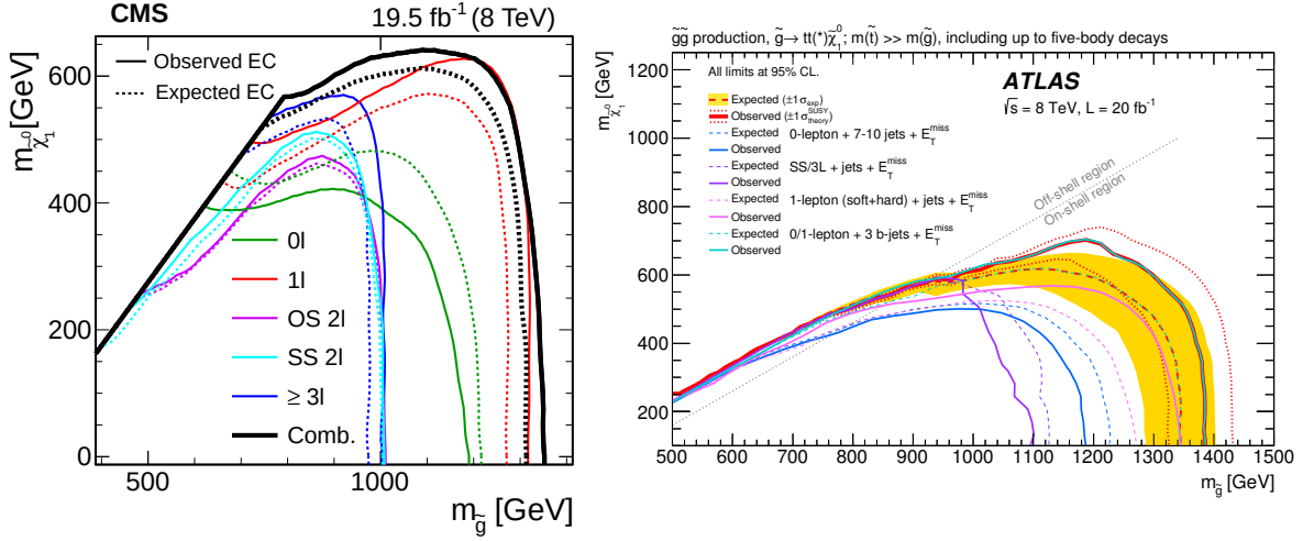
Fig. 1.4: Exclusion contours at 95% C.L. in the gluino-neutralino mass plane of \sqrt{s} = 8 TeV analyses of CMS [45] (left) and ATLAS [46] (right) searching for simplified gluino pair production with subsequent decays to t\bar{t} and a neutralino, which is the LSP.
