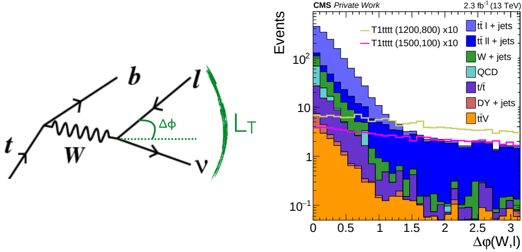
Fig. 5.9: Left : topology of a top quark and subsequent leptonic W -boson decay. \Delta\phi shows the azimuthal angle between the reconstructed boson and lepton. L_T is the scalar sum of the missing energy from the neutrino and the lepton p_T . Right : distribution of the \Delta\phi variable after the baseline selection. Due to the large and not lepton-aligned \cancel{E}_T , SUSY events give a flat \Delta\phi distribution. The filled histograms of the SM backgrounds are stacked on top of each other, and the signal benchmarks scaled by ten are shown in the solid lines.
