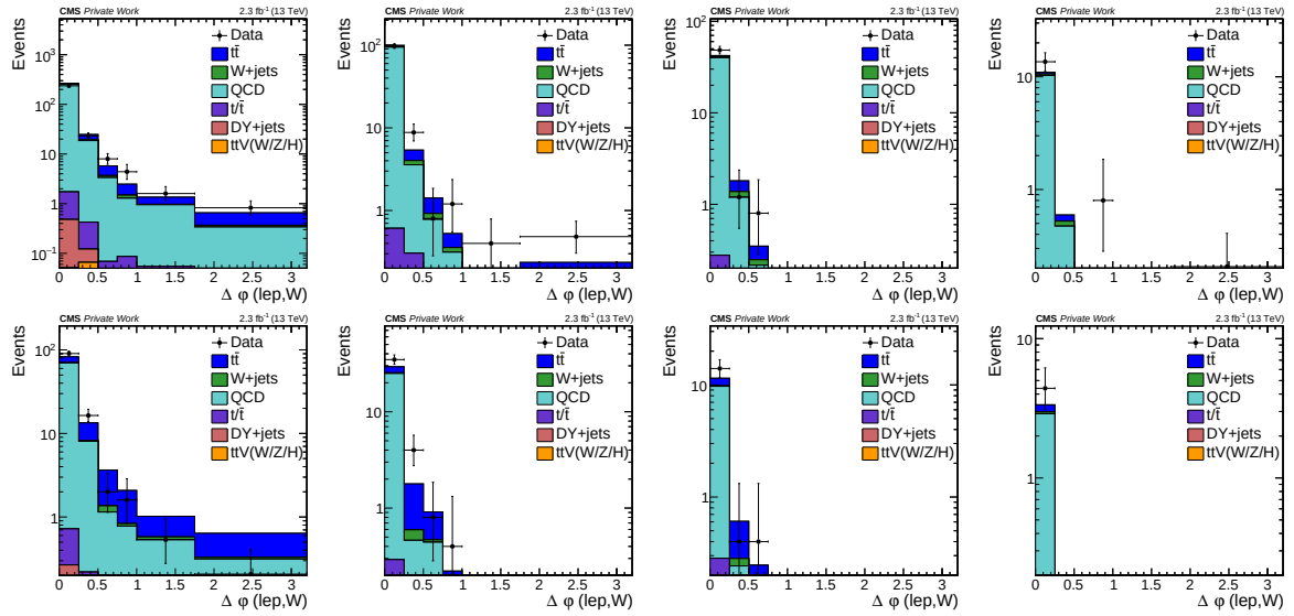
Fig. D.3: \Delta\phi for anti-selected events in data compared to simulation for n_{\text{jet}} = 4, 5 (top) and n_{\text{jet}} = 6-8 (bottom) for different L_T bins with n_{b\text{-tag}} \geq 1 : [250, 350] , [350, 450] , [450, 600] and > 600 GeV. The content is normalized to the bin width.
