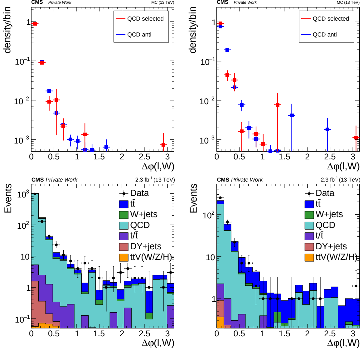
Fig. 6.22: Top : normalized \Delta\phi distributions for selected and anti-selected electron QCD events for n_{\text{jet}} \in [3, 4] (left) and n_{\text{jet}} \geq 6 (right) after the baseline selection with L_T > 250 GeV and H_T > 500 GeV. The agreement in shapes indicates a similar R_{\text{CS}} transfer factor for both samples. Bottom : distribution of \Delta\phi for anti-selected electrons in data for n_{\text{jet}} \in [3, 4] (left) and n_{\text{jet}} \geq 6 (right) compared to the simulated backgrounds. The sample is mostly dominated by QCD events, and the good dataMC agreement allows to use the simulated R_{\text{CS}} factor for data as well.
