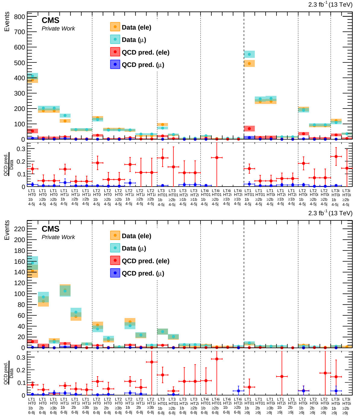
Fig. 6.24: Comparison of yields for selected electrons and muons with the data-driven QCD predictions in the sideband ( top ) and mainband ( bottom ) control regions. The average estimated contributions from the electron channel at about 10%, and in the muon channel at the percent level, agree with the expectation from simulation.
