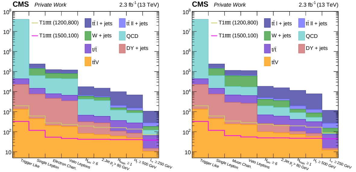
Fig. 5.7: Number of events for each sample, scaled to the luminosity by the respective cross section, after each requirement step of the baseline selection in the electron (left) and muon (right) channel. While the SM backgrounds get substantially suppressed, the two signal benchmark scenarios loose only a fraction of events.
