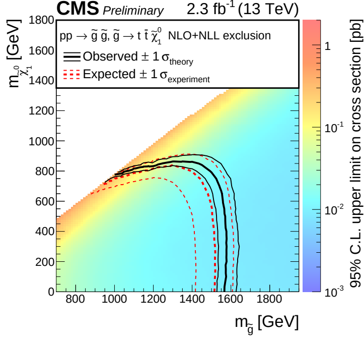
Fig. 7.6: 95% C.L. cross section limits for the T1tttt model as obtained using the \text{CL}_s criterion. The observed contour for the nominal theory cross section is shown in black, complemented with the exclusions originating from the corresponding theory uncertainty. In red (dashed) the expected exclusion contours are shown for the median and \pm 1\sigma error bands corresponding respectively to the 50%, 16% and 84% quantiles of the \mu^{95\% \text{CL}} distribution.
