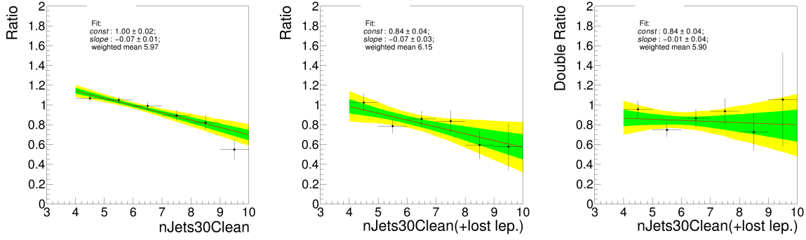
Fig. 6.5: Ratio of data and simulated events for the jet multiplicity distribution of single lepton events ( left ), dileptonic events ( middle ), and the resulting double ratio (dileptonic/semileptonic; right ) [159]. The ratios are fitted with a linear parametrisation and the fit parameters are indicated in the plots.
