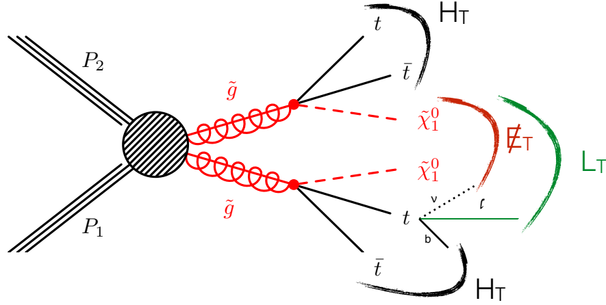
Fig. 5.1: Illustration of gluino pair production and decay within the T1tttt model. The energy scale of the event is characterized by: the multitude of jets creating a large hadronic energy H_T , while the missing transverse energy \cancel{E}_T from the neutrino and neutralinos add up with the lepton momentum into the leptonic energy scale L_T .
