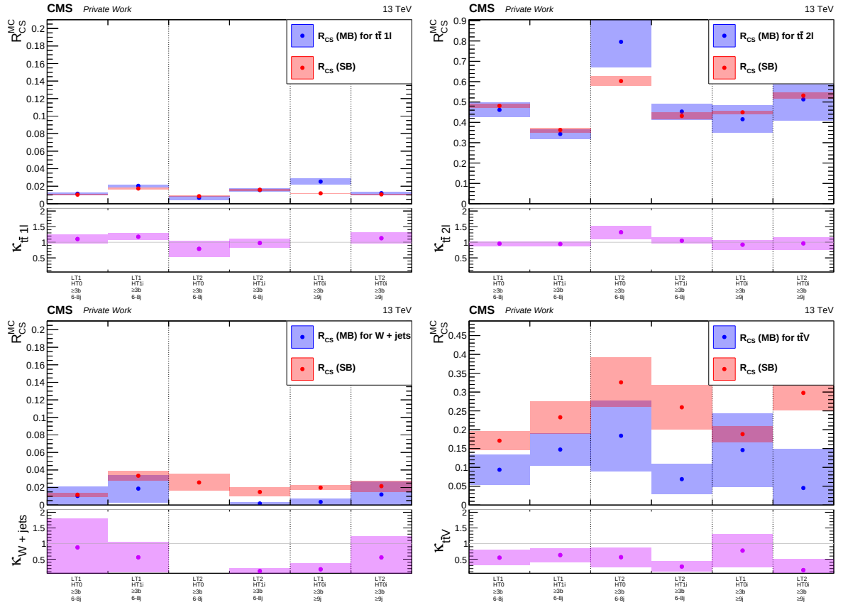
Fig. 6.11: R_{CS} in the SB and MB regions with n_{b\text{-tag}} \geq 3 , and \kappa values of the corresponding bins for the most important backgrounds. Similar to the n_{b\text{-tag}} \geq 2 behaviour except for increased statistical fluctuations due to a harder n_{b\text{-tag}} requirement in the mainband.
