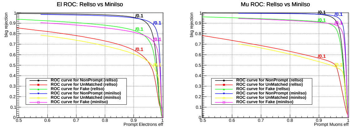
Fig. B.3: Isolation efficiency for t\bar{t} +jets events with upper requirements of I < 0.1 for both isolation types. Mini-isolation improves the efficiency of prompt leptons in general w.r.t. the fixed-cone isolation, and also remains efficient at high p_T and H_T .
