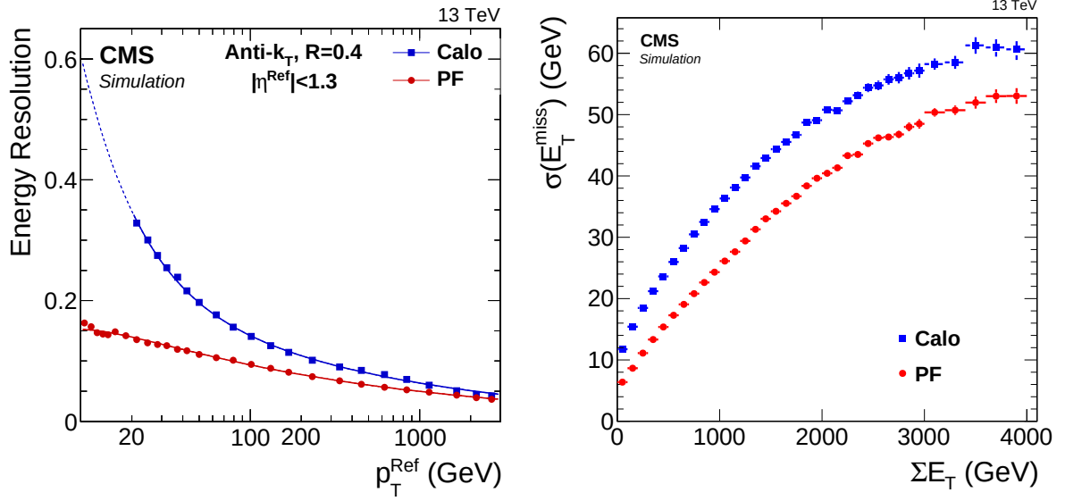
Fig. 4.7: Resolutions of the jet transverse momentum ( left ) and absolute missing transverse energy ( right ) [122]. E_T is the transverse energy sum of all objects that enter the calculation of \cancel{E}_T . The red lines indicate the resolutions for the particle-flow objects, while the blue ones correspond to jets and \cancel{E}_T reconstructed using only the information from the calorimeters [145]. The PF quantities have systematically better energy resolutions.
