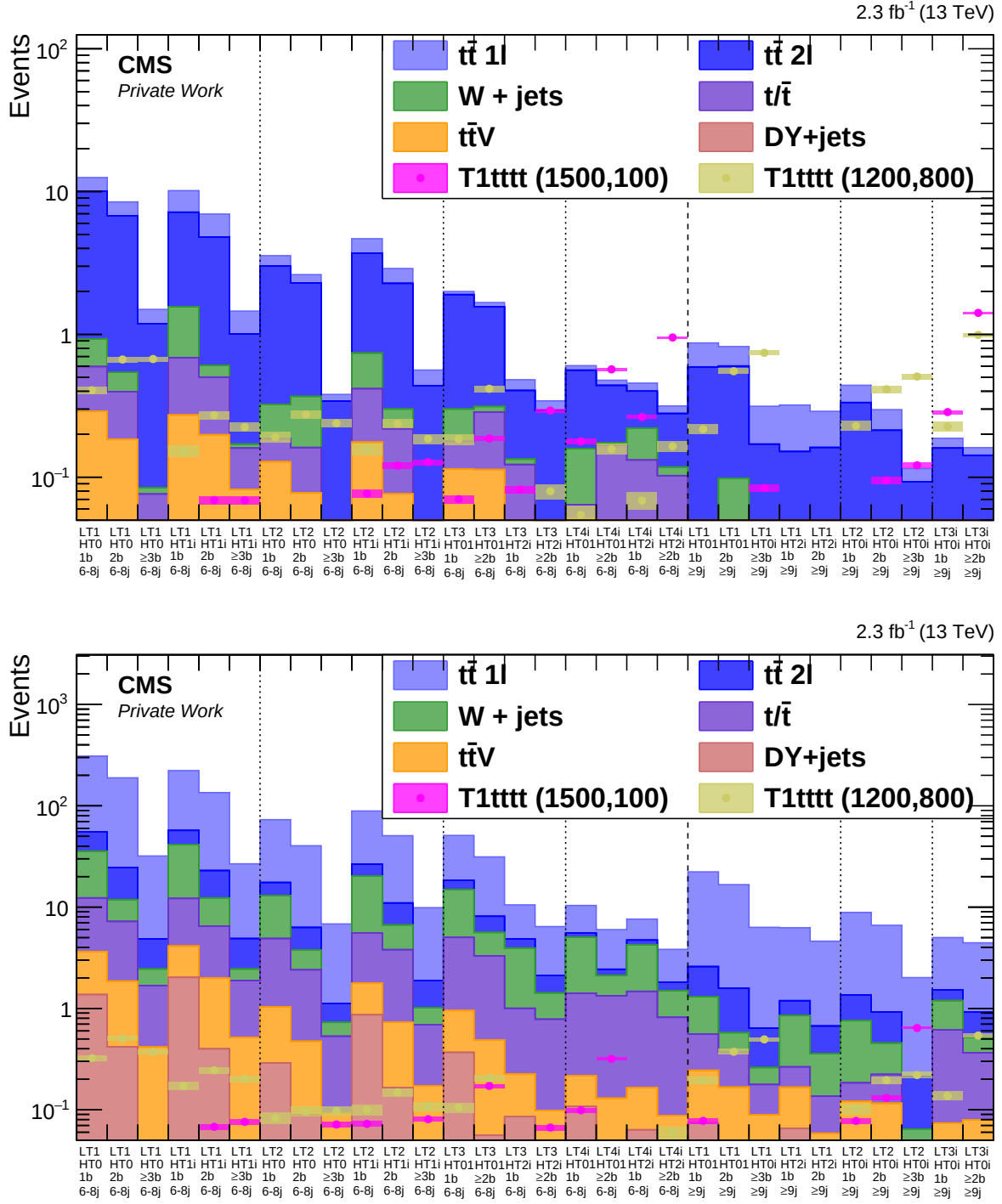
Fig. 5.13: Simulated event yields for the EWK backgrounds and two signal benchmark models in all 30 search categories for the signal ( top ) and control ( bottom ) regions. The non-compressed T1tttt (1500,100) signal mostly populates the bins with large L_T , while the compressed T1tttt (1200,800) scenario contribution is spread over the whole search phase-space. The signal contamination in the control regions is always less than one event, and hence negligible.
