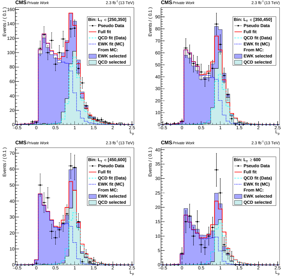
Fig. D.4: Fit results in the zero b-tag bin with n_{\text{jet}} = 3,4 for all four L_T bins. The black dots represent the pseudo-data obtained from the template of EWK and QCD selected events, which are shown with the blue and green dashed histograms. The full fit result is shown with the solid red line, while the separate EWK and QCD components are depicted by the blue and green dashed lines, respectively.
