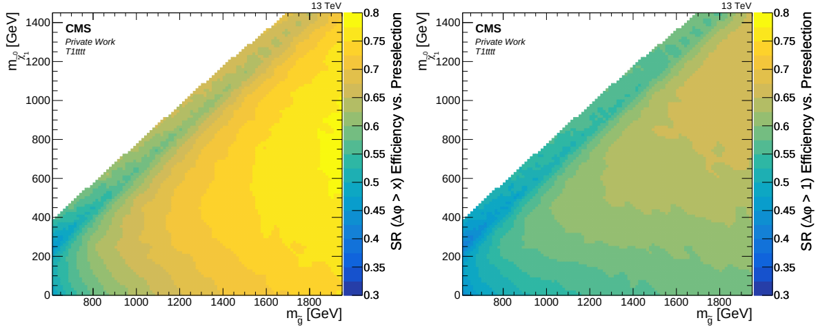
Fig. 5.12: Signal region selection efficiency with respect to the preselection for the L_T -dependent \Delta\phi threshold x ( left ) and constant \Delta\phi > 1 ( right ) for the T1tttt model. The control region efficiencies are respectively inverse.
