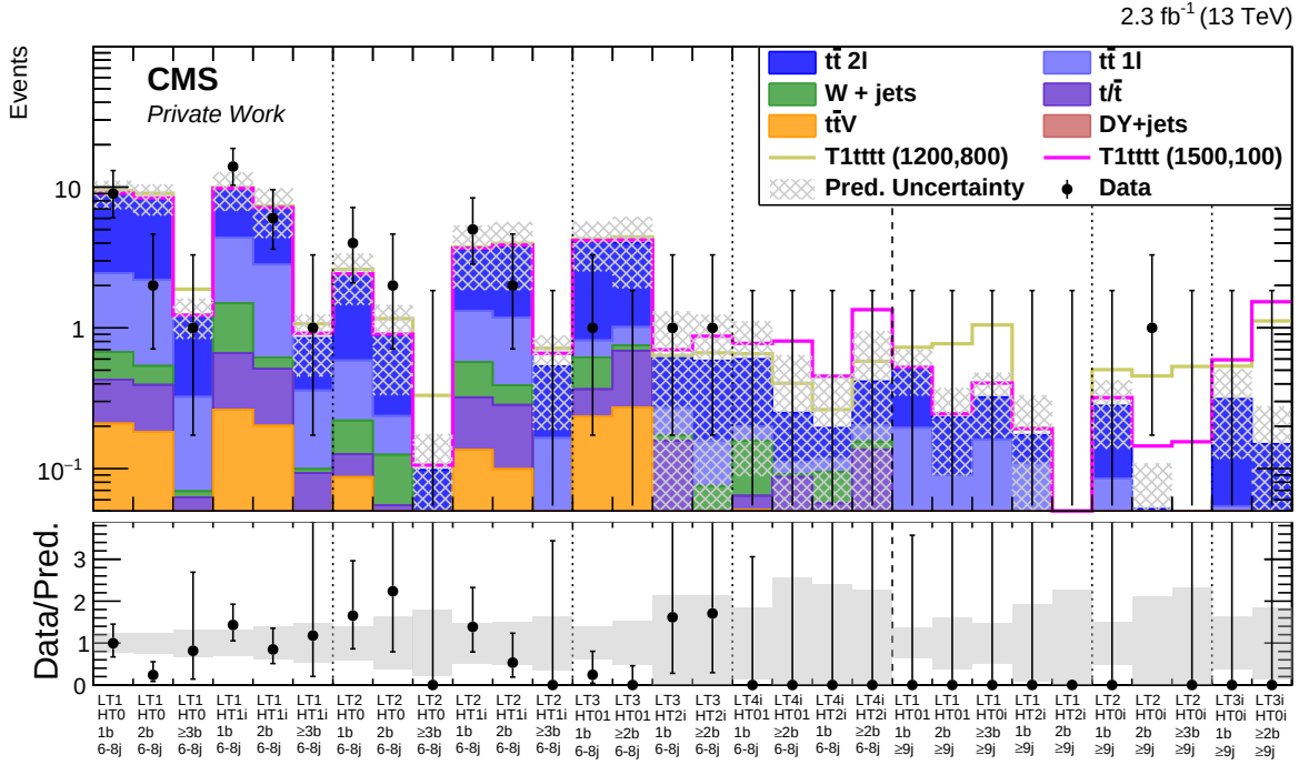
Fig. 7.1: Observed and predicted event yields in the 30 search regions. The black points show the number of events observed in data. The data-driven prediction of the SM background is represented by the filled histograms, preserving the individual contributions from simulation. The coloured lines illustrate the expectations for two benchmark scenarios of the T1tttt model, which are stacked on top of the data prediction. The lower panel shows the ratio of data to the prediction, where the error bars indicate the total statistical and systematic uncertainty on the ratio and the grey band shows the prediction uncertainty.
