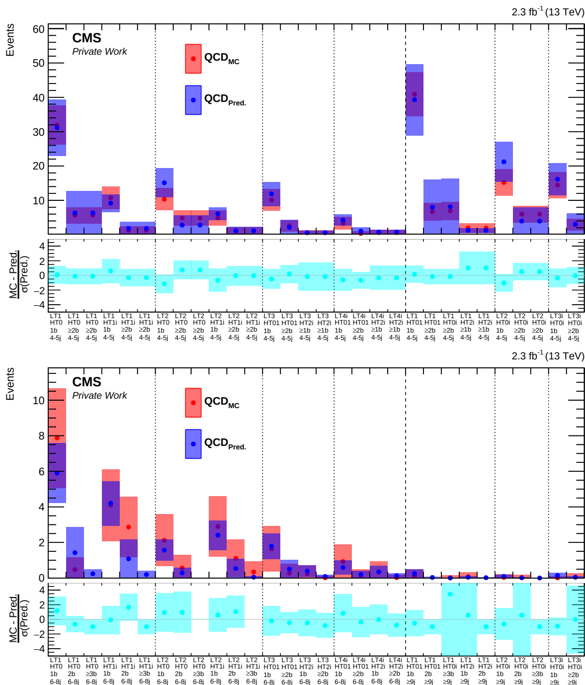
Fig. 6.19: Comparison of the number of selected QCD events in the control region as expected from simulation (red) with predicted yields estimated from the anti-selected sample for electrons. The F_{\text{sel-to-anti}} is obtained in bins of L_T from simulation, and a systematic uncertainty is added as explained in the text. For the sideband ( top ) the agreement is better than for the corresponding mainband bins ( bottom ), due to higher statistics and negligible contribution from EWK events in the anti-selected sample.
