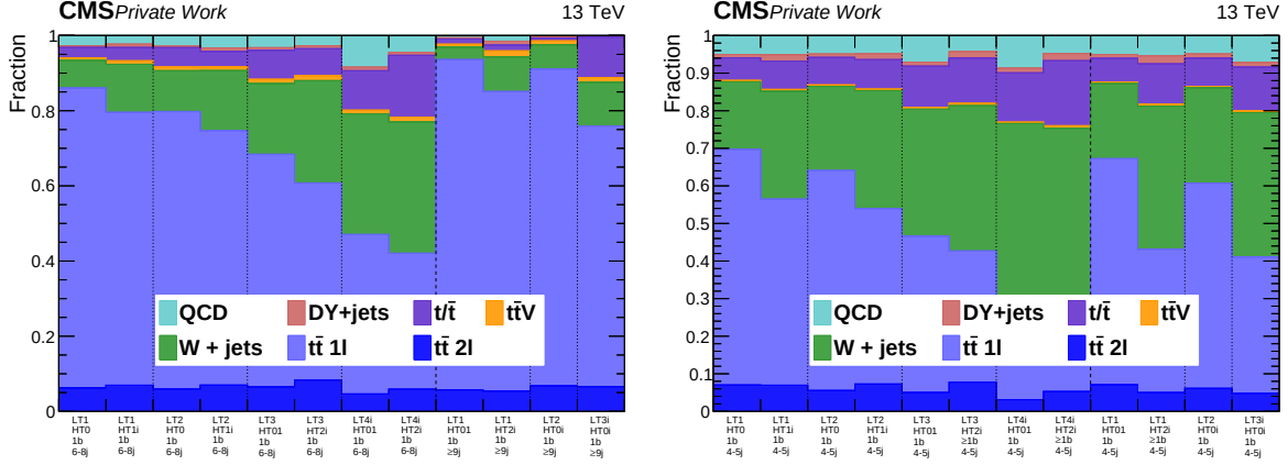
Fig. 6.6: Fractions of the SM backgrounds in the control regions of the mainband ( left ) bins with n_{b\text{-tag}} = 1 and corresponding sideband ( right ). While the MB is dominated by t\bar{t} , the SB has also a similar contribution from W +jets.
