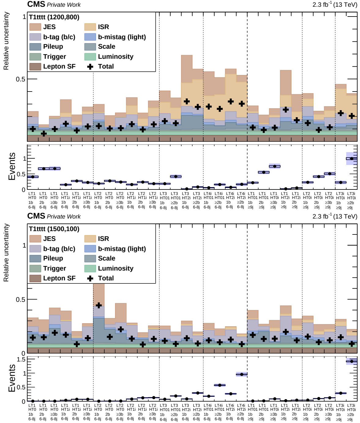
Fig. 6.26: Systematic uncertainties on the signal yields for the T1tttt(1200,800) ( top ) and T1tttt(1500,100) ( bottom ) signal points. While the non-compressed scenario shows an overall flat total uncertainty of about 15%, the compressed scenario suffers from the increased ISR uncertainty in the high L_T bins increasing the total up to 30%. The top part of the plot shows the relative uncertainty on the nominal yield for the different sources of uncertainties. The various uncertainties are stacked linearly on top of each other, while the black crosses represent the total. The bottom plot shows the nominal signal yields with the statistical uncertainty represented by the black box and the combined systematic and statistical uncertainties shown by the blue area.
