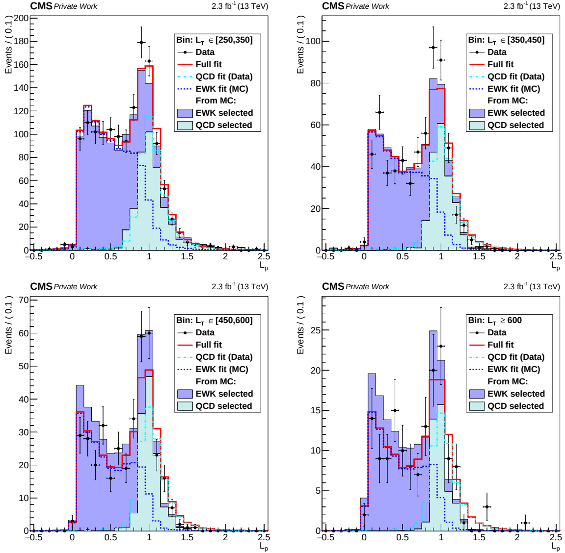
Fig. 6.20: L_p shape fit results in the data with n_{b\text{-tag}} = 0 , n_{\text{jet}} \in [3, 4] for different L_T ranges. The black dots represent data. EWK and QCD selected events from simulation normalized to the luminosity are shown with the blue and cyan filled histograms. The full fit result is shown with the red solid line, while the separate EWK and QCD components are depicted by the blue and cyan dashed lines, respectively.
