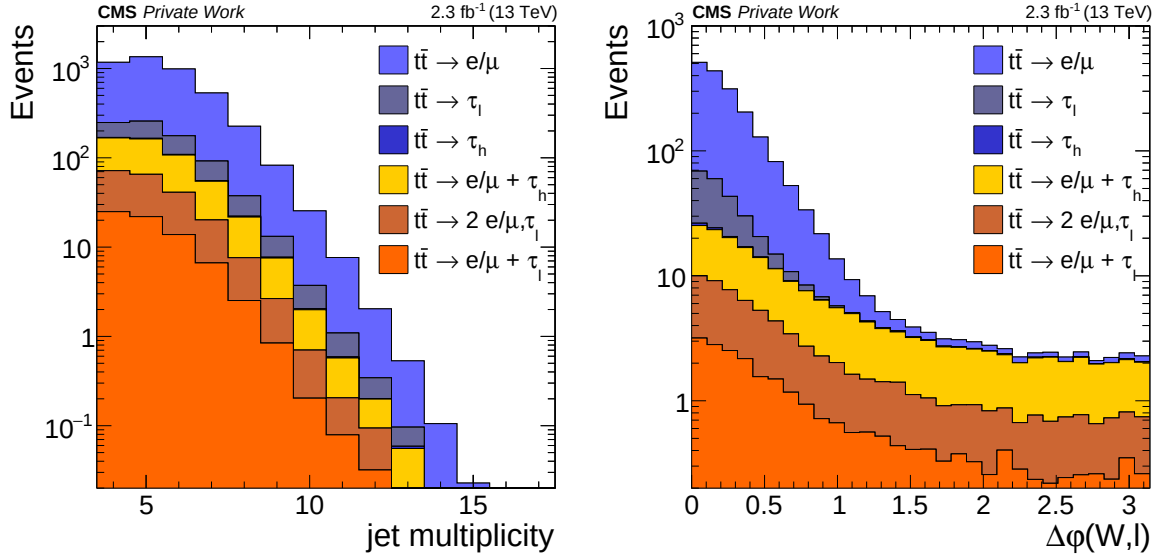
Fig. 6.2: Jet multiplicity and \Delta\phi distributions for the different components of the t\bar{t} decay after the baseline selection. Only the most contributing channels are chosen. For the left ( right ) plot an n_{\text{jet}} requirement of \geq 4 ( 6 ) jets is applied.
