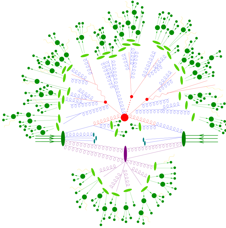
Fig. 2.12: Schematic view of a t\bar{t}H event produced in a pp-collision: the hard scattering is shown as a red blob with the solid and dashed lines as the resulting three particles [100]. Independently happening multi-particle interactions are indicated by the violet blob. The initial- and final-state radiation is shown with curly lines. Hadronization yields hadrons as shown in light green, while the final state particles are dark green.
