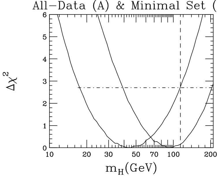
Figure 2: \Delta\chi^2 distributions for fits A and D. The dot-dashed line denotes the 95% CL upper and lower limits and the dashed line indicates the experimental lower limit on m_H .
