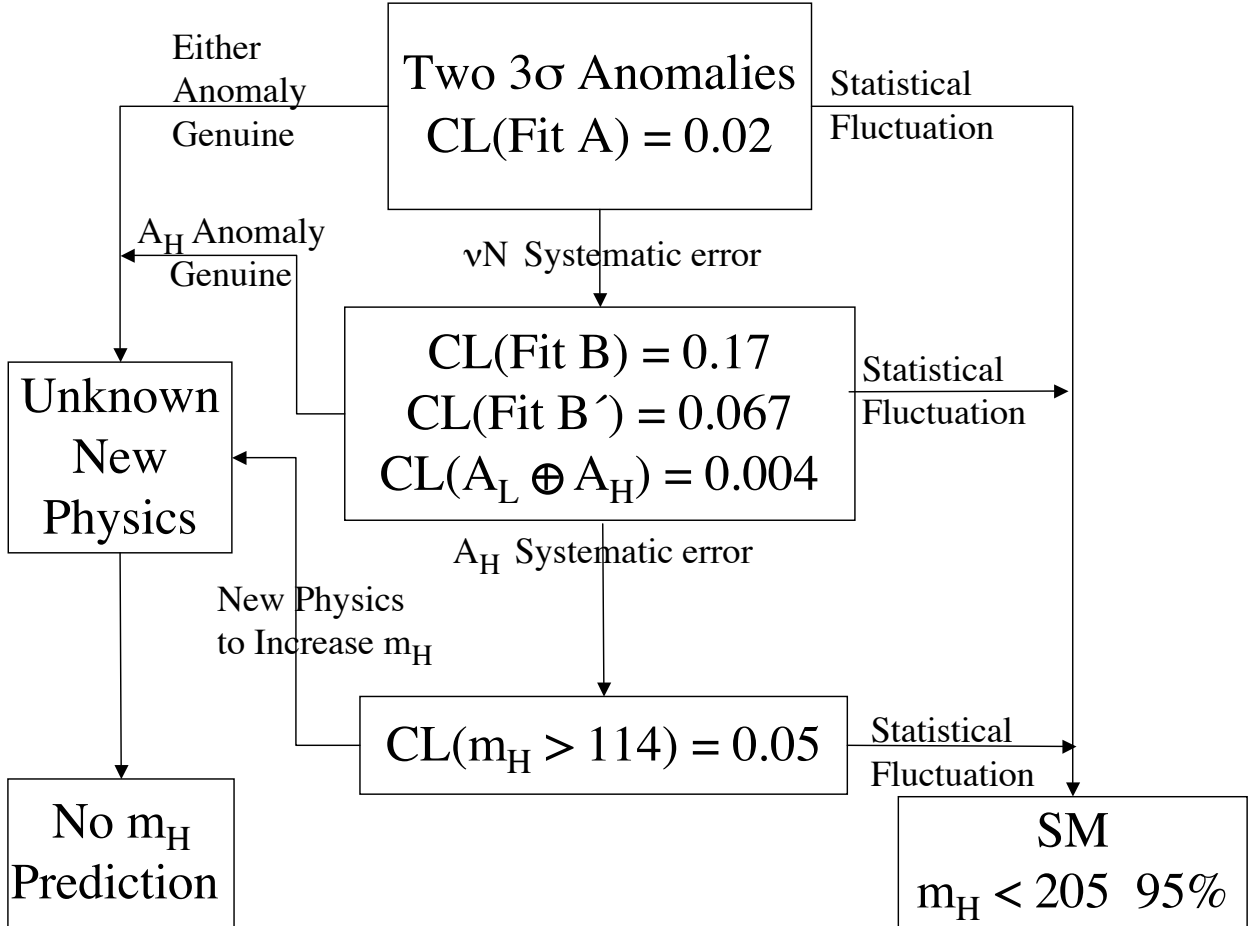
Figure 4: Electroweak schematic diagram.
