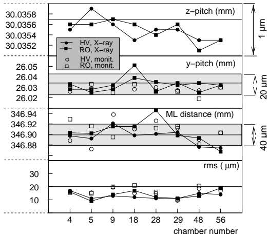
Figure 1: X-ray measurements (full symbols) of the wire grid parameters at the high-voltage (HV) and the readout (RO) end of the MDT chambers, in comparison with the monitoring during the construction (open symbols). The last row shows the standard deviations of the wire positions with respect to the nominal wire grid as obtained from the X-ray measurement and from the optical measurements. The horizontal lines represent the nominal values.
