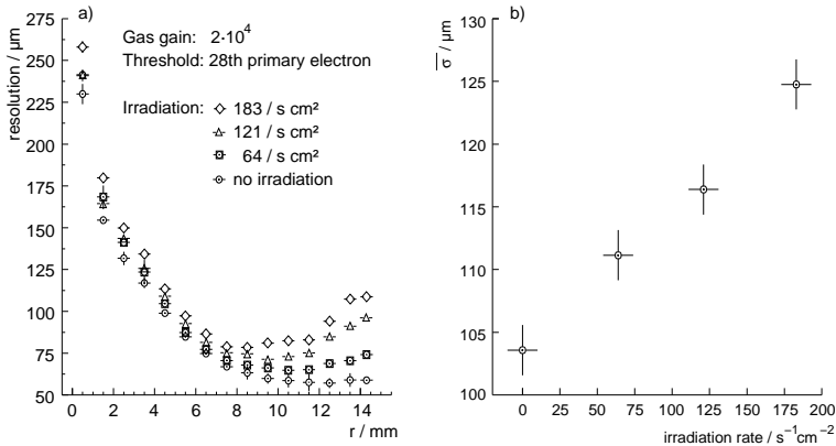
Figure 2: a) Spatial resolution of a single drift tube as a function of the impact radius r for different \gamma irradiation rates. b) Average spatial resolution \bar{\sigma} of a drift tube as a function of the \gamma irradiation rate.
