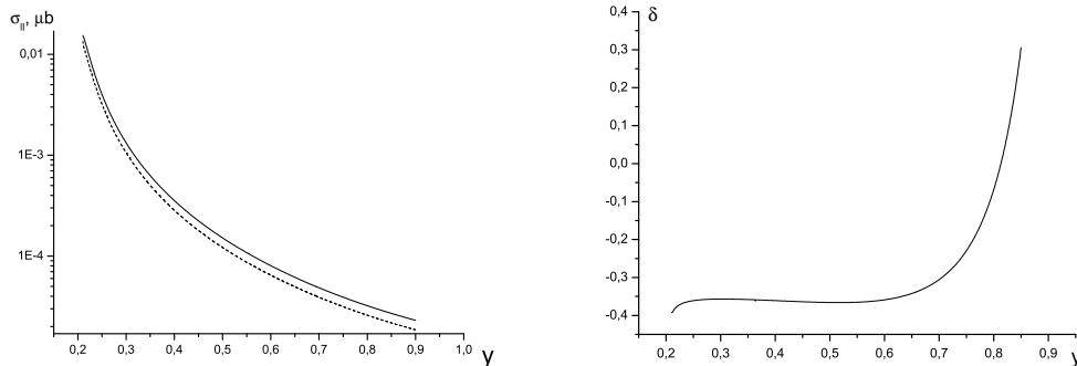
Figure 2: y -dependence of the cross section (2) (the left figure) and the quantity \delta (the right figure) in the case of the longitudinal polarization for the target polarization T = 0.83 [6]. The rest notations are the same as Fig.1
