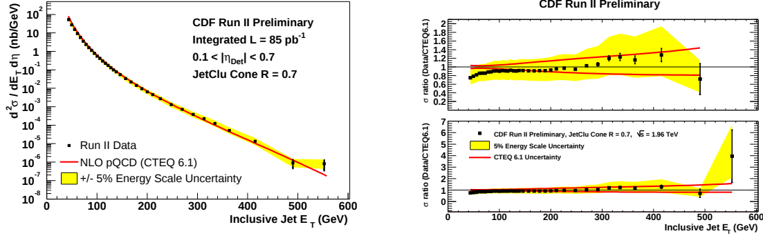
Figure 3: The inclusive jet cross section as measured by CDF for 0.1 < |y| < 0.7 compared with the JETRAD prediction with the CTEQ61 PDF. The left hand plot is on a logarithmic scale and the right hand plot shows the data divided by the theoretical prediction.
