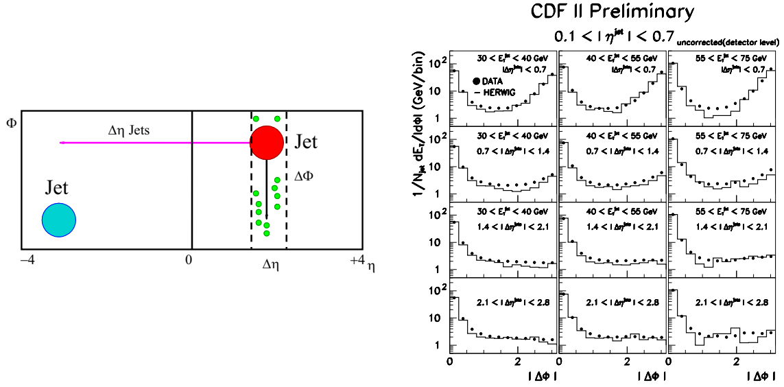
Figure 12: The CDF measures the energy outside of a jet, along a band of width \Delta\phi = 0.7 centered on the \phi axis of the jets as a function of the separation between the two leading p_T jets in the event, \Delta\eta . The left hand plot illustrates the measurement and the right hand plot compares the data with HERWIG.
