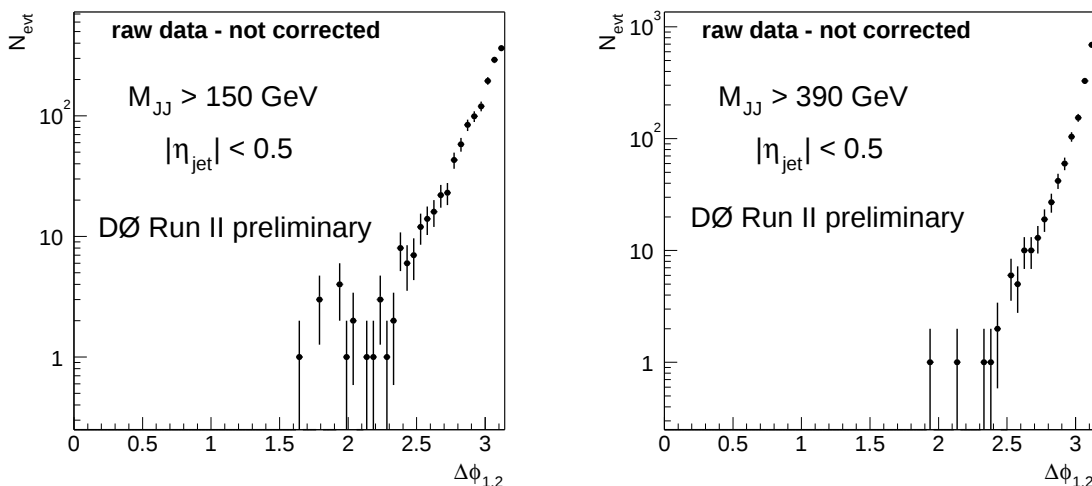
Figure 8: The separation in \phi between the two highest- p_T jets in the event above a given mass threshold. The left hand plot is for M_{JJ} > 150 \text{ GeV}/c^2 and the right hand plot is for M_{JJ} > 390 \text{ GeV}/c^2 .
