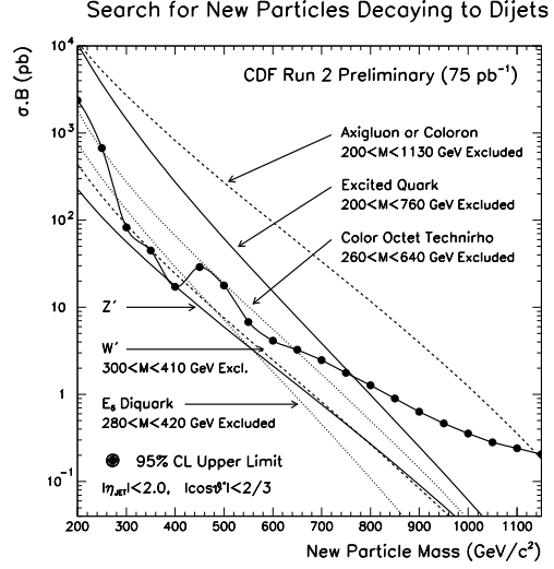
Figure 10: The 95% CL on the production cross section multiplied by B(X \rightarrow \text{dijet}) and acceptance for various theoretical models.
