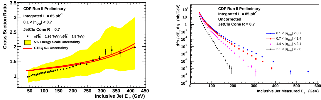
Figure 4: The ratio of inclusive jet cross sections at \sqrt{s} = 1960 divided by \sqrt{s} = 1800 GeV by CDF for 0.1 < |y| < 0.7 compared with the JETRAD prediction.
