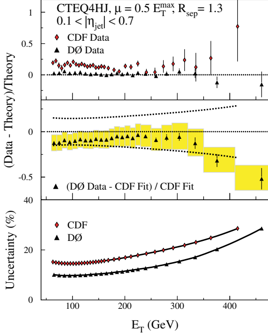
Figure 1: Inclusive Jet Cross Sections for 0.1 < |\eta| < 0.7 from DØ and CDF compared to the theory prediction JETRAD with the CTEQ4HJ PDF.
