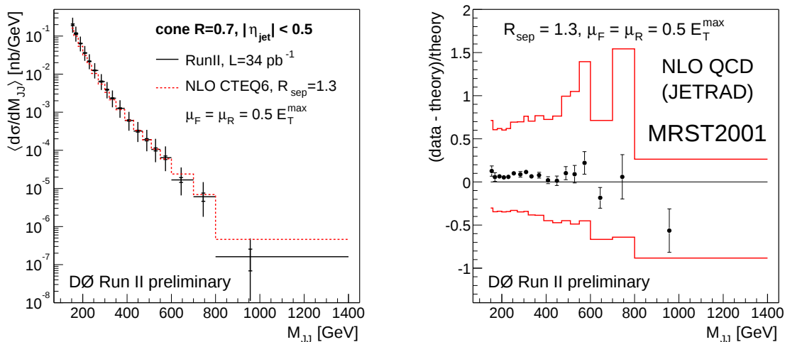
Figure 7: The dijet mass cross section as measured by DØ for |y| < 0.5 compared with JETRAD predictions. The left hand plot is on a logarithmic scale and uses the CTEQ6M PDF and the right hand plot shows The difference between the data and the prediction, divided by the prediction using the MRST2001 PDF.
