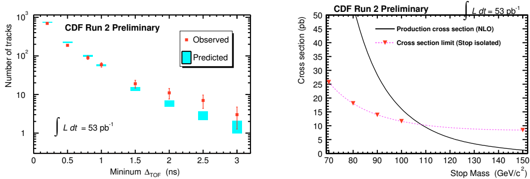
Figure 6: Search for charged massive stable particles at CDF : \Delta_t distribution measured with the time of flight detector (left), cross section upper limit as a function of the stop mass (right).
