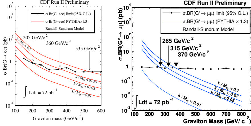
Figure 9: Search for small extra dimensions at CDF : Cross section limits as a function of the Randall Sundrum graviton mass in the dielectron (left) and dimuon (right) channels.
