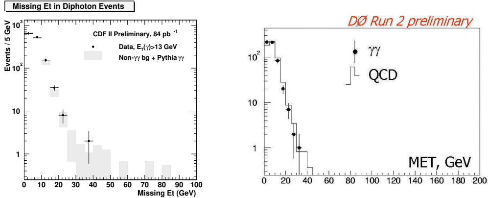
Figure 4: Search for photon events in GMSB at CDF and DØ : Missing E_T distribution for data (points) and backgrounds (histogram) in the CDF (left) and DØ (right) analyses.
