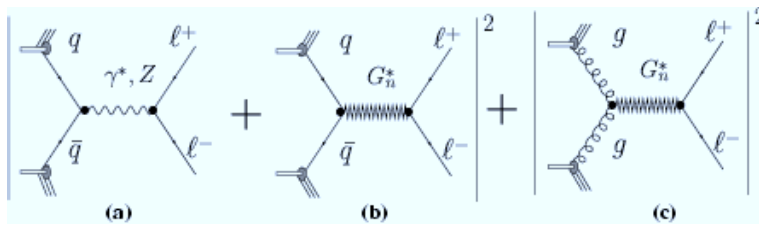
Figure 10: Feynman diagrams showing contributions of virtual graviton exchange to Drell-Yan processes.
