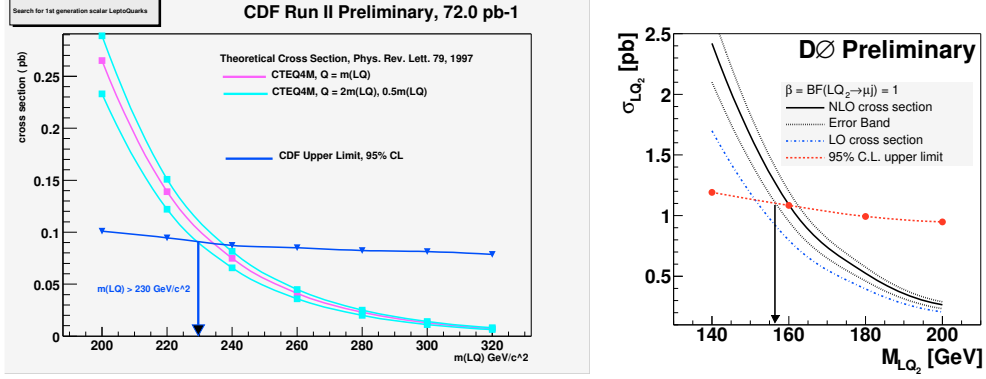
Figure 5: Search for leptoquarks : 95% cross section limit as a function of the leptoquark mass for the CDF analysis LQ_1 LQ_1 \rightarrow eeqq (left) and for the D\bar{O} analysis LQ_2 LQ_2 \rightarrow \mu\mu qq (right).
