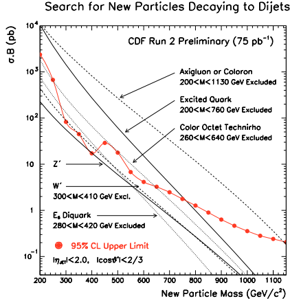
Figure 7: Search for resonances in dijets at CDF : 95% CL upper limits on the cross section times branching ratio for new particles decaying into dijets.
