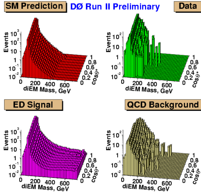
Figure 11: Large Extra Dimension search at D\emptyset in the diEM channel : invariant mass distribution as a function of \cos\theta^* for Standard Model expectation, data, LED signal and QCD background.
