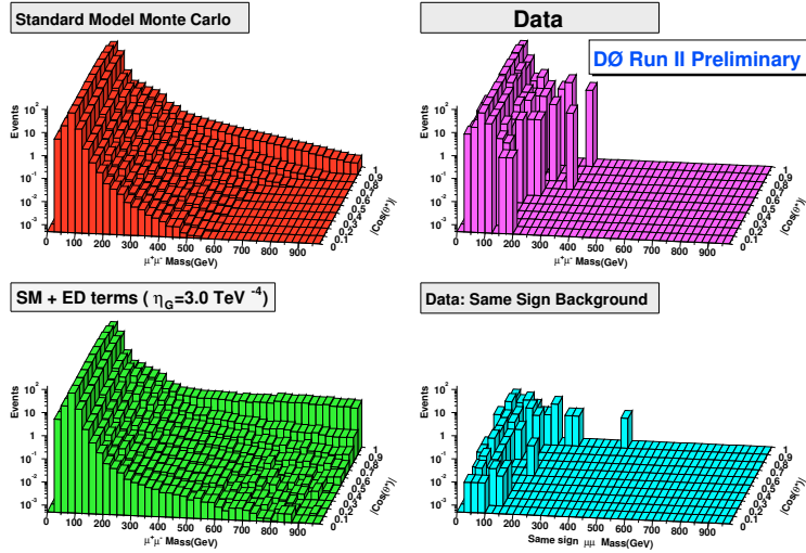
Figure 12: Large Extra Dimension search at DØ in the dimuon channel : invariant mass distribution as a function of \cos\theta^* for Standard Model expectation, data, LED signal and same-sign dimuon background.
