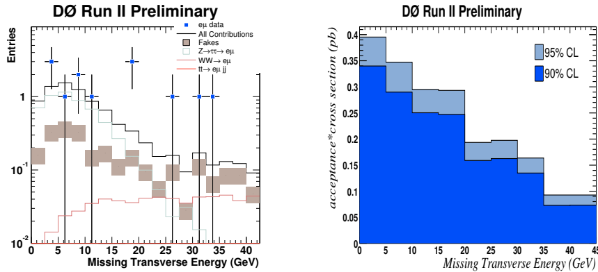
Figure 2: Search for e\mu at D\bar{O} : Missing E_T distribution (left) and cross section limit as a function of the missing E_T cut (right).
