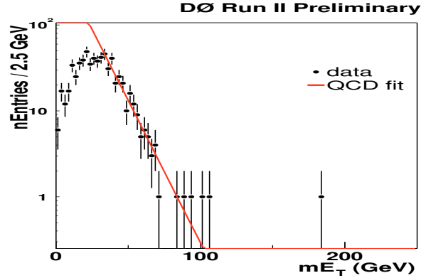
Figure 1: Search for jets and missing E_T at D\bar{O} : missing E_T distribution for data (dot) and the QCD fit (line).
