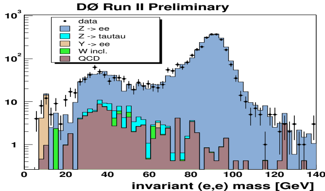
Figure 3: Search for eel at DØ : dielectron invariant mass distribution.
