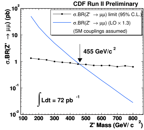
Figure 8: Search for extra gauge bosons Z' : Drell-Yan dilepton invariant mass spectra (left) and the corresponding cross section limit (right) of CDF dielectron analysis (upper), of D\bar{O} dielectron analysis (middle) and of CDF dimuon analysis (lower).
