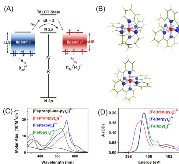
Fig. 4 (A) Schematic of probing a Fe(II) complex in O_h -symmetry at the N K-edge (1s spectroscopy). (B) Molecular structures of [\text{Fe}(\text{tren}(\text{py})_3)]^{2+} , [\text{Fe}(\text{terpy})_3]^{2+} , and [\text{Fe}(\text{bpy})_3]^{2+} . (C) Optical absorption spectra showing MLCT bands of the three Fe complexes. (D) Transmission N K-edge XAS spectra of solid [\text{Fe}(\text{tren}(\text{py})_3)]^{2+} (red), [\text{Fe}(\text{terpy})_3]^{2+} solution (blue), and [\text{Fe}(\text{bpy})_3]^{2+} solution (green).
