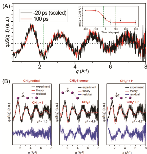
Fig. 11 (A) Time-resolved X-ray solution scattering curves of \text{CHI}_3 photolysis at the time delays of -20 ps (black) and 100 ps (red). (Inset) Temporal change of the intensity at a negative peak position ( q = 2.205 \text{ \AA}^{-1} , marked with a green dashed line in the main figure) displayed from -200 ps to 300 ps. (B) Theoretical difference scattering curves at -20 ps time delay for three candidate reaction pathways, (i) dissociation into \text{CHI}_2 radical and \text{I} , (ii) \text{CHI}_2\text{-I} isomer formation and (iii) dissociation into \text{CHI}_2^+ and \text{I}^- ions. Experimental (black) and theoretical (red) curves are compared at the top and the residual (blue) obtained by subtracting the two curves is displayed at the bottom.
