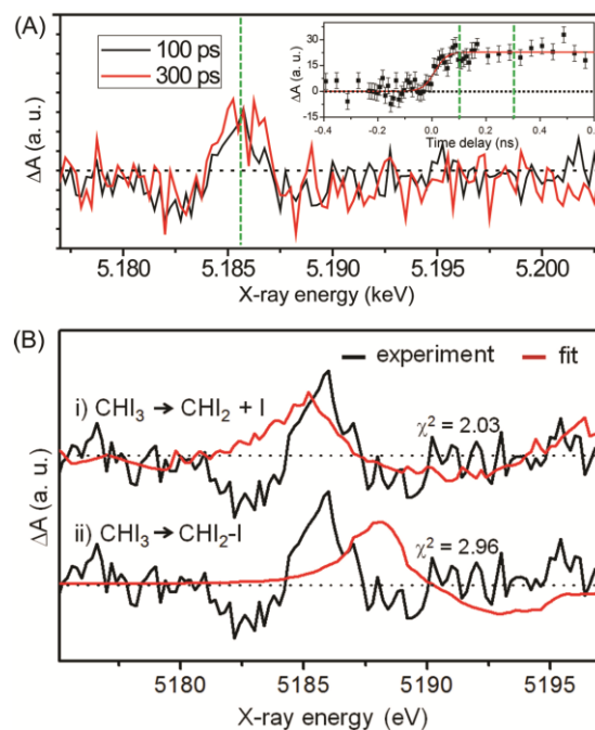
Fig. 12 (A) Time-resolved X-ray absorption spectra of the iodoform photolysis measured at the L1 edge of the iodine atom and at the time delays of 100 ps (black) and 300 ps (red). (Inset) Temporal change of the difference absorption intensity at a peak position of 5.1857 \text{ keV} (green dashed line) in the time range from -0.4 to 0.6 ns. (B) The fitting analysis of the L1-edge difference XANES spectrum measured at 100 ps for two candidate reaction pathways, (i) \text{CHI}_2 radical + \text{I} and (ii) \text{CHI}_2\text{-I} isomer formation. Experimental (black) and theoretical (red) difference XANES spectra are compared with each other.
