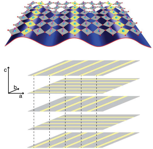
FIG. 1 (color online). Schematic drawing of the \text{La}_{1.875}\text{Ba}_{0.125}\text{CuO}_4 charge, spin, and lattice arrangement within a \text{CuO}_2 plane in the stripe-ordered, low-temperature tetragonal phase ( T < 55 K). Here, Cu atoms are shown as (big) blue, oxygen atoms as (small) red spheres. Holes form stripes which separate domains of oppositely phased antiferromagnetic domains (spins indicated by arrows). The LTT distortion is visible through the tilt of the octahedra central planes. The periodic stacking of those \text{CuO}_2 planes is sketched in the lower figure part. The stripe orientation rotates by 90^\circ between layers.
