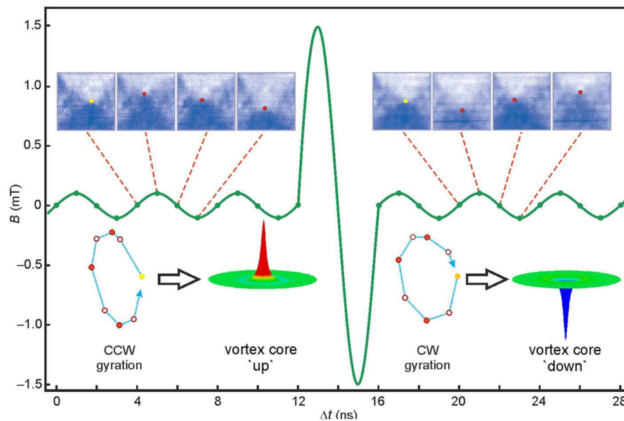
FIGURE 1 | Switching of the vortex core by excitation of the vortex gyromode at 250 MHz with a single period burst at an amplitude of 1.5 mT [7]. Permalloy sample: 1.5 \mu\text{m} in diameter, 50 nm thick. Before and
