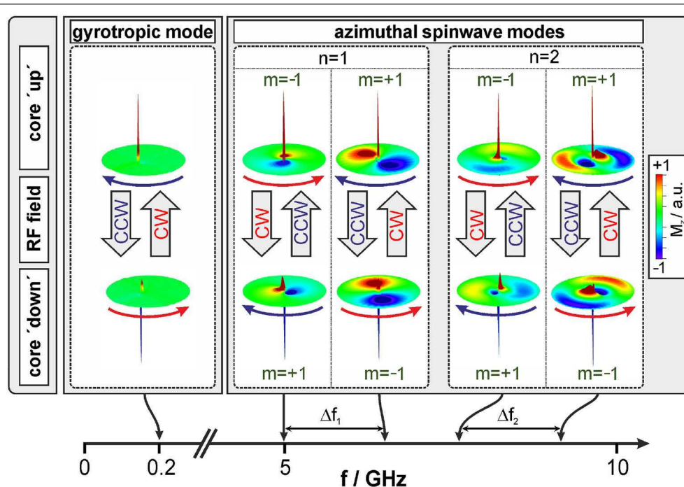
FIGURE 2 | Unidirectional vortex core reversal by excitation of the (sub-GHz) gyromode or (multi-GHz) azimuthal spin waves with external rotating magnetic fields [3]. Using 24 periods for
