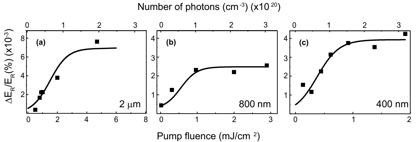
FIG. 3. Differential time-domain transient \Delta E_R/E_R measured at the THz electric-field peak 1.5 ps after photoexcitation plotted as a function of pump fluence for different excitation wavelengths. The black lines are sigmoid function fits, returning threshold fluences of 3.0, 1.1, and 0.75 mJ/cm 2 for 2- \mu m, 800-, and 400-nm excitation wavelengths, respectively. On the top horizontal scale the fluence is expressed in terms of total number of absorbed photons per unit volume, returning a saturation value of \sim 10^{20} photons/cm 3 , independent of pump wavelength.
