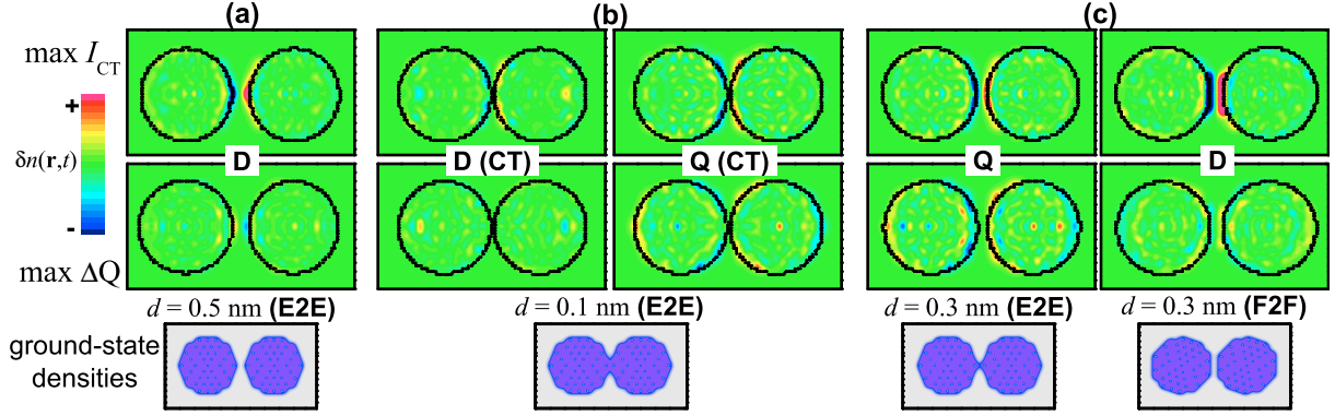
Figure 4: Snapshots of the induced electron densities at different resonant frequencies, as indicated in each panel. The top panels depicts the induced densities when the current between clusters reaches a maximum, whereas the second line corresponds to induced densities when the charge difference between clusters is maximum (zero intensity). The scale range is -\rho \leq \delta n \leq +\rho , where \rho = 0.5 \times 10^{-6} a.u. for d = 0.1 nm and d = 0.3 nm, whereas \rho = 10^{-6} a.u. for d = 0.5 nm. A sketch of the corresponding ground-state electron densities is also shown to illustrate the different contact regimes.
