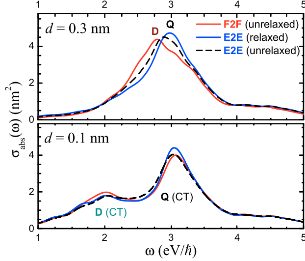
Figure 3: The impact of the atomic relaxation on the absorption cross sections for E2E \text{Na}_{297} dimers at separations d = 0.1 nm and d = 0.3 nm. Optical absorption for relaxed geometries: solid blue lines; absorption for unrelaxed geometries: dashed lines. For the sake of comparsion, the corresponding F2F spectra are also depicted (red solid lines).
