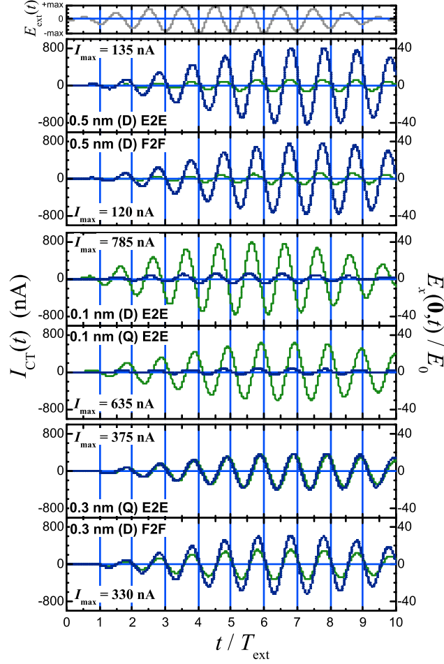
Figure 5: Time evolution of induced currents (solid green lines) and total electric fields (dotted blue lines) at the middle of the dimer junction ( \mathbf{r} = \mathbf{0} ) due to the resonant coupling of selected modes of the nanoparticle dimer with an applied external field (depicted in the upper panel) of frequency \omega_{\text{ext}} . In each panel we indicate the maximum value of the induced intensity, I_{\text{CT}} , corresponding to an incident electric field with maximum amplitude E_0 = 10^{-6} a.u..
