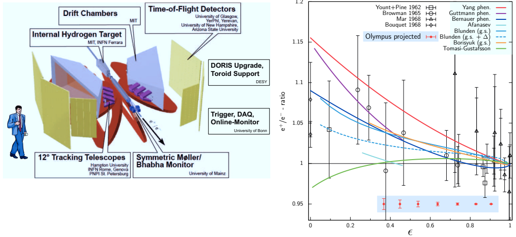
Figure 2. Left: Schematic layout of the OLYMPUS experiment with components labeled in the figure. Right: Projected precision of OLYMPUS for the e^+p to e^-p cross section ratio versus \epsilon along with previous data [27] and various theoretical predictions [12–18], which have been evaluated for a constant beam energy of E = 2 GeV.
