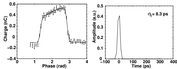
Figure 3: Charge measured at the gun exit as a function of the relative phase gun/laser (left) and the reconstructed laser pulse length from the rising edge (right).
