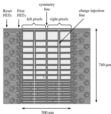
Figure 2: The silicon pixel detector.
