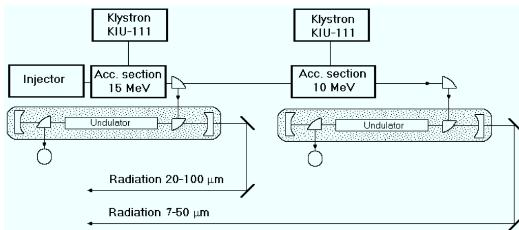
Figure 1: General layout of free electron laser
