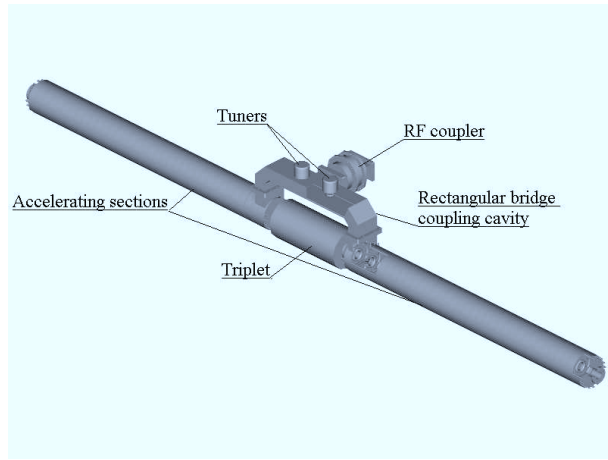
Fig. 2: Accelerating cavity in the second PPA part.
