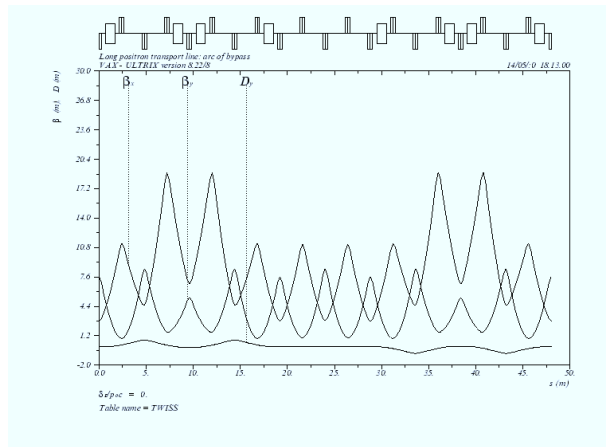
Fig. 4. Behaviour of optical functions along one bypass arc.
