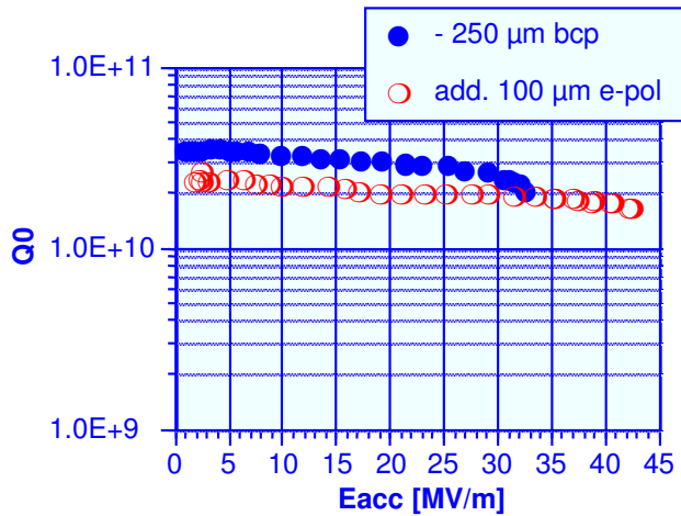
Figure 6: Q vs E_{acc} for cavity 1K2 after bcp and ep surface treatment.
