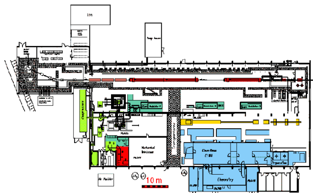
Figure 1: The TESLA Test Facility.
