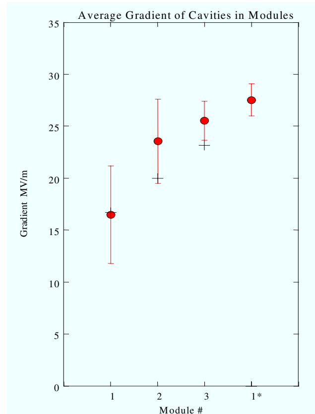
Figure 4: Average gradient, as measured in vertical tests, of the 9-cell cavities assembled into accelerator modules. Crosses indicate the gradients obtained in the module.
