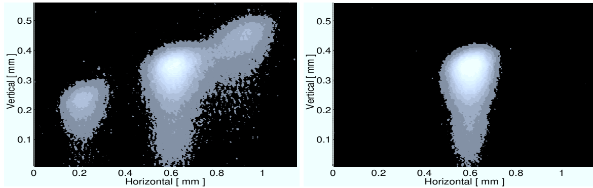
Figure 5: Synchrotron radiation image of the beam near the 3 \nu_x resonance. Left is the situation before the optic is corrected and right is the situation after the optic is corrected. (There is a distortion in the light optic in the vertical plane that is responsible for the vertical asymmetry of the image).
