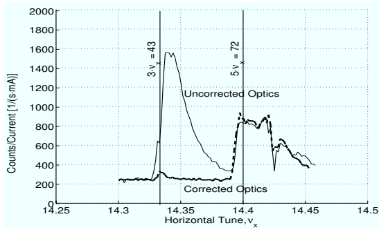
Figure 3: Horizontal tunes scans before (thin,solid) and after (thick,dotted) the optic is corrected. The vertical tune is kept constant at 8.15. At each horizontal tune, the count rate (as measured in a gamma counter) divided by beam current is plotted.
