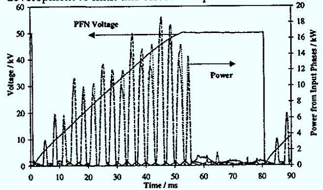
Figure 5: Charging voltage and power extracted from the three phases of the mains during one charging cycle
