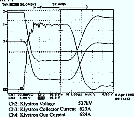
Figure 2: Typical waveforms
