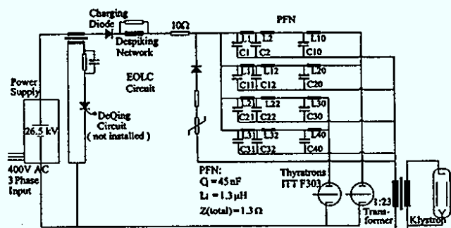
Figure 1: Basic circuit diagram
