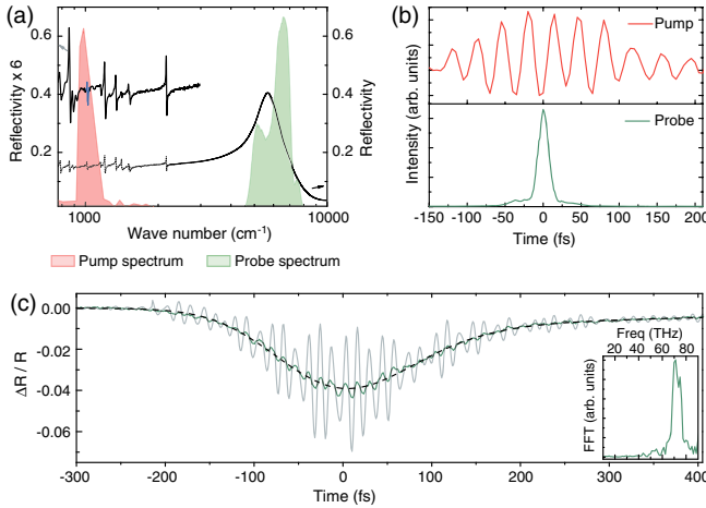
FIG. 3 (color online). (a) (red) Spectrum of the midinfrared excitation pulses centered at 1000 cm -1 (10 μm wavelength) resonant to the ET molecular vibration mode (blue). The sample reflectivity in direction perpendicular to the a axis is shown in gray. (green) The spectrum of the near-infrared probe beam covers the charge transfer band along the a axis. (b) (upper panel) Phase-locked electric field of the midinfrared pump pulse measured via electro-optic sampling; (lower panel) intensity profile of NIR probe pulse. (c) (green) Spectrally integrated time-dependent reflectivity changes in ET-F 2 TCNQ at a pump fluence of 0.9 mJ/cm 2 at room temperature, together with a double exponential fit of the form A\exp(-t/t_d + 1)\sum_{i=1,2}A_i\exp(-t/\tau_i) in dashed black. The gray solid line shows the deconvolved reflectivity changes, and the inset shows a Fourier transformation of the measured oscillations peaking at 70 THz.
