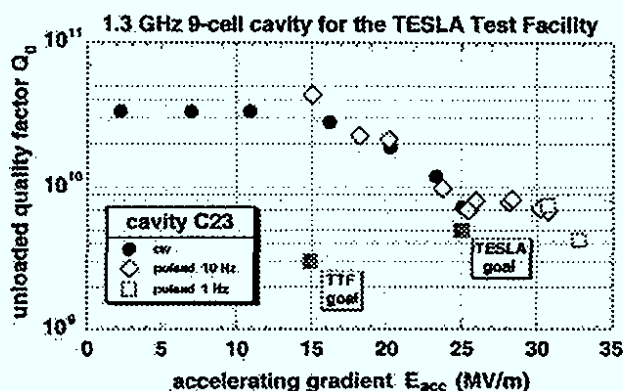
Fig. 2: The best TESLA 9-cell cavity measured in a horizontal test cryostat. For this test the cavity is equipped with the main RF input coupler and the HOM couplers.
