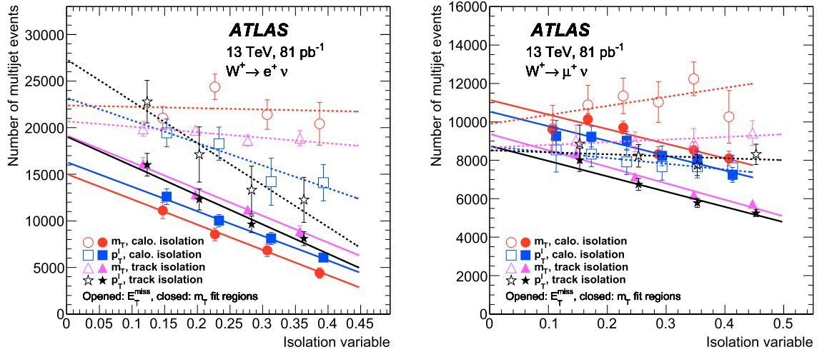
Fig. 1. The number of multijet events versus the isolation variable for the W^+ \rightarrow e\nu (left) and W^+ \rightarrow \mu\nu (right) analysis is shown. The plots illustrate the multijet-evaluation methodology for the W^+ analysis. The results obtained for two of the four discriminant variables used to evaluate the multijet yields are shown for both types of isolation: m_T (circles) and p_T^\ell (squares) with calorimeter-based isolation and m_T (triangles) and p_T^\ell (stars) with track-based isolation. Open markers represent the yields obtained with the E_T^{\text{miss}} fit region while closed markers are those with the m_T fit region. The points represent the extracted multijet fraction from the fit of the variables, in the isolation intervals represented on the x-axis for the template selection. The lines represent the linear extrapolation of the points to the signal region. The definition of the signal region is p_T and isolation-flavour dependent but corresponds approximately to the region of isolation below 0.1 in these plots. The error bar in each bin represents the uncertainty from the fit of the variable rescaled by the square root of the reduced \chi^2 of the fit.
