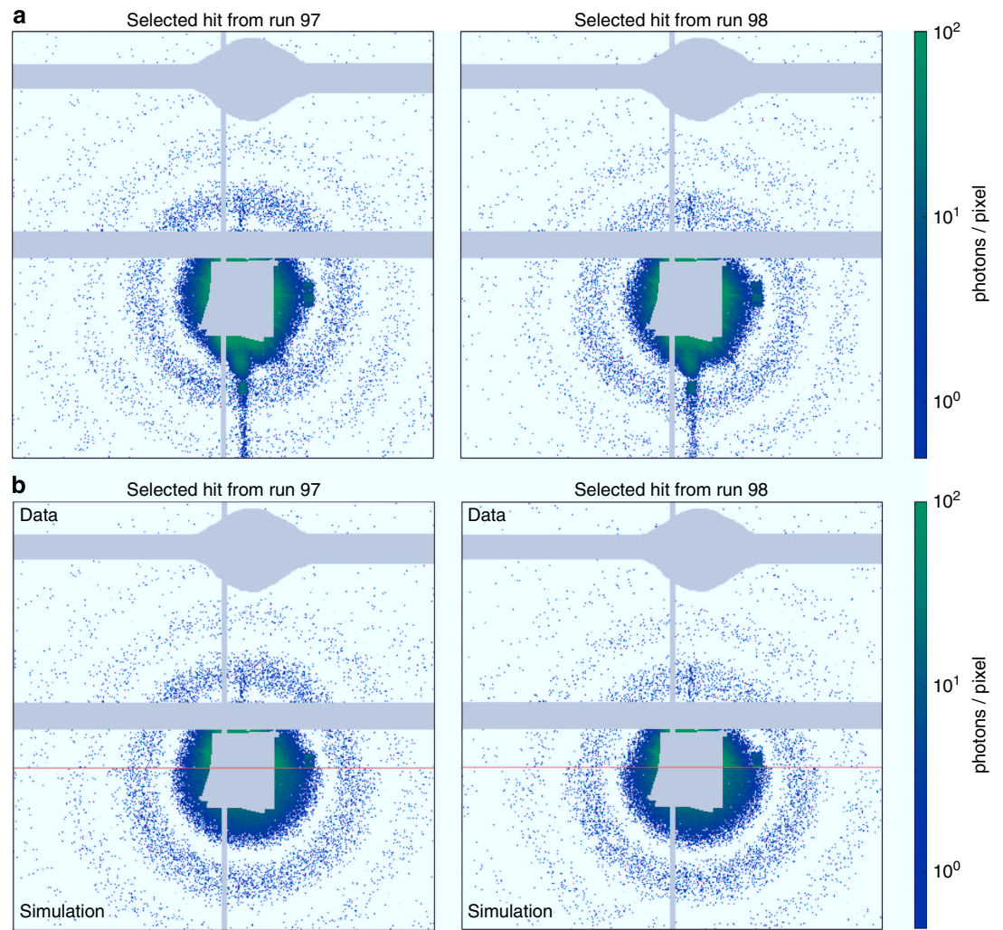
Figure 5. Measured and simulated diffraction patterns of single RDV particles. (a) , Two hits on the back detector, selected on the expected size for RDV and high diffraction intensity. (b) , Measured and simulated data combined. The top half of each of the two patterns shows the measured signal and is identical to the top halves of the patterns in (a) . The bottom half of each pattern shows simulated diffraction data from a homogenous sphere of size 71 nm and with a mass density of 1.381 \text{ g cm}^{-3} . The simulation assumes a photon energy of 7 keV, a detector distance of 2.4 m, a pixel size of 110 microns and a conversion of 33 ADUs per photon. Regions of beam-stops and gaps between the detector panels are masked in grey.
