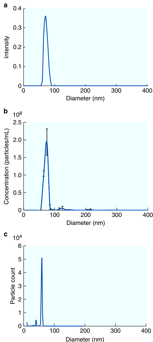
Figure 2. The purity of RDV was analyzed with DLS, NTA and DMA. (a) , Size distribution determined with DLS. The average size of the RDV particles was approximately 76 nm. (b) , Size distribution determined with NTA. The mean and mode of the RDV particles were approximately 76 and 73 nm, respectively. (c) , DMA measurement of RDV gave an apparent particle diameter of approximately 60 nm. Here the actual gas flow was lower than the set value, which resulted in an under estimation of the particle size by about 10%. The main purpose of the DMA measurement was to assess sample purity and the results show that.
