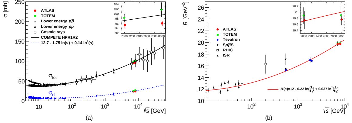
Figure 4: (a) Comparison of total and elastic cross-section measurements presented here with other published measurements [2, 35–39] and model predictions as a function of the centre-of-mass energy. (b) Comparison of the measurement of the nuclear slope B presented here with other published measurements at the ISR, at the Spp\bar{p}S , at RHIC, at the Tevatron and with the measurement from TOTEM at the LHC. The red line shows a model calculation [40], which contains a linear term and quadratic term in \ln s .
