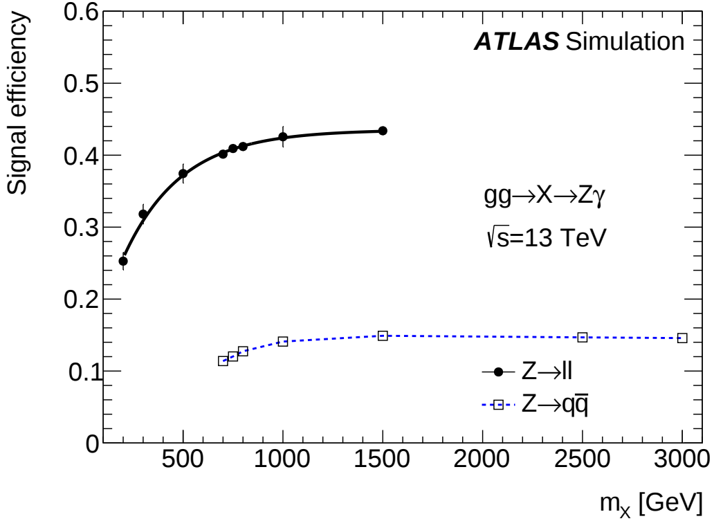
Fig. 2. Efficiency of the leptonic selection for simulated signal events in which Z bosons decay to \ell\ell (solid circles), and of the hadronic selection for simulated signal events in which the Z bosons decay to q\bar{q} (open squares), as a function of the resonance mass m_X . The solid line represents an interpolation with a smooth function (of the type a + be^{cm_X} ) of the leptonic analysis efficiency, while the dashed line represents a linear, piece-wise interpolation of the efficiencies of the hadronic analysis.
