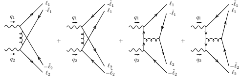
Figure 3: Diagrams contributing to M_H for \gamma_L^* .
