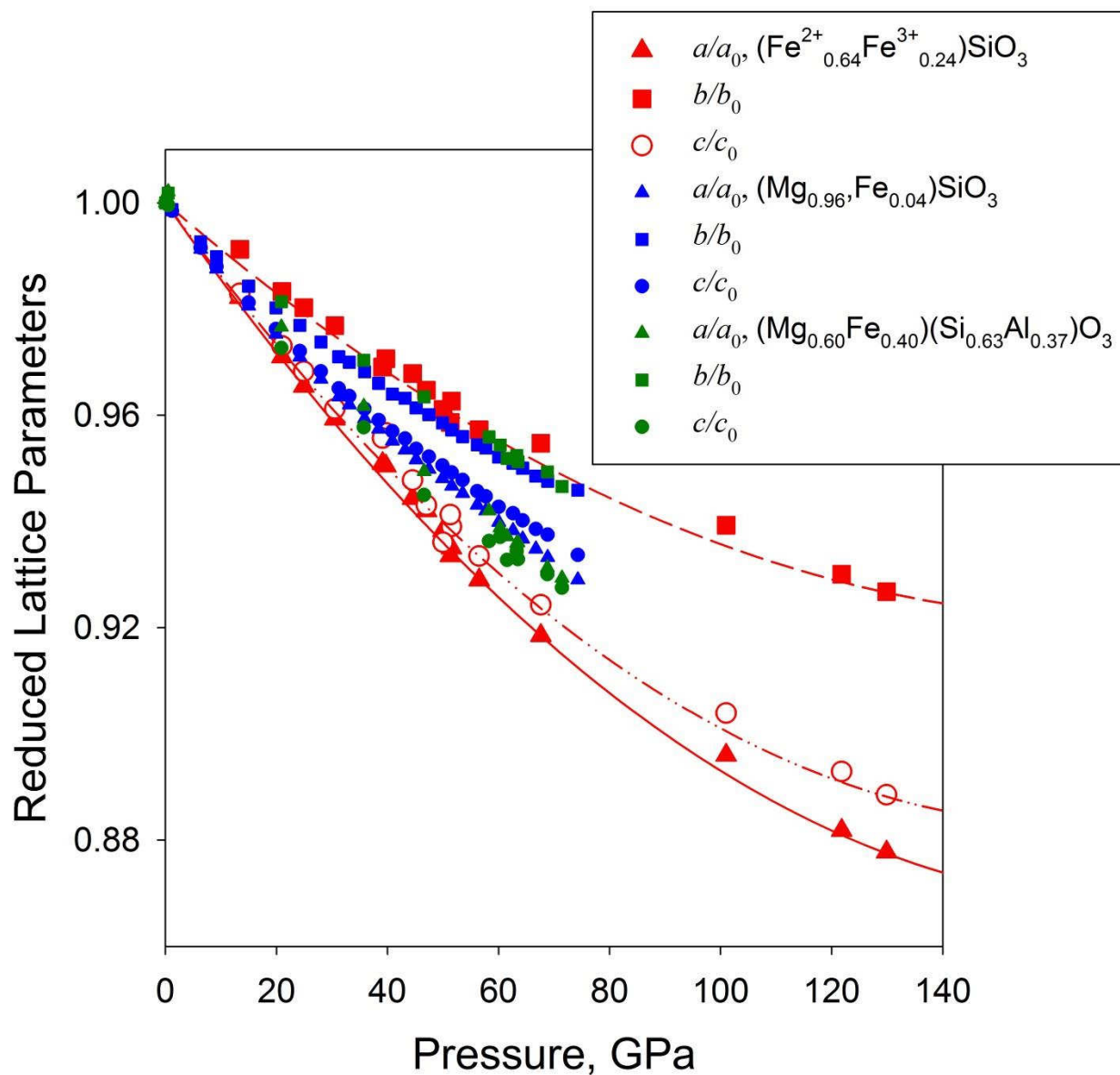
fig.S7. Variation with pressure of the normalized unit-cell parameters for three bridgmanites—Fe-bridgmanite (this study), (\text{Mg}_{0.96}, \text{Fe}_{0.04})\text{SiO}_3 (32), and \text{Mg}_{0.60}\text{Fe}_{0.40}\text{Si}_{0.63}\text{Al}_{0.37}\text{O}_3 . (12) Note the clearly different behavior of the a - and b -axis of Fe-bridgmanite.
