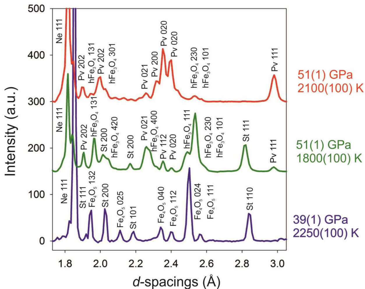
fig. S5. Typical powder x-ray diffraction patterns of skiaegite-majorite garnet that was laser-heated at different pressures and temperatures (St, stishovite; \text{hFe}_3\text{O}_4 , orthorhombic \text{CaTi}_2\text{O}_4 -type \text{Fe}_3\text{O}_4 , Pv, perovskite-structured phase). Pressure was determined using Ne lattice parameters (see http://kantors50webs.com/diffraction.htm ).
