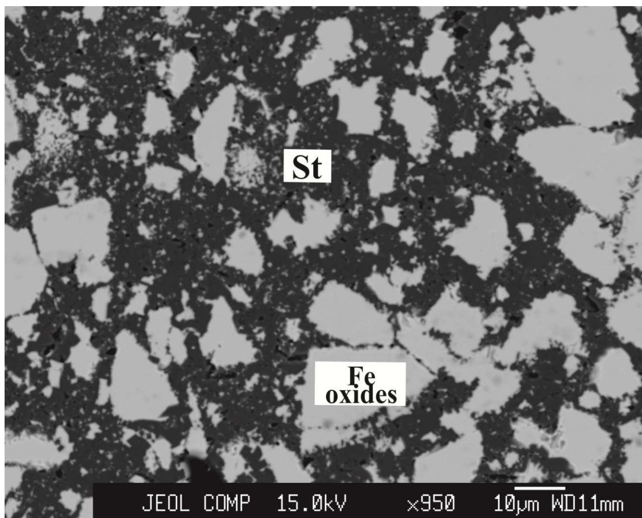
fig S4. Backscattered electron image of skiagite starting composition at 23 GPa and 1600°C (run S6151). Skiagite-majorite garnet decomposes to oxides: dark gray – \text{SiO}_2 (stishovite), light gray – Fe oxides ( \text{Fe}_{1-x}\text{O} and \text{Fe}_4\text{O}_5 ).
