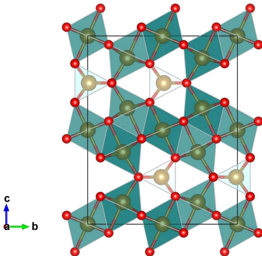
fig S6. Crystal structure of \text{Fe}_4\text{O}_5 obtained as the product of decomposition of skiaegite-majorite garnet in a laser-heated DAC at 39(1) GPa and 2250(100) K (see table S4 for crystallographic data). Fe1 occupy trigonal-prismatic sites (light green) and Fe2 and Fe3 occupy the two slightly different octahedral sites (green). Red balls represent oxygen atoms.
