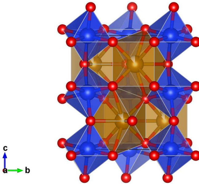
fig. S3. Representative polyhedral structural model of orthorhombic bridgmanite. The bridgmanite structure (space group Pbmn , #62) has two cation positions – a distorted bi-capped prism (“A”-site, brown) and octahedra (“B-site”, blue). Red balls represent oxygen atoms. For the case of (\text{Fe}^{2+}_{0.64(2)}\text{Fe}^{3+}_{0.24(2)})\text{Si}_{1.00(3)}\text{O}_3 bridgmanite (synthesized, for example, at 67 GPa and 2200(100)K; orthorhombic Pbmn , a=4.5516(3) Å, b=4.7753(15) Å, c=6.5497(4) Å, V=142.36(5) Å 3 ) vacancies on the A-site are indicated in white.
