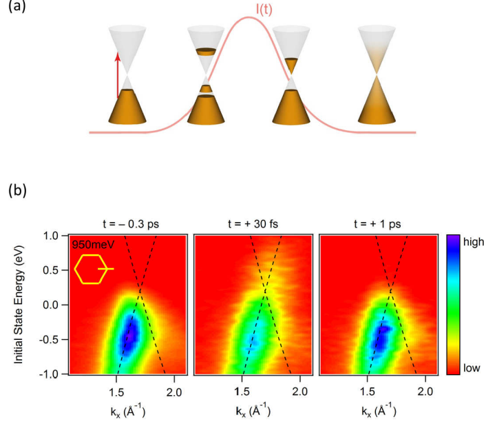
FIG. 4: Direct interband transition regime for excitation at \hbar\omega_{\text{pump}} = 950\text{ meV} : (a) Cartoon of the excitation mechanism. The red line represents the intensity envelope of the pulse. If \hbar\omega_{\text{pump}} > |2\mu_e| , the graphene layer is excited via direct interband transitions that leave the system with a highly non-thermal electron distribution that cannot be observed within the temporal resolution of the present experiment. Within \sim 10 femtoseconds the electrons thermalize and form separate Fermi-Dirac distributions for the valence and conduction band. After some hundreds of femtoseconds the separate chemical potentials merge, resulting in a single Fermi-Dirac distribution for valence and conduction band. (b) Snapshots of the band structure (smoothed) for excitation at \hbar\omega_{\text{pump}} = 950\text{ meV} with a fluence of F = 4.6\text{ mJ/cm}^2 and a probe photon energy of \hbar\omega_{\text{probe}} = 31.5\text{ eV} . The measurements were done along the \bar{\Gamma}\text{K} -direction (inset). Dashed black lines represent the dispersion obtained from a tight-binding model [20].
