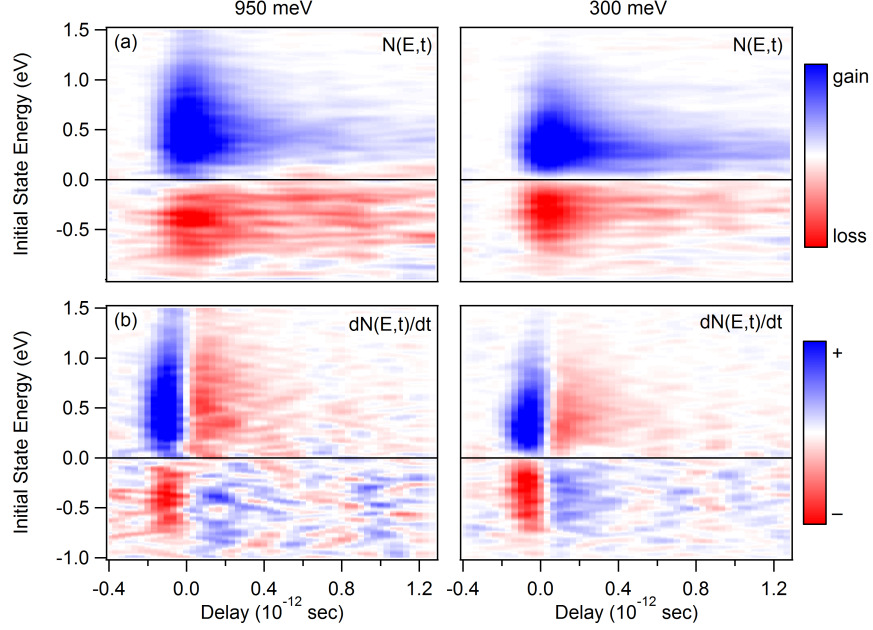
FIG. 6: No indication of carrier multiplication for direct interband transitions (left column) and free carrier absorption (right column): The pump-probe signal in panel (a) is given by the difference between the photocurrent shown in Figs. 3a and 5a, respectively, and the photocurrent at negative time delays. Panel (b) shows the time derivative of the pump-probe signal, which is equivalent to the electron-hole pair generation/recombination rate. Electron-hole pairs are generated only for a short time interval in the presence of the pump pulse. The data has been smoothed.
