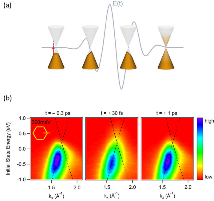
FIG. 2: Free carrier absorption regime for excitation at \hbar\omega_{\text{pump}} = 300 \text{ meV} : (a) Cartoon of the excitation mechanism. For \hbar\omega_{\text{pump}} < 2|\mu_e| direct interband transitions are impossible. The Fermi liquid sloshes around the Dirac cone following the electric field E(t) of the laser pulse (light grey line) like water in a shaking glass. Electron-electron and electron-phonon scattering events subsequently establish a thermal Fermi-Dirac distribution. Within the time resolution of the present investigation the coherent dynamics at earliest times could not be resolved. (b) Snapshots of the band structure (smoothed) close to the \bar{\text{K}} -point for different pump-probe delays: negative time delays (left), close to zero delay (+30 fs, middle), t = 1 \text{ ps} (right). The sample is excited at \hbar\omega_{\text{pump}} = 300 \text{ meV} with a fluence of F = 0.8 \text{ mJ/cm}^2 . Photoelectrons are ejected using photons of energy \hbar\omega_{\text{probe}} = 31.5 \text{ eV} . The measurements were done along the \bar{\Gamma}\bar{\text{K}} -direction (inset), where the photocurrent is suppressed for one of the two \pi -bands [22]. Dashed black lines represent the dispersion obtained from a tight-binding model [20].
