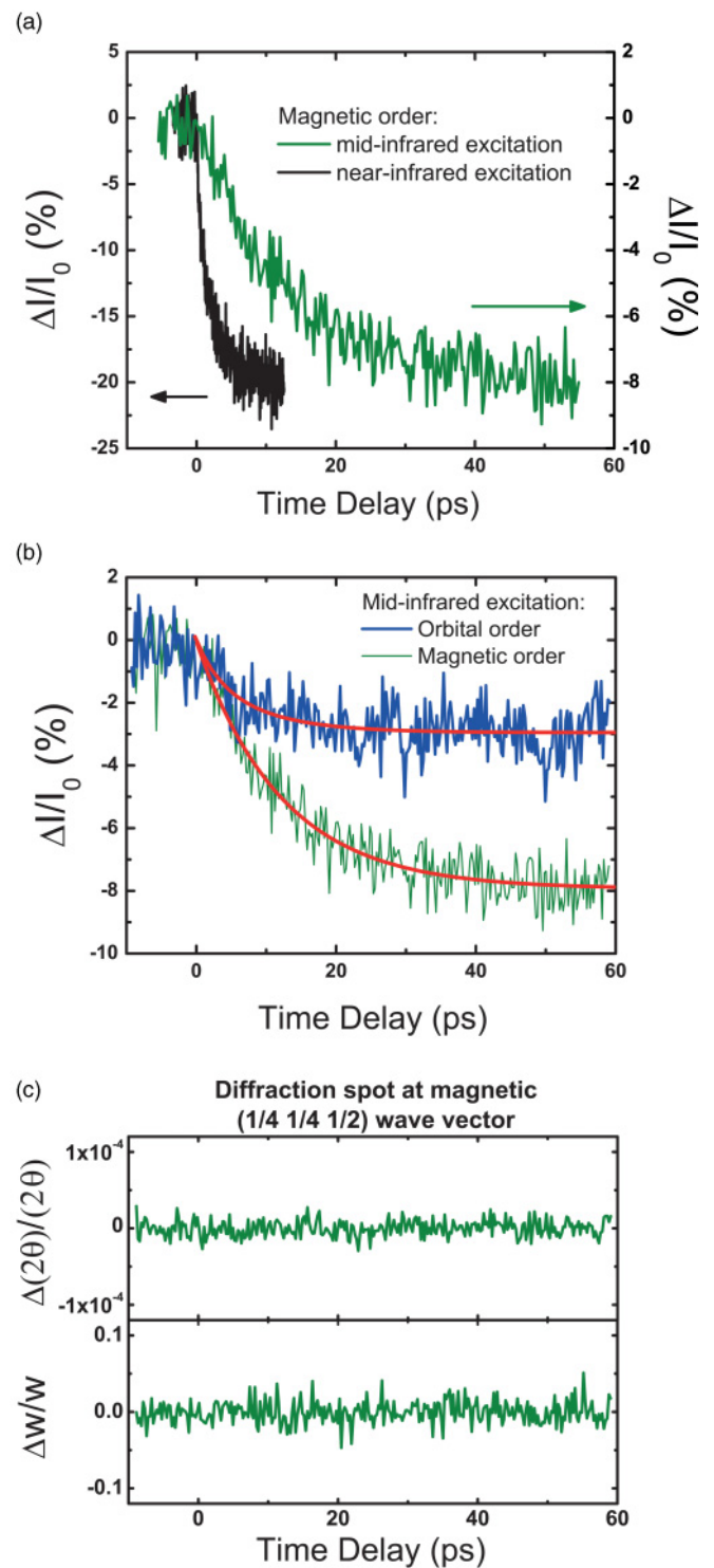
FIG. 2. (Color) (a) Time-resolved changes of the intensity of the scattered x-ray spot at the magnetic (\frac{1}{4}\frac{1}{4}\frac{1}{2}) diffraction peak for vibrational excitation at 13.8\text{ }\mu\text{m} (midinfrared) and photodoping at 800\text{-nm} (near-infrared) pump wavelengths. Excitation fluences are 1.2 and 5\text{ mJ/cm}^2 , respectively. (b) Comparison of the melting of the orbital and magnetic order for 1.2\text{-mJ/cm}^2 midinfrared excitation. The red lines are single exponential fits to the data, with time constants of 6.3 and 12.2\text{ ps} , respectively. (c) Transient change of the scattering angle 2\theta and the width w of the diffracted x-ray spot measured for the magnetic wave vector following the midinfrared excitation.
