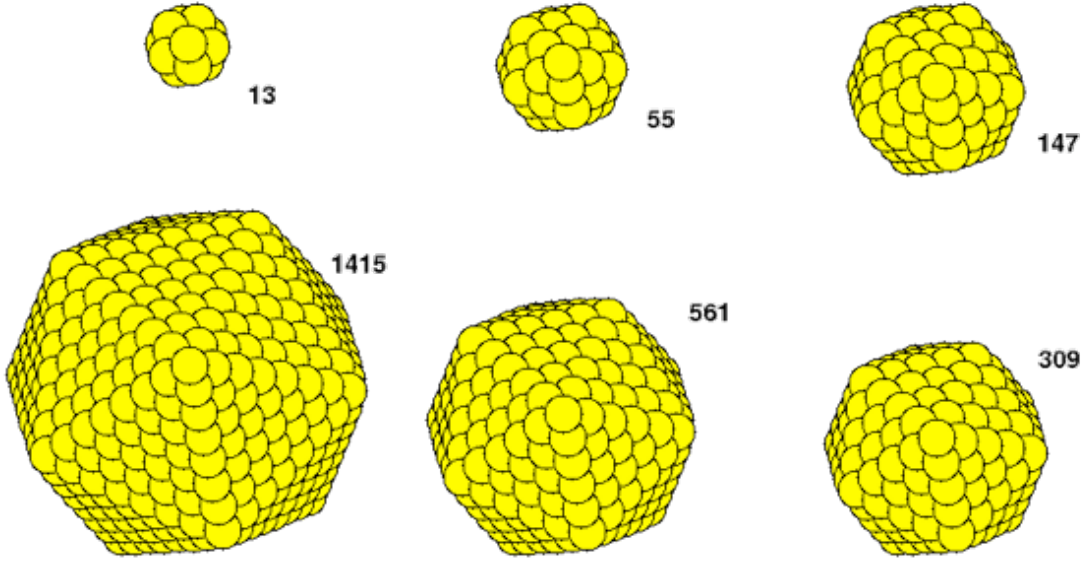
FIG. 5 Closed shell configurations of rare gas clusters form so called isocaheders and are particularly stable. They contain the number of atoms as indicated.
