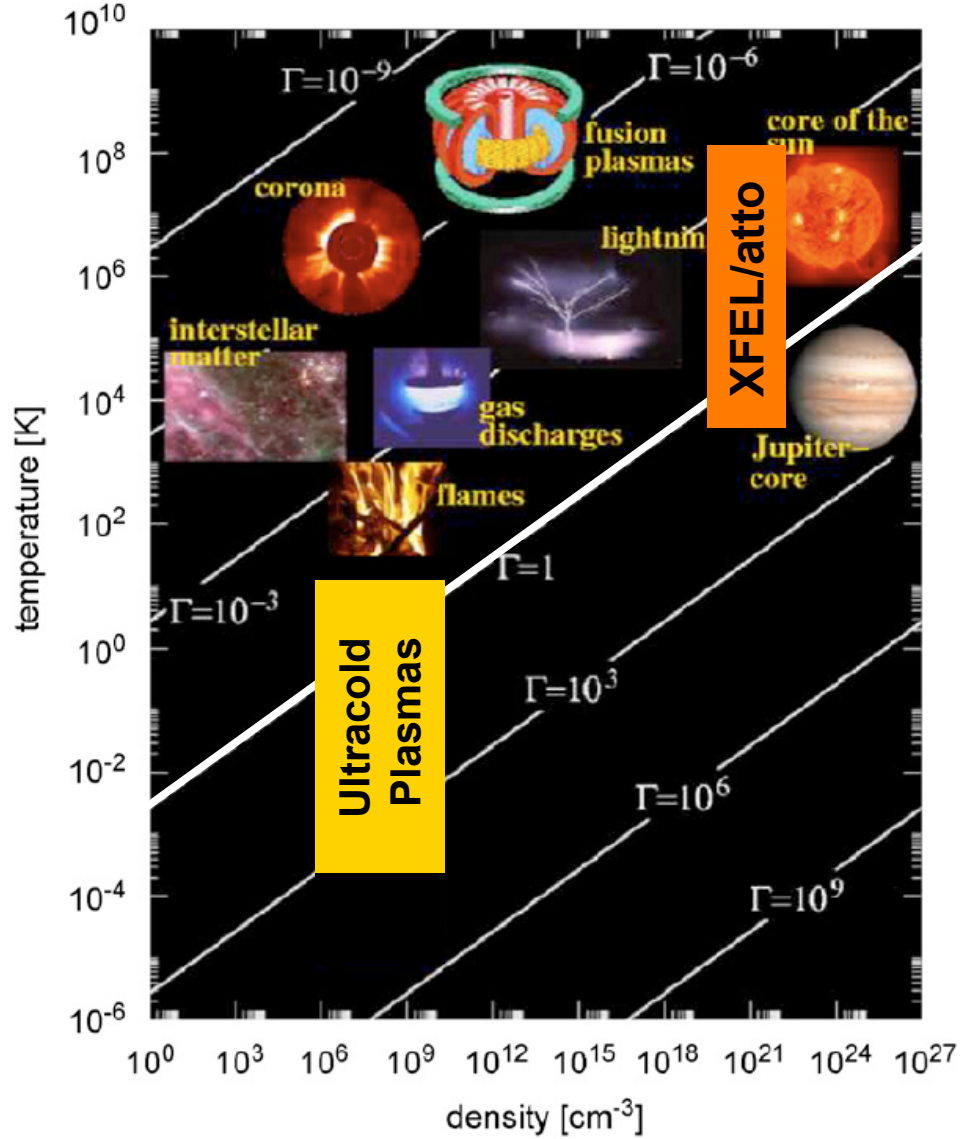
FIG. 1 Natural and man-made plasmas in the density- temperature plane, after (1). Lines of equal Coulomb coupling parameter \Gamma (see text) are given in white, the thick white line corresponds to \Gamma = 1 , the dividing line between ideal plasmas ( \Gamma \ll 1 ) and strongly coupled plasmas ( \Gamma \gg 1 ). Parameter ranges of the plasmas discussed here are indicated by the yellow and orange bars for ultracold and laser pulse generated plasmas, respectively.
