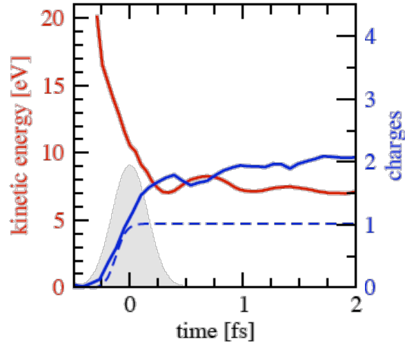
FIG. 7 Oscillation of the charges (black/blue, right axis) probed as in figure 6 with a pulse of variable time delay against the pump pulse (shown shaded, centered at time t = 0 ) which triggers the plasma dynamics in a cluster of 55 argon atoms, after (12). The probed charges indirectly map out the oscillation of the plasma electrons as is evident by the average kinetic energy of the plasma electrons (grey/red line, left axis), oscillating out of phase but with the same frequency. Also shown is the average charge state of the ions (dashed) which stays constant after the laser pulse is over. The two laser pulses have a photon energy of \hbar\omega = 20\text{eV} , peak intensity of 5 \times 10^{14}\text{W/cm}^2 and a duration of 250 attoseconds.
