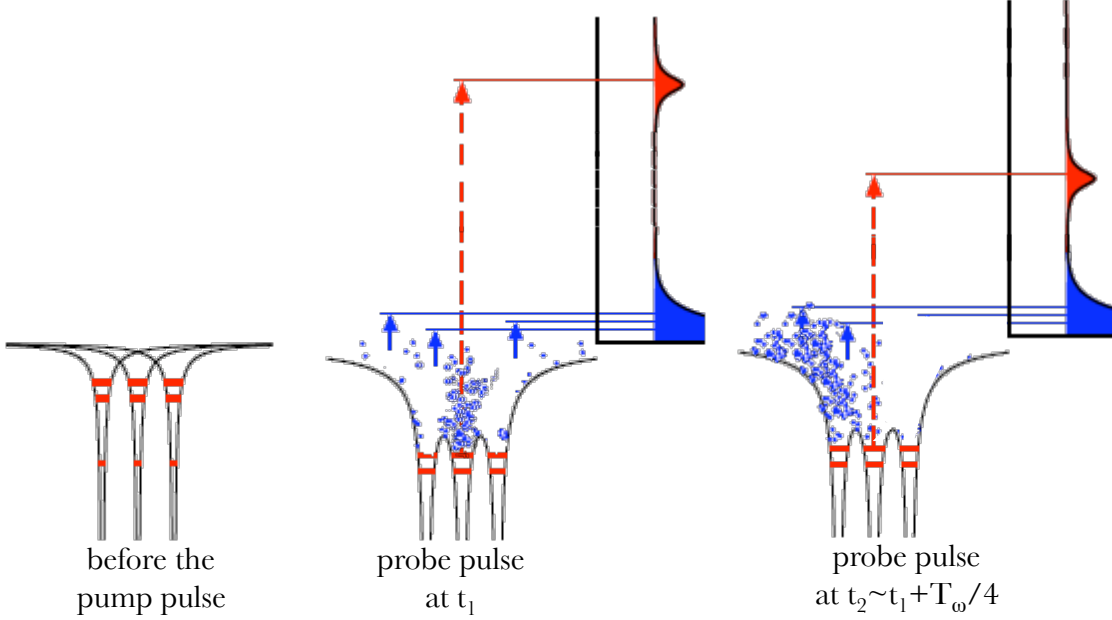
FIG. 6 Sketch of a double-pulse pump-probe measurement of electronic plasma dynamics, for details see text.
