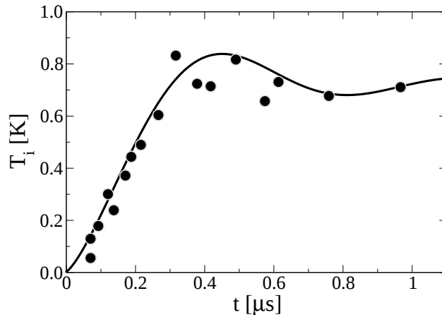
FIG. 8 Calculated (3) (line) and measured (13) (points) ion temperature of an expanding plasma of 1 million strontium ions with initial density \rho = 2 \times 10^9/\text{cm}^3 and initial electron temperature of T_e = 38 \text{ K} .
