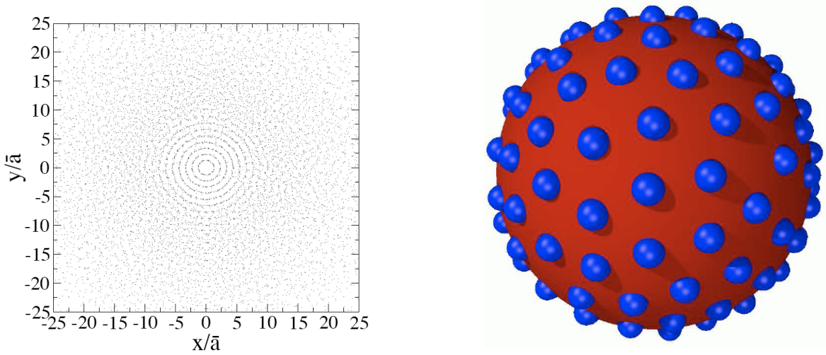
FIG. 4 Selforganization of a plasma of 80000 Beryllium ions after expansion time t = 216/\Omega into a crystal upon cooling with a rate of \beta = 0.2\Omega . The initial electronic Coulomb coupling parameter was \Gamma_e = 0.08 , after (10). Shown is on the left a cut through the center of the plasma, with the length scaled by the local mean distance a of ions. Distributions for several orientations have been superimposed for clarity of the structure. On the right the fourth shell of ions is shown (fourth circle from the center in the left figure).
