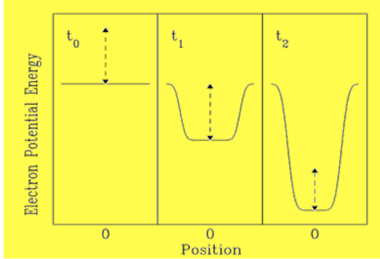
FIG. 2 Sketch of plasma formation by photo ionization of a geometrically confined gas, after (8). The left panels shows the neutral gas in the beginning at time t_0 . Electrons ionized acquire a kinetic energy E which is the difference between the photon energy \hbar\omega and the atomic binding energy I of the electron, E = \hbar\omega - I , indicated by the vertical dashed lines. The center panel captures the onset of plasma formation: due to multiple ionization a positive background potential of ions has formed which attracts the electrons. It is deep enough that the kinetic energy of a further electron ionized (indicated by an arrow) is not sufficient to escape from the cluster. Right panel: photo ionization of electrons into the plasma.
