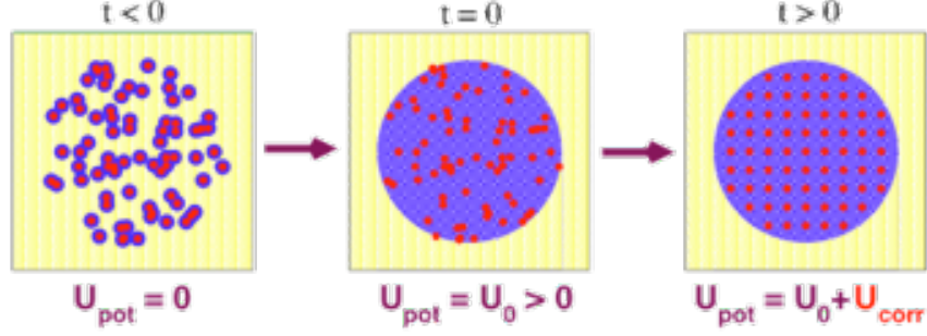
FIG. 3 A gas with randomly placed atoms (left panel, t < 0 ) is ionized at time t = 0 . As a consequence, there is potential energy E_{\text{pot}} = U_0 between the ions. Subsequently, correlations develop by which the potential energy is lowered, the generated positive correlation energy U_{\text{corr}} appears as kinetic energy (higher temperature) of the ions ( t > 0 ).
