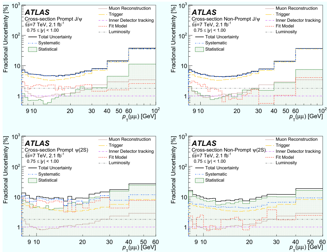
Fig. 5 Statistical and systematic contributions to the fractional uncertainty on the prompt (left column) and non-prompt (right column) J/\psi (top row) and \psi(2S) (bottom row) cross-sections for 7 TeV, shown for the region 0.75 < |y| < 1.00
