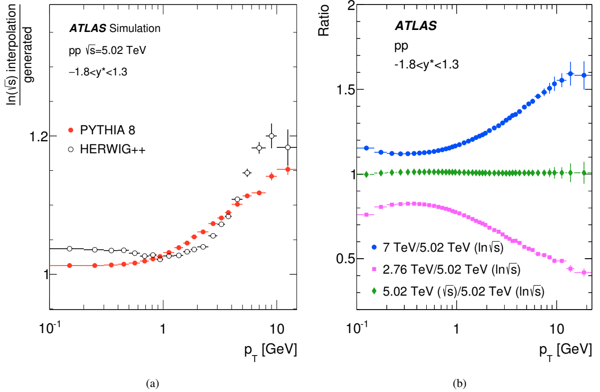
Figure 2: (a) The correction factors that are applied to the data. They are obtained as a ratio of the simulated differential cross section at \sqrt{s} = 5.02 TeV to the interpolated cross section, obtained from simulated samples at \sqrt{s} = 7 TeV and \sqrt{s} = 2.76 TeV with PYTHIA8 and Herwig++. (b) The ratios of the input invariant cross sections at \sqrt{s} = 7 TeV (blue circles) and at \sqrt{s} = 2.76 TeV (magenta squares) to the interpolated cross section at \sqrt{s_{NN}} = 5.02 TeV. The error bars represent the statistical uncertainties of the input spectra. The comparison between interpolation using \sqrt{s} and \ln(\sqrt{s}) is shown with green diamond markers. All the ratios are extracted within the maximal acceptance of the ID detector ( -1.8 < y^* < 1.3 ).
