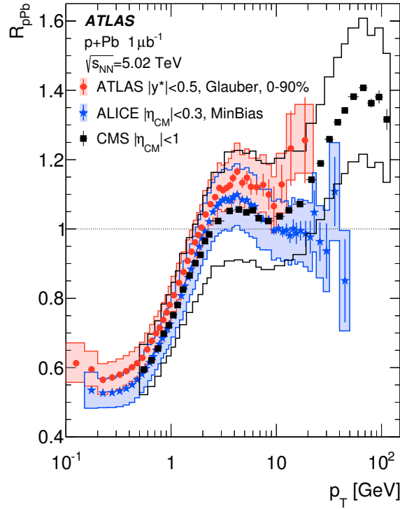
Figure 6: R_{pPb} values as a function of p_T in the 0–90% centrality interval averaged over |y^*| < 0.5 , are compared to the minimum-bias (0–100%) results from a different pseudorapidity range in the centre-of-mass system: ALICE for |\eta_{CM}| < 0.3 [26] and CMS for |\eta_{CM}| < 1 [29]. The \langle T_{Pb} \rangle value for the ATLAS centrality correction is calculated with the Glauber model. The total systematic uncertainties, which include the uncertainty in \langle T_{Pb} \rangle , are indicated by lines of the same colour. Strict quantitative agreement is not expected as each measurement uses different rapidity intervals for the centrality determination and apply different event selection criteria to reject diffractive collisions.
