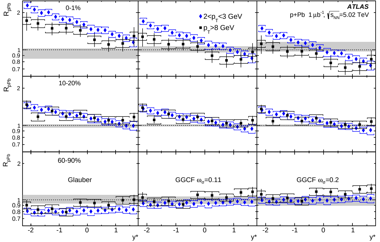
Figure 9: The R_{pPb} values for the 0–1% (top panels), 10–20% (middle panels) and 60–90% (lower panels) centrality intervals. The data points are shown for two different transverse momentum intervals indicated in the legends. The columns correspond to the Glauber model (left), Glauber-Gribov model with \omega_\sigma = 0.11 (middle), and Glauber-Gribov model with \omega_\sigma = 0.2 (right). The grey box in each panel reflects the systematic uncertainty associated with the centrality interval and with the model assumption. Statistical uncertainties are shown with vertical bars and systematic uncertainties with brackets.
