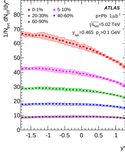
Figure 4: The invariant differential y^* spectra of charged particles produced in p +Pb collisions at \sqrt{s} = 5.02 TeV are shown in five centrality intervals for p_T > 0.1 GeV. The statistical uncertainties are indicated with vertical lines and the systematic uncertainties are indicated with boxes.
