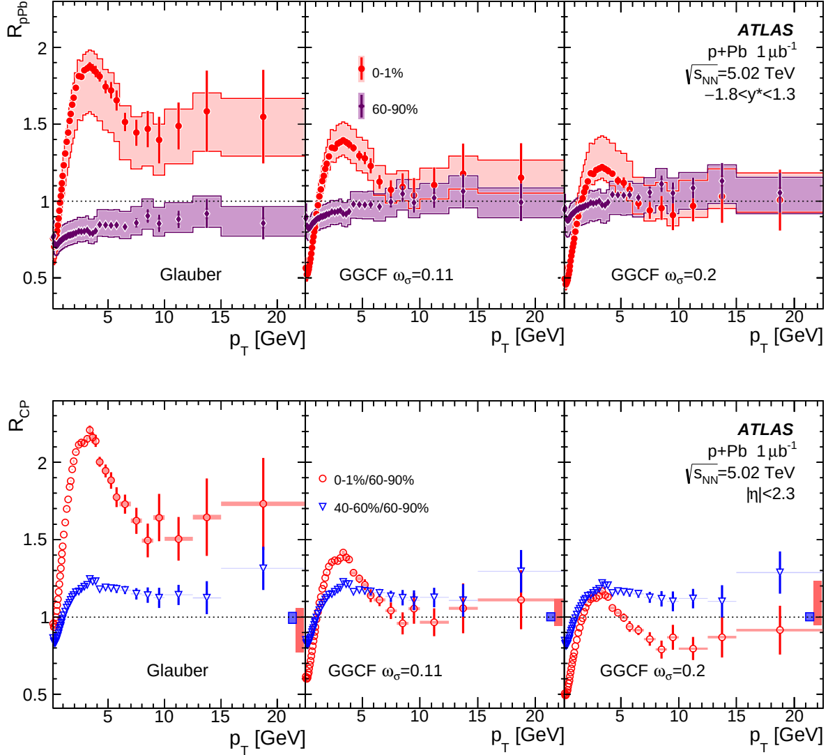
Figure 7: (top row) R_{pPb} as a function of p_T extracted from the invariant yields integrated over -1.8 < y^* < 1.3 for the 0–1% and 60–90% centrality intervals, and for different geometrical models used to calculate \langle T_{pB} \rangle : Glauber, Glauber-Gribov \omega_\sigma = 0.11 and Glauber-Gribov \omega_\sigma = 0.2 ; (bottom row) R_{CP} for 0–1% and 40–60% central collisions with respect to the 60–90% centrality interval, also for the geometrical models, which are used to calculate \langle T_{pB} \rangle . Statistical errors are indicated with vertical lines and the systematic uncertainties in the invariant yields are indicated by a shaded area. The total systematic uncertainty, which includes the uncertainty in \langle T_{pB} \rangle are indicated by lines of the same colour. The systematic uncertainty in the ratios of \langle T_{pB} \rangle are indicated by boxes of the same colour.
