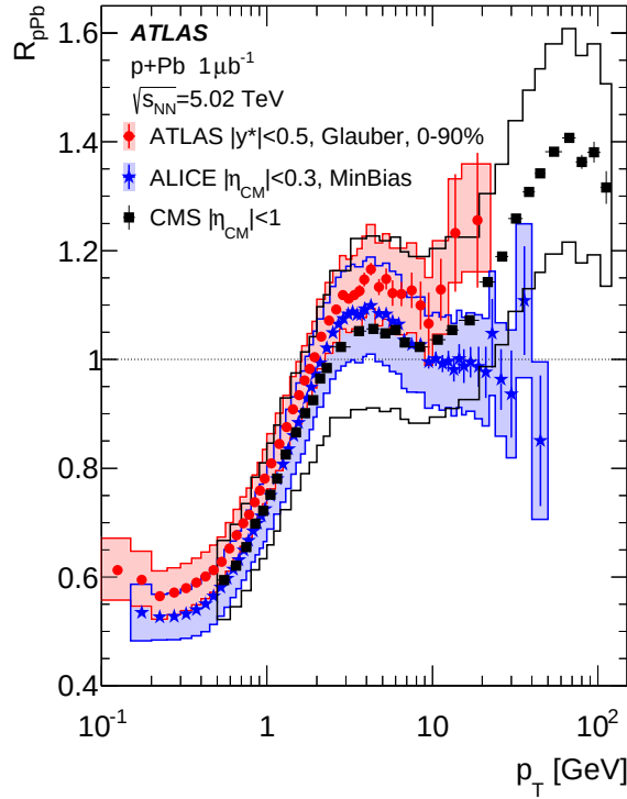
Figure 6: R_{p\text{Pb}} values as a function of p_{\text{T}} in the 0–90% centrality interval averaged over |y^*| < 0.5 , are compared to the minimum-bias (0–100%) results from a different pseudorapidity range in the centre-of-mass system: ALICE for |\eta_{\text{CM}}| < 0.3 [26] and CMS for |\eta_{\text{CM}}| < 1 [29]. The \langle T_{\text{pB}} \rangle value for the ATLAS centrality correction is calculated with the Glauber model. The total systematic uncertainties, which include the uncertainty in \langle T_{\text{pB}} \rangle , are indicated by lines of the same colour. Strict quantitative agreement is not expected as each measurement uses different rapidity intervals for the centrality determination and apply different event selection criteria to reject diffractive collisions.
