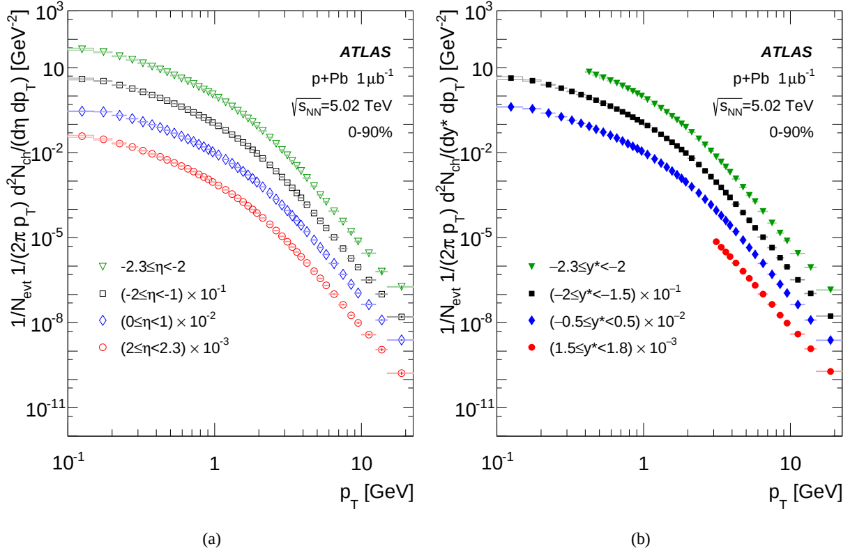
Figure 3: Invariant differential p_T spectra of charged particles which are produced in p +Pb collisions at \sqrt{s} = 5.02 TeV shown in (a) four \eta intervals and (b) four y^* intervals, for the 0–90% centrality interval. The individual spectra are scaled by constant factors (indicated in the legend) for visibility. The statistical uncertainties are indicated with vertical lines and the systematic uncertainties are indicated with boxes, but are generally much smaller than the size of the symbols.
