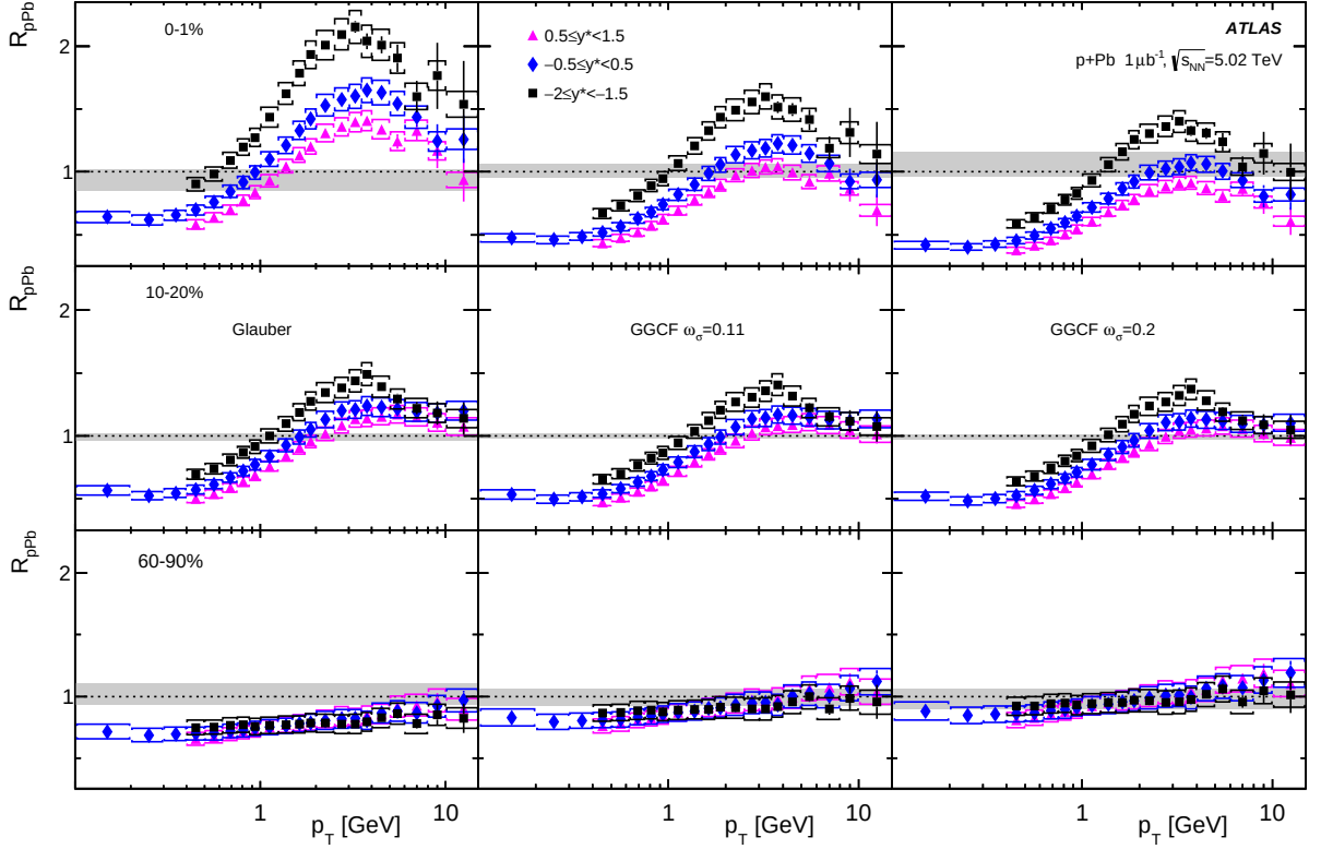
Figure 8: The R_{pPb} values for the 0–1% (top panels), 10–20% (middle panels) and 60–90% (lower panels) centrality intervals. The data points are shown for three different rapidity intervals indicated in the legends. The columns correspond to the Glauber model (left), Glauber-Gribov model with \omega_\sigma = 0.11 (middle), and Glauber-Gribov model with \omega_\sigma = 0.2 (right). The grey band in each panel reflects the systematic uncertainty associated with the centrality interval and with the model assumption. Statistical uncertainties are shown with vertical bars and systematic uncertainties with brackets.
