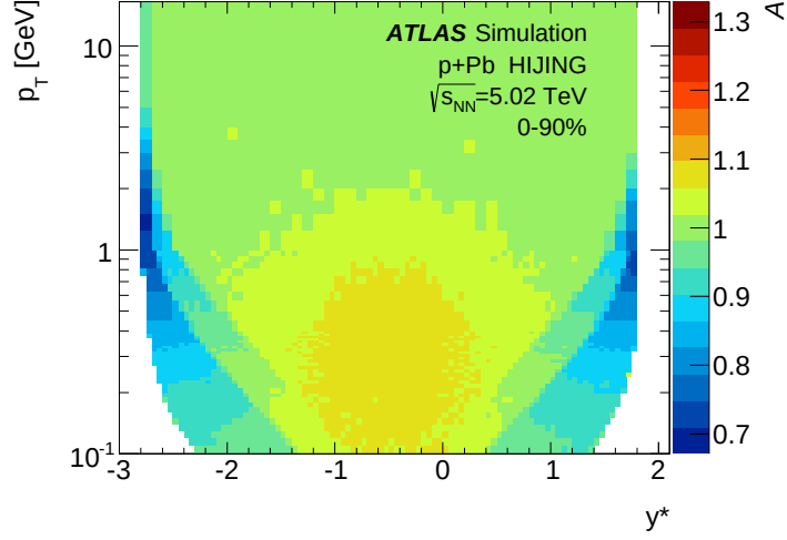
Figure 1: \mathcal{A}(p_T, y^*) as a function of p_T and y^* for the p +Pb MC sample.
