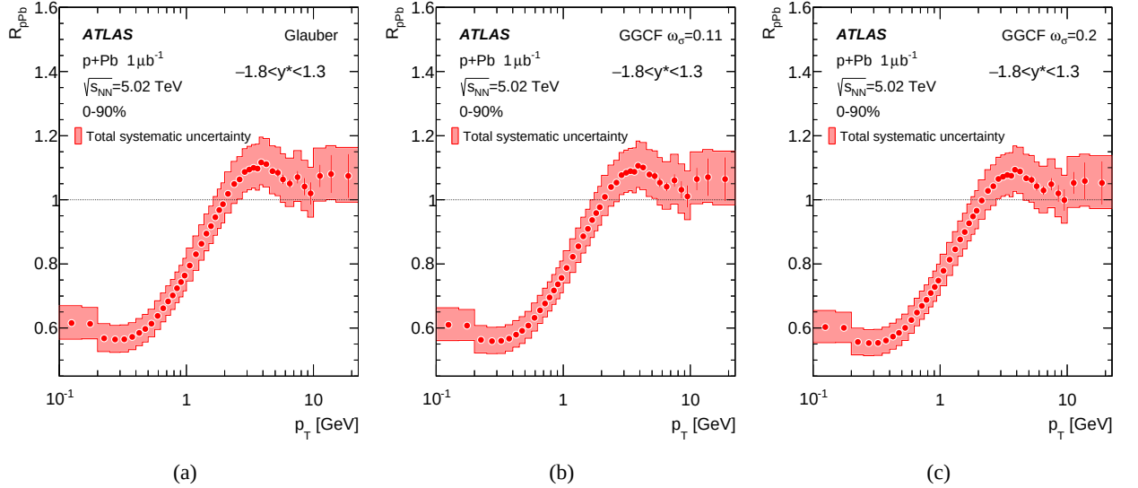
Figure 5: R_{pPb} as a function of p_T integrated over rapidity range -1.8 < y^* < 1.3 for the 0–90% centrality interval for the three geometric models: (a) Glauber, (b) Glauber-Gribov with \omega_\sigma = 0.11 and (c) Glauber-Gribov with \omega_\sigma = 0.2 .
