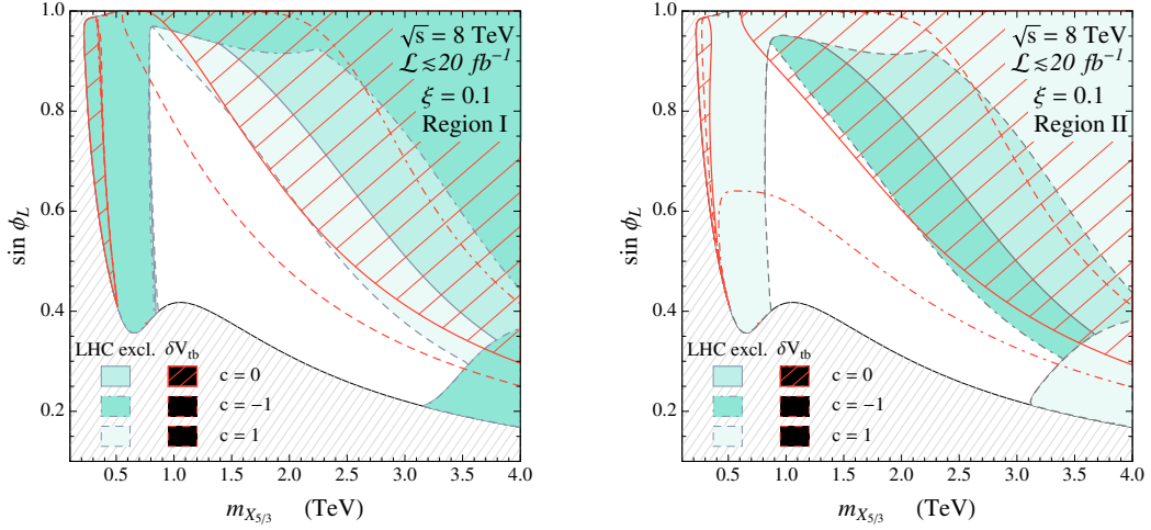
Figure 12. Exclusion bounds in the 2-site model with \xi = 0.1 coming from the 8 TeV LHC data for different values of c = 0, 1, -1 . The green regions show the bounds coming from the direct searches, while the red contours show the 95% CL constraints coming from the V_{tb} measurement.
