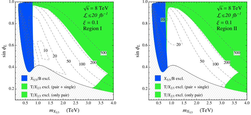
Figure 11. Exclusion bounds in the 2-site model with \xi = 0.1 and c = 0 for the 8 TeV LHC data. The left (right) panel corresponds to the Region I (Region II) of the parameter space. The blue and green region are excluded by the searches for the exotic X_{5/3} and the charge-2/3 resonances respectively. The darker green region shows the exclusions on the charge-2/3 states if only pair production is taken into account, while the estimates of additional constraints from single production are shown by the light green area. The dashed contours show the amount of tuning \Delta estimated by using eq. (4.5).
