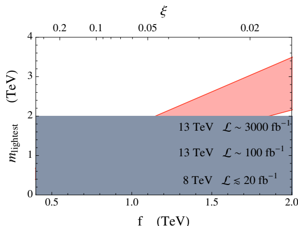
Figure 15. Maximal value of the mass of the lightest fermionic partner in the 5 + 5 2-site model as a function of f . The red band is obtained by assuming that the relation in eq. (4.4) is valid with 20% accuracy. The gray bands correspond to the present and expected universal bounds coming from pair production searches.
