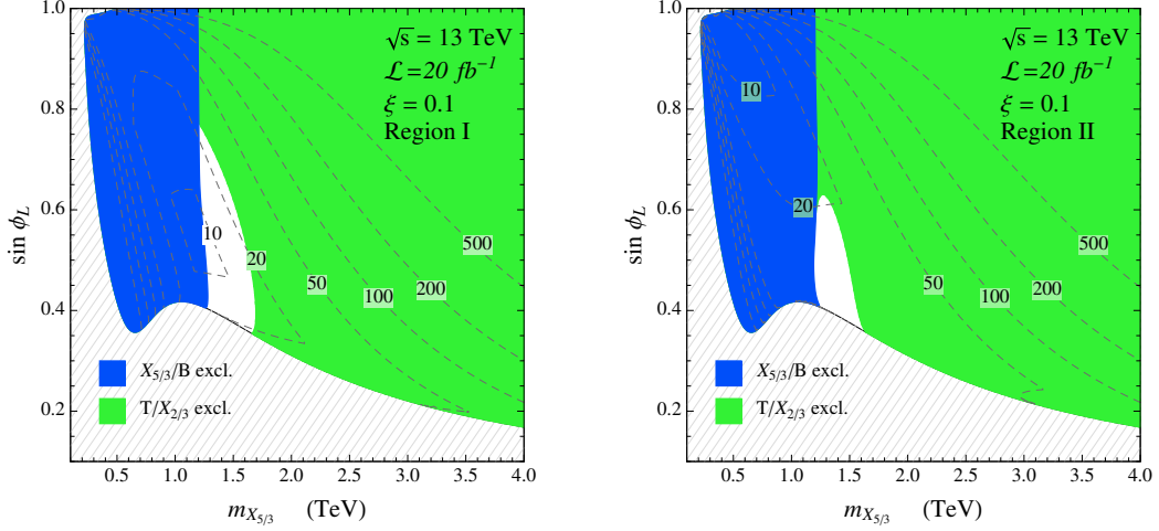
Figure 13. Expected exclusion bounds in the 2-site model with \xi = 0.1 and c = 0 for the 13 TeV LHC run with \mathcal{L} = 20 \text{ fb}^{-1} integrated luminosity. For further details see caption of figure 11.
