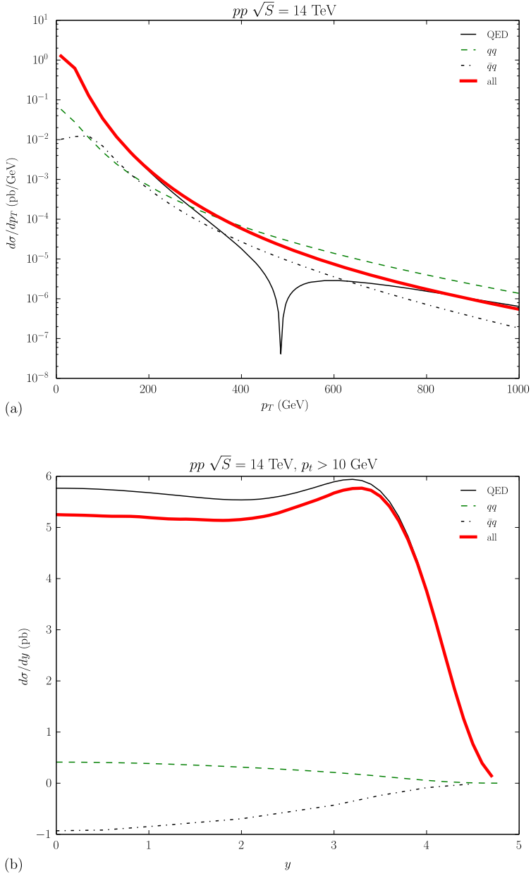
Fig. 11. Same as in Fig. 9, but for pp \rightarrow Z + X at \sqrt{S} = 14 TeV (LHC).
