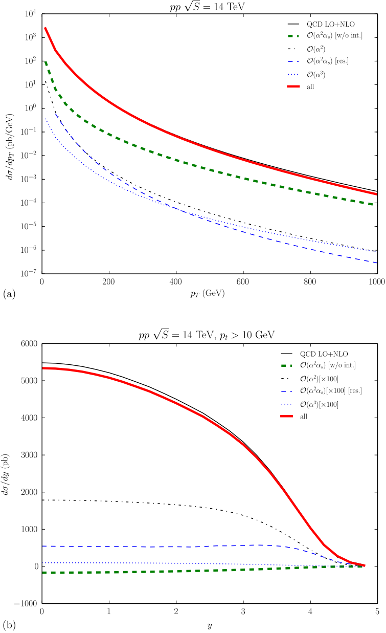
Fig. 10. Same as in Fig. 8, but for pp \rightarrow Z + X at \sqrt{S} = 14 TeV (LHC).
