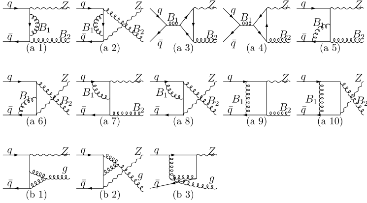
Fig. 2. QCD and QED one-loop diagrams contributing to the partonic subprocess q + \bar{q} \rightarrow Z + g at \mathcal{O}(\alpha\alpha_s^2) ( B_1 = B_2 = g ) and \mathcal{O}(\alpha^2\alpha_s) (diagrams (a 1)–(a 10) with B_1 = \gamma and B_2 = g ) and to the partonic subprocess q + \bar{q} \rightarrow Z + \gamma at \mathcal{O}(\alpha^2\alpha_s) (diagrams (a 1)–(a 10) with B_1 = g and B_2 = \gamma ). The QCD and QED one-loop diagrams contributing to the partonic subprocess q + g \rightarrow Z + q at \mathcal{O}(\alpha\alpha_s^2) and \mathcal{O}(\alpha^2\alpha_s) are obtained by appropriately crossing external legs.
