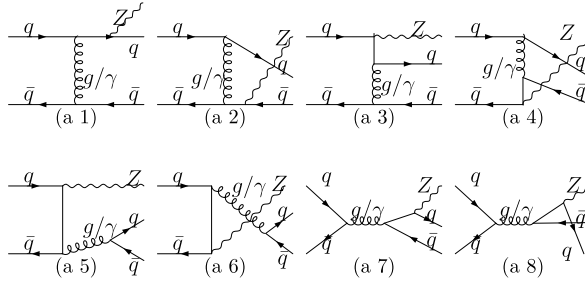
Fig. 4. Tree-level diagrams contributing to the partonic subprocess q + \bar{q} \rightarrow Z + q + \bar{q} at \mathcal{O}(\alpha_s^2) (with a virtual gluon). Interferences of diagrams (a 5)–(a 8) with a virtual photon or Z boson (gluon) with diagrams (a 1)–(a 4) with a virtual gluon (photon or Z boson) contribute at \mathcal{O}(\alpha^2\alpha_s) .
