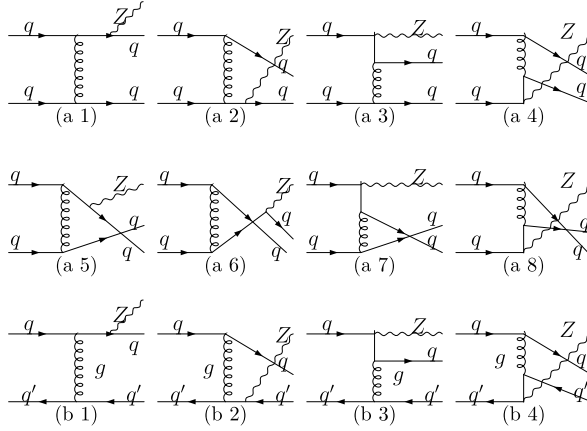
Fig. 6. Tree-level diagrams contributing to the partonic subprocesses q + q \rightarrow Z + q + q and q + q' \rightarrow Z + q + q' at \mathcal{O}(\alpha\alpha_s^2) . Interferences of diagrams (a 5)–(a 8) with the gluon replaced by a photon or Z boson with diagrams (a 1)–(a 4) contribute at \mathcal{O}(\alpha^2\alpha_s) .
