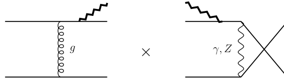
Fig. 7. \mathcal{O}(\alpha^{1/2}\alpha_s) and \mathcal{O}(\alpha^{3/2}) tree-level diagrams interfering to yield \mathcal{O}(\alpha^2\alpha_s) contributions to subprocesses q + \bar{q} \rightarrow Z + q + \bar{q} and q + q \rightarrow Z + q + q .
