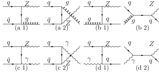
Fig. 1. Tree-level diagrams contributing to the partonic subprocesses q + \bar{q} \rightarrow Z + g and q + g \rightarrow Z + q at \mathcal{O}(\alpha_s) and to the partonic subprocesses q + \bar{q} \rightarrow Z + \gamma and q + \gamma \rightarrow Z + q at \mathcal{O}(\alpha^2) .
