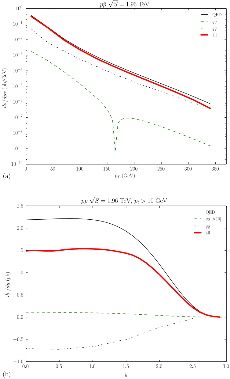
Fig. 9. The residual electroweak \mathcal{O}(\alpha^2\alpha_s) corrections in Fig. 8 (thick solid red lines) are decomposed into the combination of the \mathcal{O}(\alpha) QED corrections to subprocesses (10) and (12) (thin solid lines), and the \mathcal{O}(\alpha_s) QCD corrections to subprocess (11) (thin dot-dashed lines), and the QCD-electroweak interference contributions from subprocesses (14) (thin dashed green lines) and (18) (thin dashed green lines). (For interpretation of the references to color in this figure legend, the reader is referred to the web version of this article.)
