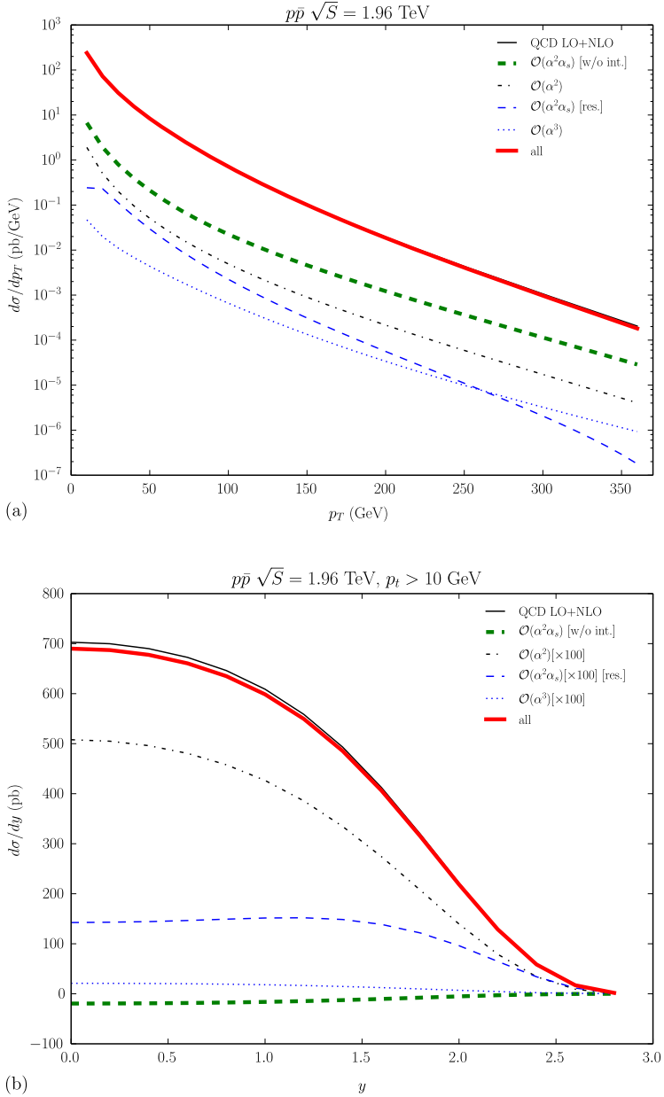
Fig. 8. Cross section distributions in (a) p_T and (b) y for p\bar{p} \rightarrow Z + X at \sqrt{S} = 1.96 TeV (Tevatron run II). In each frame, the NLO QCD result [12], i.e. the sum of the \mathcal{O}(\alpha\alpha_s) and \mathcal{O}(\alpha\alpha_s^2) results (thin solid lines), the \mathcal{O}(\alpha^2) Born result (thin dot-dashed lines), the purely weak \mathcal{O}(\alpha^2\alpha_s) corrections to subprocesses (10) and (12) [17] (thick dashed green lines), the residual electroweak \mathcal{O}(\alpha^2\alpha_s) corrections (thin dashed blue lines), the \mathcal{O}(\alpha^3) photoproduction contributions (thin dotted blue lines), and the total sum (thick solid red lines) are shown. (For interpretation of the references to color in this figure legend, the reader is referred to the web version of this article.)
