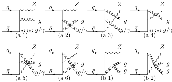
Fig. 5. Tree-level diagrams contributing to the partonic subprocess q + \bar{q} \rightarrow Z + g + g at \mathcal{O}(\alpha_s^2) and to the partonic subprocess q + \bar{q} \rightarrow Z + g + \gamma at \mathcal{O}(\alpha_s^2) .
