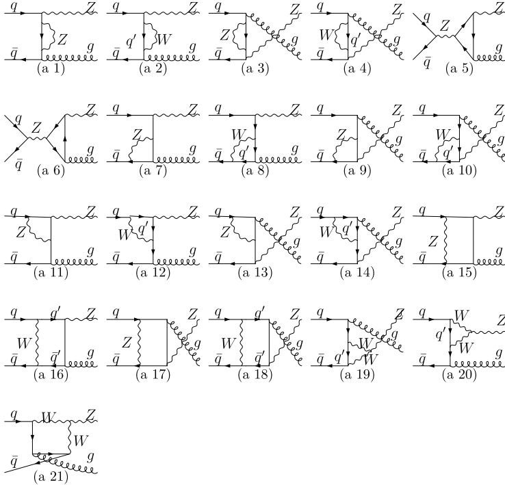
Fig. 3. Weak-interaction one-loop diagrams contributing to the partonic subprocess q + \bar{q} \rightarrow Z + g at \mathcal{O}(\alpha^2\alpha_s) . The weak-interaction one-loop diagrams contributing to the partonic subprocess q + g \rightarrow Z + q at \mathcal{O}(\alpha^2\alpha_s) are obtained by appropriately crossing external legs.
