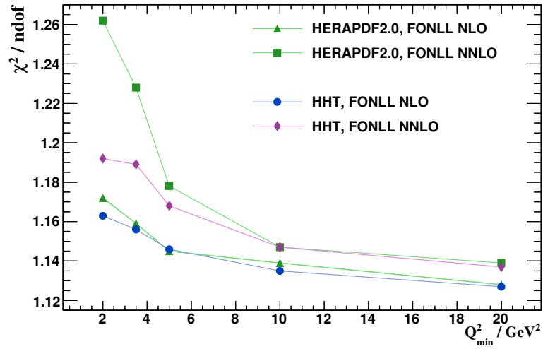
Figure 3: The \chi^2/\text{ndof} versus Q^2_{\min} for HHT and HERAPDF2.0 fits at NNLO and NLO using the FONLL heavy-flavour scheme instead of the default RTOPT scheme.
