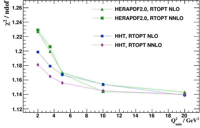
Figure 2: The \chi^2/\text{ndof} versus Q^2_{\min} for HHT and HERAPDF2.0 fits at NNLO and NLO.
