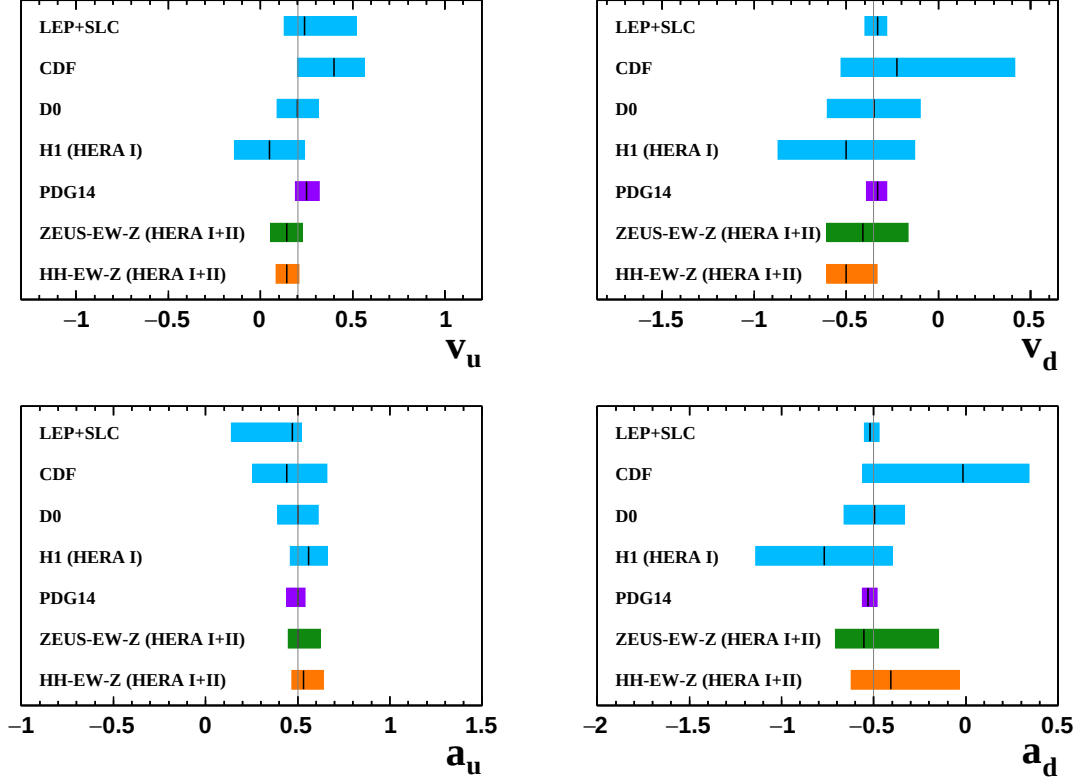
Figure 7: The values from the HH-EW-Z fit for a_d , a_u , v_d and v_u compared to the values from ZEUS-EW-Z and the results from LEP (ALEPH, OPAL, L3 and DELPHI) plus SLC (SLD) combined, the Tevatron (CDF and D0), HERA I (H1). The PDG14 world average is also shown; this does not contain the measurements from the HH-EW-Z and ZEUS-EW-Z fits based on all HERA data. All results are given with total uncertainties. Vertical black lines in each box indicate central values, the long gray vertical lines indicate the SM predictions.
