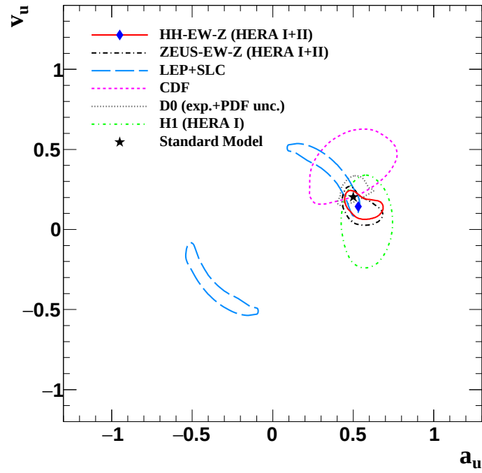
Figure 6: The 68 % C.L. contours for a_d , v_d and a_u , v_u obtained for the HH-EW-Z fit. Also shown are results from ZEUS-EW-Z, HERA I (H1), LEP (ALEPH, OPAL, L3 and DELPHI) plus SLC (SLD) combined, and the Tevatron (CDF and D0).
