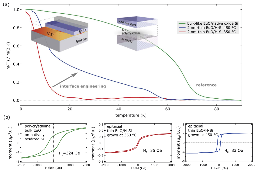
Figure 8. Ferromagnetic properties of ultrathin EuO on H-passivated Si (001) and of a bulk EuO reference grown on native \text{SiO}_2/\text{Si} . (a) Magnetization vs. T recorded at saturation field. Panel (b) shows hysteresis loops M(H) recorded at T = 2\text{ K} . The formula unit (f.u.) used for normalization is one \text{Eu}^{2+}\text{O}^{2-} in an fcc lattice with cubic parameter a = 5.14\text{ \AA} .
