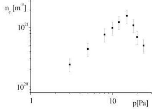
Figure 3: Time averaged electron density of the LF ICP.
