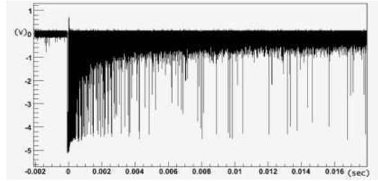
Figure 2: High energy muon event with long tail observed by CsI(Tl) detector. The time scale shown in the figure is up to 17ms and one can still see the photoelectrons.
