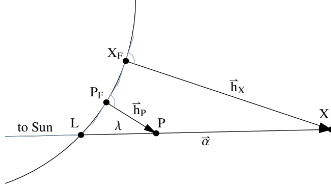
Figure 1: Geometry of the GECOSAX configuration drawn in the plane spanned by the center of the Earth, the center of the Sun and the satellite's position at t_0 . Figure taken from [4].
