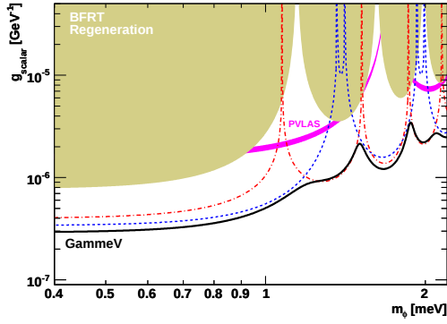
Figure 3: Exclusion region obtained by GammeV for the coupling to photons versus the mass of a scalar axion-like particle. The dashed lines show the limits obtained separately for the data recorded with the “wall” in the middle and near one end of the magnet. Also shown is the anomalous PVLAS region of interest. Finally, the shaded region indicates the previous exclusion from the BFRT.
