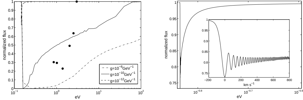
Figure 1: Left: Spectral oscillation feature as predicted for magnetars ( B = 10^{15} G and n(r_*) = 10^{15} \text{ cm}^{-3} (with the photospheric radius, r_* = 10 \text{ km} ) for several values of g . Note the prominent absorption-like feature which can be observed for g = 10^{-10} \text{ GeV}^{-1} which is the best current limit on g from CAST and horizontal branch stars. Also shown for comparison is (normalized) photometric data for a magnetar (circles; adopted from [8]). Right: Zoom in on the spectral oscillation feature for g = 10^{-12} \text{ GeV}^{-1} . The feature is broad and can be detected using low resolution spectra. The inset shows a high resolution blow up of the feature revealing oscillatory pattern being a trademark of photon-particle spectral conversion features.
