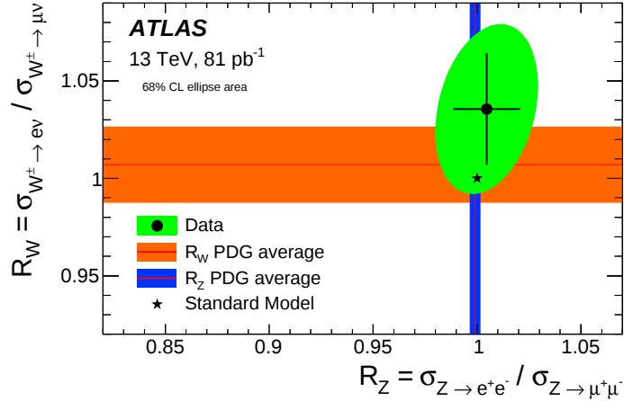
Figure 3: Ratio of the electron- and muon-channel W^\pm and Z -boson production fiducial cross sections, compared to the expected values of the Standard Model and previous experimental verifications of lepton universality for on-shell W^\pm and Z bosons, shown as PDG average bands [49, 50]. The PDG average values and the result are shown with total uncertainties.
