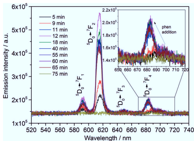
Fig. 5 In situ emission spectrum of [\text{Eu}(\text{phen})_2(\text{NO}_3)_3] ( \lambda_{\text{ex}} = 395 \text{ nm} ) measured with assembly 2. Inset: shift of {}^5\text{D}_0 \rightarrow {}^7\text{F}_4 \text{Eu}^{3+} transition upon addition of the phen solution.
