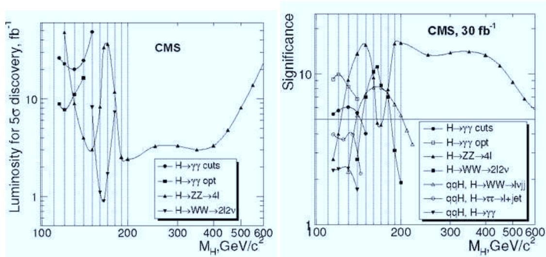
Fig. 3: Left: Integrated luminosity needed for 5\sigma discovery of the inclusive Higgs boson production pp \rightarrow H + X with the Higgs boson decay modes H \rightarrow \gamma\gamma , H \rightarrow ZZ^* \rightarrow 4l and H \rightarrow WW^* \rightarrow \ell\nu\ell\nu in the CMS experiment. Right: The signal significance as a function of the Higgs boson mass for 30 \text{ fb}^{-1} of the integrated luminosity for the different Higgs boson production and decay channels in the CMS experiment.
