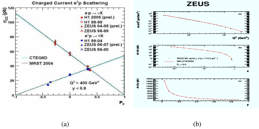
Fig. 1: (a) Cross section of CC e^\pm p DIS as a function of polarization from the ZEUS (triangles) and the H1 (circles) Collaborations. The results are consistent with SM predictions of \sigma_{CC}^{RH} = 0 (b). Single differential NC e^+p cross section as a function of Q^2 , Bjorken- x and y from the ZEUS Collaboration. The measured cross sections are consistent with SM predictions evaluated using the ZEUS-JETS PDF's.
